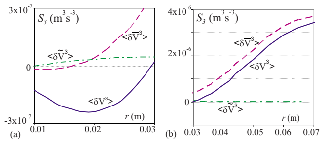
FIG. 10. (Color online) S_3 calculated using the full velocity \langle \delta V^3 \rangle , mean velocity \langle \delta \bar{V}^3 \rangle , and the fluctuation velocity \langle \delta \tilde{V}^3 \rangle at scales from (a) 0.01 m to 0.03 m and (b) from 0.03 m to 0.07 m.
