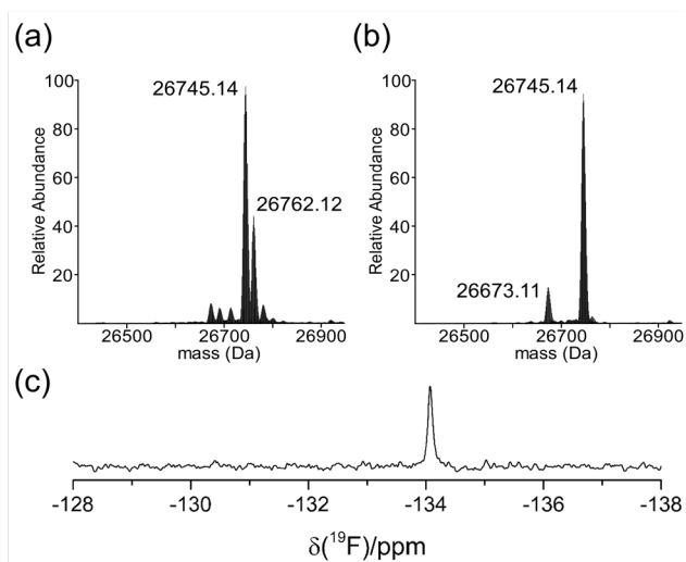
Figure 2. Protein production with single-site incorporation of 7FTrp. (a) Intact protein mass spectrum of RFP-13TAG expressed in a culture medium supplemented with 2 mM 7FTrp. The calculated mass for protein with a single 7FTrp residue in position 13 is 26,745.09 Da. The peak at 26762.12 Da corresponds to the additional installation of a 7FTrp residue in place of a natural tryptophan residue. (b) Intact protein mass spectrum of RFP13-TAG expressed in a culture medium supplied with 2 mM 7FTrp and 4 mM tryptophan. The mass of the minor peak at 26673.11 Da corresponds to amber stop codon suppression by glutamyl-tRNA. (c) 1D 19 F NMR spectrum of the RFP-13TAG sample in (b), demonstrating the incorporation of a single 7FTrp residue. The spectrum was recorded of a 0.2 mM protein solution in phosphate-buffered saline (PBS) at 25 °C on a 9.4 T NMR spectrometer.
