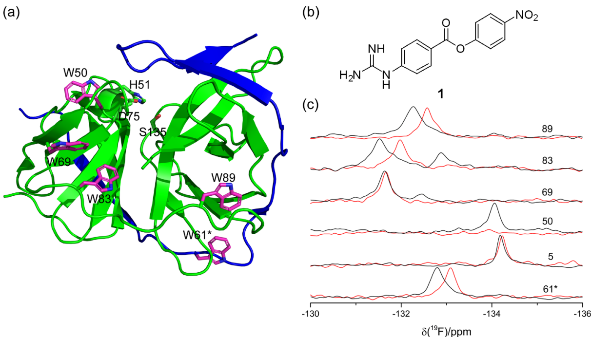
Figure 3. ZiPro with single-point mutations of tryptophan to 7FTrp. (a) Cartoon representation of the crystal structure of ZiPro (PDB ID: 5LC0). 31 NS3pro and NS2B are shown in green and blue, respectively. The side chains of the tryptophan residues are highlighted in magenta (the crystal structure did not report electron density for Trp5). Side chain atoms of the catalytic triad (Ser135, His51, and Asp75) are displayed as sticks. (b) Chemical structure of the broadband protease inhibitor 4-nitrophenyl-4-guanidinobenzoate. (c) 1D ^{19}\text{F} NMR spectra of the six ZiPro 7FTrp mutants recorded in the absence (black spectra) and presence of 20 equivalents of the inhibitor 1 (red spectra). The spectra were recorded of 0.3–0.7 mM protein solutions in NMR buffer (20 mM MES, pH 6.5, 150 mM NaCl) at 25 °C on a 9.4 T NMR spectrometer. The total recording time for each spectrum ranged between 5 and 25 minutes. The spectra are annotated with the sequence number of the respective mutation sites.
