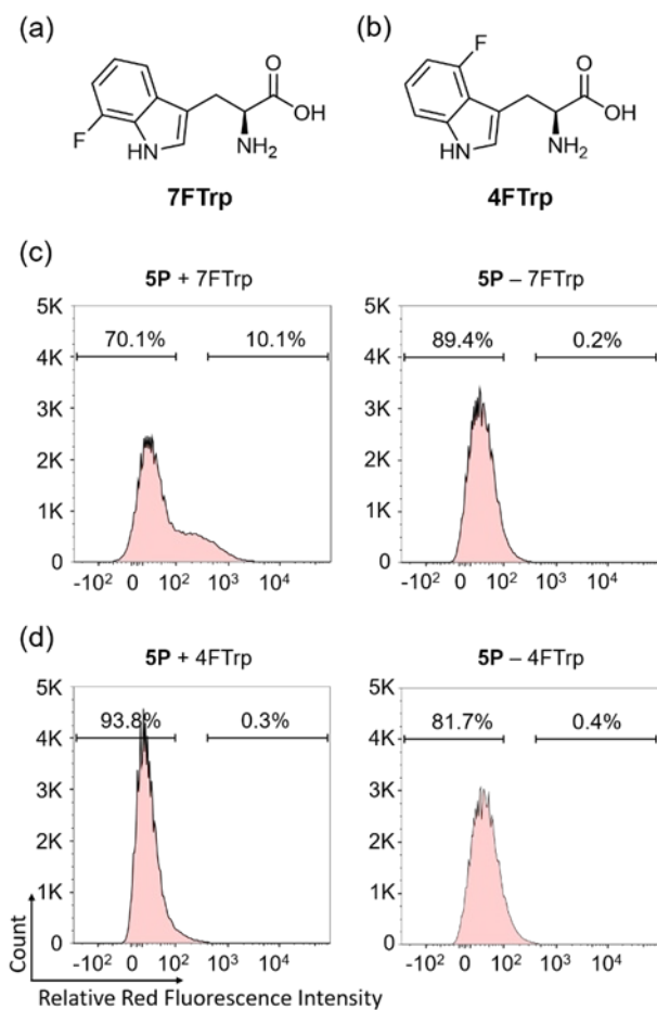
Figure 1. Chemical structures of (a) 7-fluoro-L-tryptophan (7FTrp) and (b) 4-fluoro-L-tryptophan (4FTrp). (c) Histogram of the fifth selection round to identify active G1PylRS enzymes for 7FTrp by FACS. P stands for positive selection rounds, where cells were cultured in the presence of FTrp. Identical cell cultures omitting FTrp (– FTrp) serve as controls. Cells were fluorescent when the gene of mCherry red fluorescent protein (RFP) containing an amber stop was expressed successfully. The difference in RFP fluorescence intensity of cells grown with or without FTrp serves as an indicator of the presence of FTrp-specific RS enzymes in the gene pool. (d) Same as (c), but for 4FTrp. Enrichment of active G1PylRS enzymes was observed only in the selection process targeting 7FTrp.
