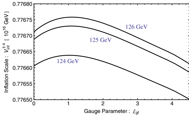
FIG. 2 (color online). The energy scale of inflation, V_{\text{inf}} , as the gauge parameter \xi_{\text{gf}} varies. We fix M_t = 170 GeV and show three values of M_H .
