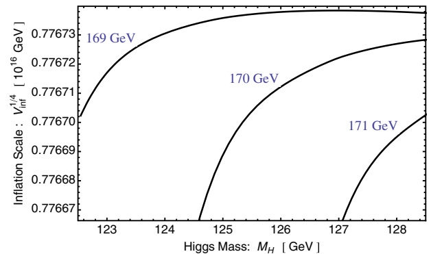
FIG. 1 (color online). The predicted energy scale of inflation, V_{\text{inf}}^{1/4} , over a range of Higgs boson masses ( M_H ), for three values of the top quark mass ( M_t ) and in the Landau gauge, \xi_{\text{gf}} = 0 .
