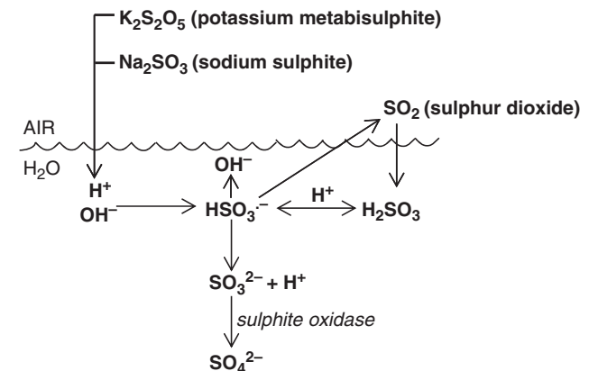
Fig. 1. Sulphite chemistry. Adapted from Stevenson and Simon [12].
