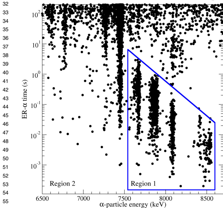
Fig. 2. A two-dimensional plot of the ER- \alpha correlation times on a logarithmic scale as a function of the \alpha -particle energies observed in the ^{34}\text{S} + ^{209}\text{Bi} reaction. The maximum searching time was 200 s.
