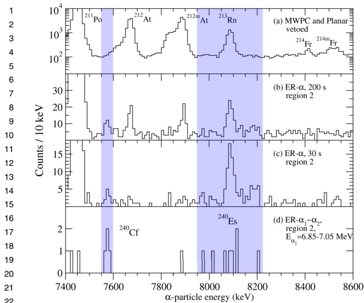
Fig. 1. Energy spectra of \alpha particles measured in the DSSDs and vetoed with the gas counter (MWPC) and the planar germanium detector from the ^{34}\text{S} + ^{209}\text{Bi} reaction: (a) all \alpha -like events; (b) \alpha -like events following a recoil implantation within 200 s; (c) \alpha -like events following a recoil implantation within 30 s; (d) as in (b) but followed by a second \alpha decay within 1200 s gated on the \alpha particle energy of ^{236}\text{Cm} . In panels (b), (c) and (d) the fast components identified as decays from transfer-reaction products shown in Fig. 2 (Region 1) have been excluded (see text for details). The \alpha -particle energy ranges assigned to ^{240}\text{Cf} and ^{240}\text{Es} are shaded in blue. (For interpretation of the references to colour in this figure legend, the reader is referred to the web version of this article.)
