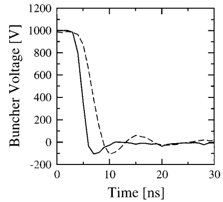
FIG. 3. Output waveform for the switching circuit, with no connected load (solid line), showing a measured fall time of 2.5 ns, and waveform when connected to the gating hardware (dashed line), showing a measured fall time of 3.2 ns. The slight ringing is of no consequence in our application, where the gate is effectively shut below 200 V.
