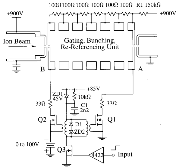
FIG. 1. Schematic diagram of the fast MOSFET switching circuit. This circuit includes the second MOSFET switch and bunching bias network required for driving the gating, bunching, and potential rereferencing unit described elsewhere (Ref. 3).
