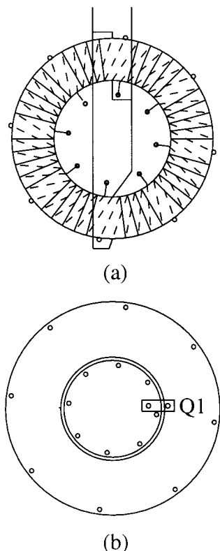
FIG. 2. Construction of (a) the pulse transformer, and (b) the associated printed circuit board, for the MOSFET drive circuit. This construction approach is required to minimize the MOSFET gate-drive inductance.
