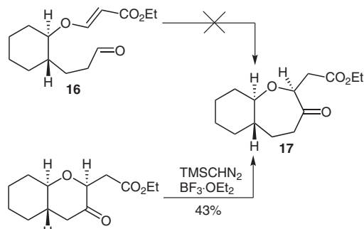
Scheme 4 Oxepanone synthesis
