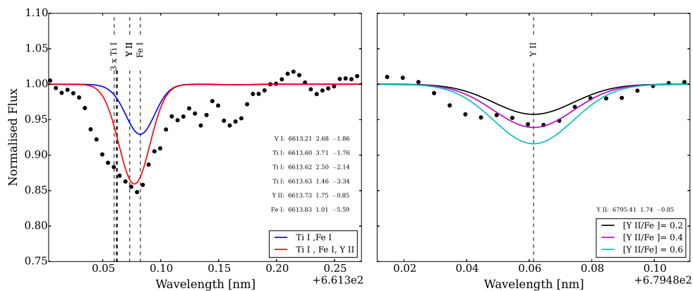
Figure 1. The blended Y \text{ II} feature, which is very similar for all stars, is shown for star B-128. The panel at left shows the synthesis of this line with the contribution of \text{Ti I} and \text{Fe I} in blue and the contribution of \text{Ti I} , \text{Fe I} and Y \text{ II} in red, for the Y value measured for this star shown at right, of [\text{Y}/\text{Fe}] = 0.4 dex (and [\text{Ti}/\text{Fe}] = 0.25 as measured from the \text{Ti} lines in the spectra). The panel at right shows the best-fitting abundance of [\text{Y}/\text{Fe}] = 0.4 dex and syntheses at \pm 0.2 dex comparison, for the unblended feature at 679.4 nm which we use to derive all of our [\text{Y}/\text{Fe}] abundances. The parameters of the absorption features are provided in the figures, to indicate the relative line strengths, in order of element, wavelength, excitation potential and log g_f .
