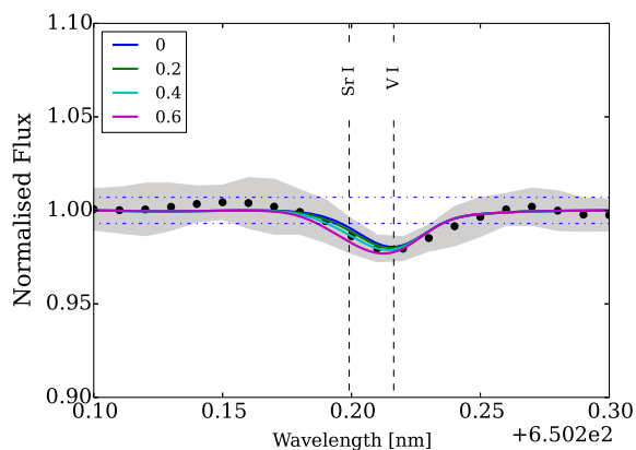
Figure 2. The median spectra from all eight stars combined for the \text{Sr} feature at 650.4 nm. The synthesis shows the line profiles for abundance ratios of [\text{Sr}/\text{Fe}] = 0, 0.2, 0.4, 0.6 for the typical [\text{V}/\text{Fe}] ratio of [\text{V}/\text{Fe}] \approx 0 for the stars. The solid grey lines represent the 1\sigma measurement of the mean of the eight stars and the dashed lines either side of the line profile show the width of the noise of the combined spectra. The best fit to the line adopting [\text{V}/\text{Fe}] = 0 is [\text{Sr}/\text{Fe}] = 0.40 .
