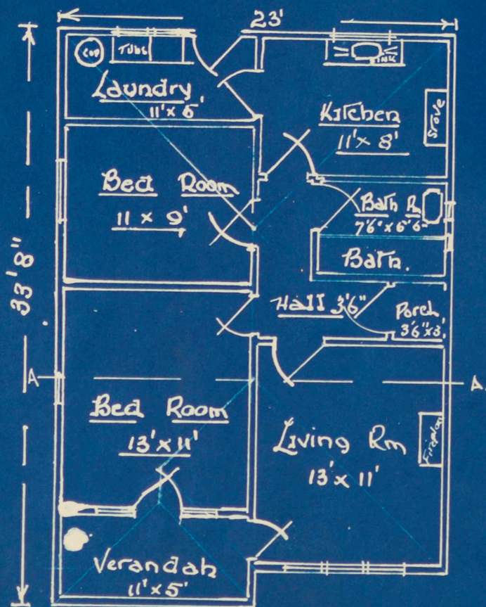
Plan Scale 1/8" = 1ft.
