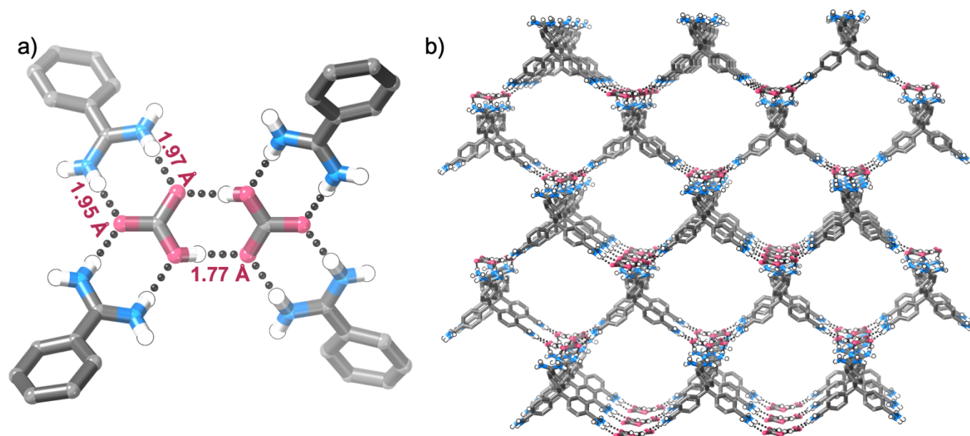
Fig. 2 Views of structure of AEHB framework \mathbf{1}\cdot(\text{HCO}_3)_4 : a) view of hydrogen bonding interactions showing unique \text{H}\cdots\text{O} distances (a fourfold screw axis is present located between the two \text{HCO}_3^- anions); b) view of one of the diamondoid nets. C–H hydrogen atoms, water molecules, and bicarbonate dimers in pores are omitted for clarity.
