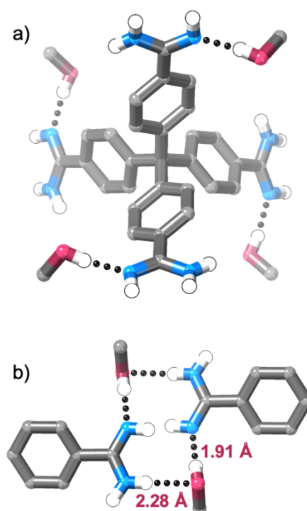
Fig. 3 Views of structure of 2 ·(CH 3 OH) 4 : a) view of one molecule; b) view of the intramolecular H-bonding showing crystallographically unique H···O and H···N distances. C–H hydrogen atoms are omitted for clarity.
