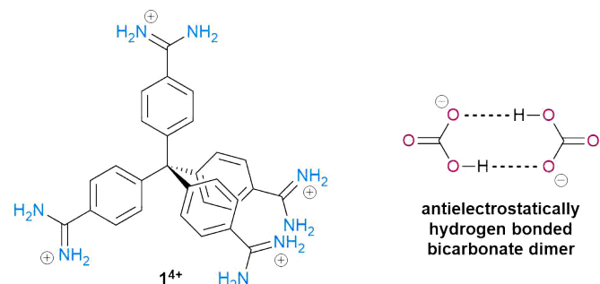
Fig. 1 Structure of tetraamidinium building block 1 4+ and AEHB bicarbonate dimer.
