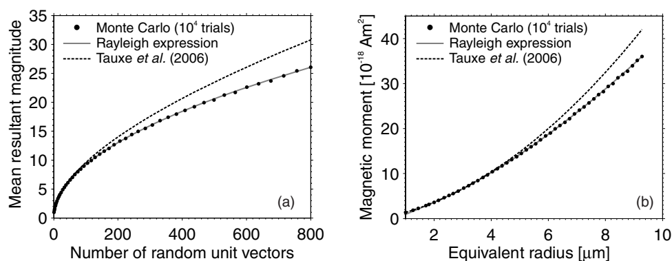
Figure 2. (a) The mean resultant magnitude of a given number of random unit vectors drawn uniformly from the surface of a sphere. The mean result from 10^4 Monte Carlo trials (black points) is consistent with the asymptotic Rayleigh expression (grey line). The Monte Carlo model of Tauxe et al. (2006) clearly overestimates the resultant magnitude for larger systems. (b) when converted to a floc model based on a fundamental floc size of 1 \mu\text{m} and a magnetization of 0.33 \text{ Am}^{-1} it can be seen that the polynomial approximation employed in earlier models (dashed line) is in error for higher equivalent radii.
