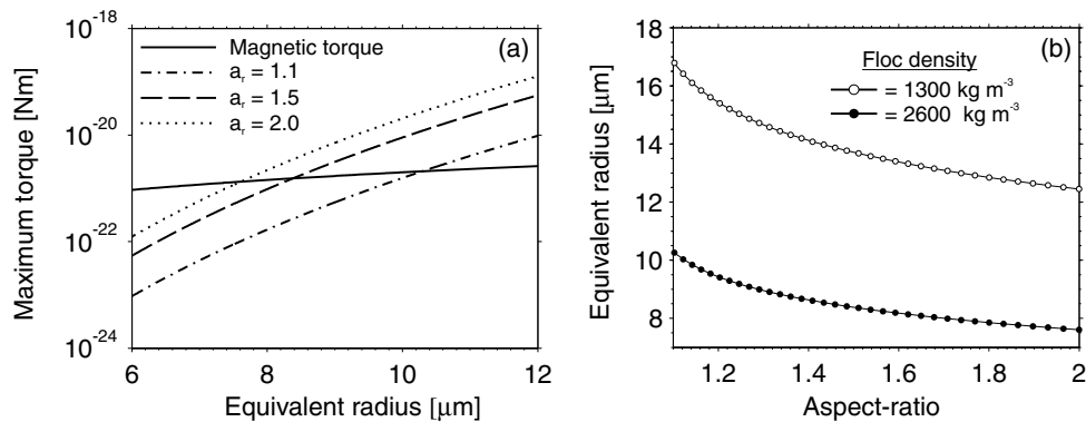
Figure 4. (a) A comparison of the maximum magnetic and hydrodynamic torques as a function of equivalent radius for prolate ellipsoids with aspect ratios of 1.1, 1.5 and 2.0 and a density of 2600 \text{ kg m}^{-3} . (b) The equivalent radius at which the maximum magnetic and hydrodynamic torques are equal for a prolate ellipsoid with a given aspect ratio. As the density of the floc decreases the equivalent radius at which the torques balance increases.
