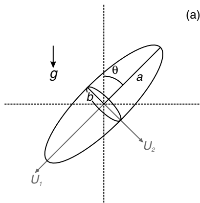
Figure 3. (a) The size and shape of the prolate ellipsoids employed in this study are described by their large and small radii, a and b , respectively. The orientation of the long axis of the ellipsoid to the vertical is given by the angle \theta and g represents the direction in which gravity is acting. The components of the ellipsoid's velocity parallel and perpendicular to its long axis are given by U_1 and U_2 , respectively. (b) The geometric factor, G , for a prolate ellipsoid versus eccentricity, e .
