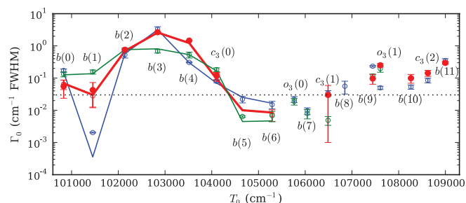
FIG. 6. Experimental natural linewidths, \Gamma_0 , extrapolated to J' = 0 of excited ^1\Pi_u -states of ^{14}\text{N}_2 , ^{14}\text{N}^{15}\text{N} , and ^{15}\text{N}_2 (blue, red, and green lines and points; respectively); plotted versus their ^{14}\text{N}^{15}\text{N} term-origins, T_0 . Experimentally determined natural linewidths are from the present and previous observations (filled and empty circles, respectively), and CSE-calculated predissociation linewidths (which exclude radiative broadening) are connected by lines. The locations of o_3(1) and b(9) have been shifted from their true T_0 for clarity and a horizontal line has been superimposed indicating the minimum width detectable in the present ^{14}\text{N}^{15}\text{N} spectrum. References to previous measurements of ^{14}\text{N}^{15}\text{N} linewidths are given in Table II, values for ^{14}\text{N}_2 and ^{15}\text{N}_2 are collected from a variety of sources. 14, 18, 23, 25, 26, 31, 32, 46, 60
