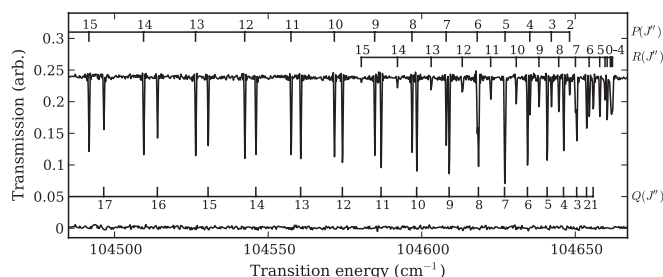
FIG. 2. The recorded transmission spectrum of b\ ^1\Pi_u(v=5) \leftarrow X(0) (upper trace) and the residual error of a model spectrum following the fitting of lineshapes (lower trace).
