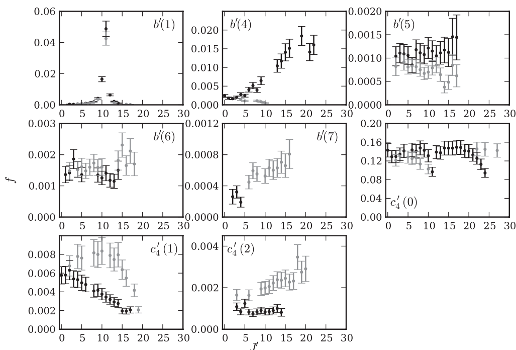
FIG. 8. Rotational dependence of ^1\Sigma_u^+ - X experimental ^{14}\text{N}^{15}\text{N} f -values labelled according to their excited vibrational level. Values are shown for P - and R -branch transitions (dark and light points, respectively).
