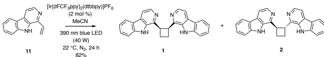
Scheme 2: The [2+2]-photodimerization of alkene 11 leading to compounds 1 and 2 .
