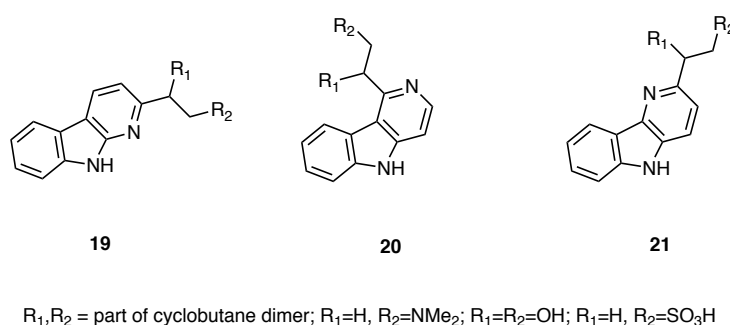
Figure 2: Possible alternative structures, 19-20 , considered for orthoscuticellines A-E
