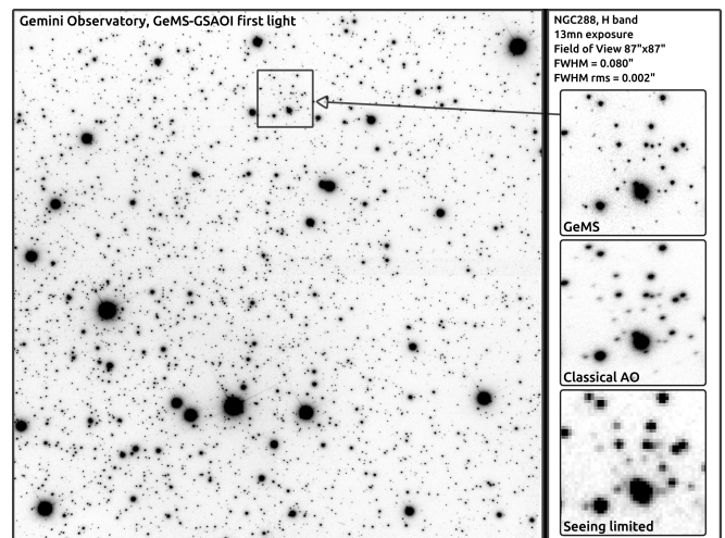
FIG. 4.— First light image of GeMS, the Gemini MCAO system, providing close to the diffraction-limited resolution images over 2 arcminute square, an order of magnitude larger – in surface – than the isoplanatic patch at 2.2 microns.
