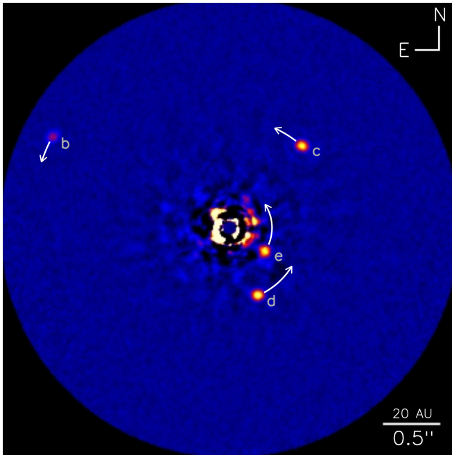
FIG. 3.— The detection and direct imaging of a planetary system around main sequence star HR8799 (Marois et al. 2010). In 2013, out of the six planetary systems directly imaged (excluding distant planets), five had been with Adaptive Optics system and one from HST (Marchis private communication).
