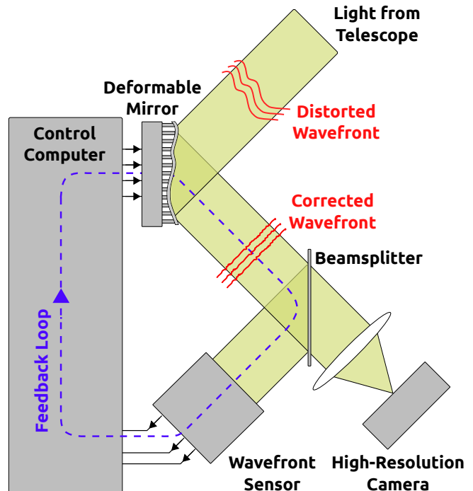
FIG. 1.— Principle of AO in a close loop arrangement.
