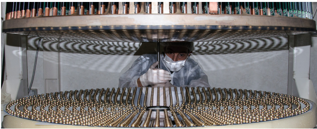
FIG. 2.— Deformable secondary mirror being assembled, showing the shell and magnets (bottom) and reference surface, coils and electronic (top). Credit AdOptica.
