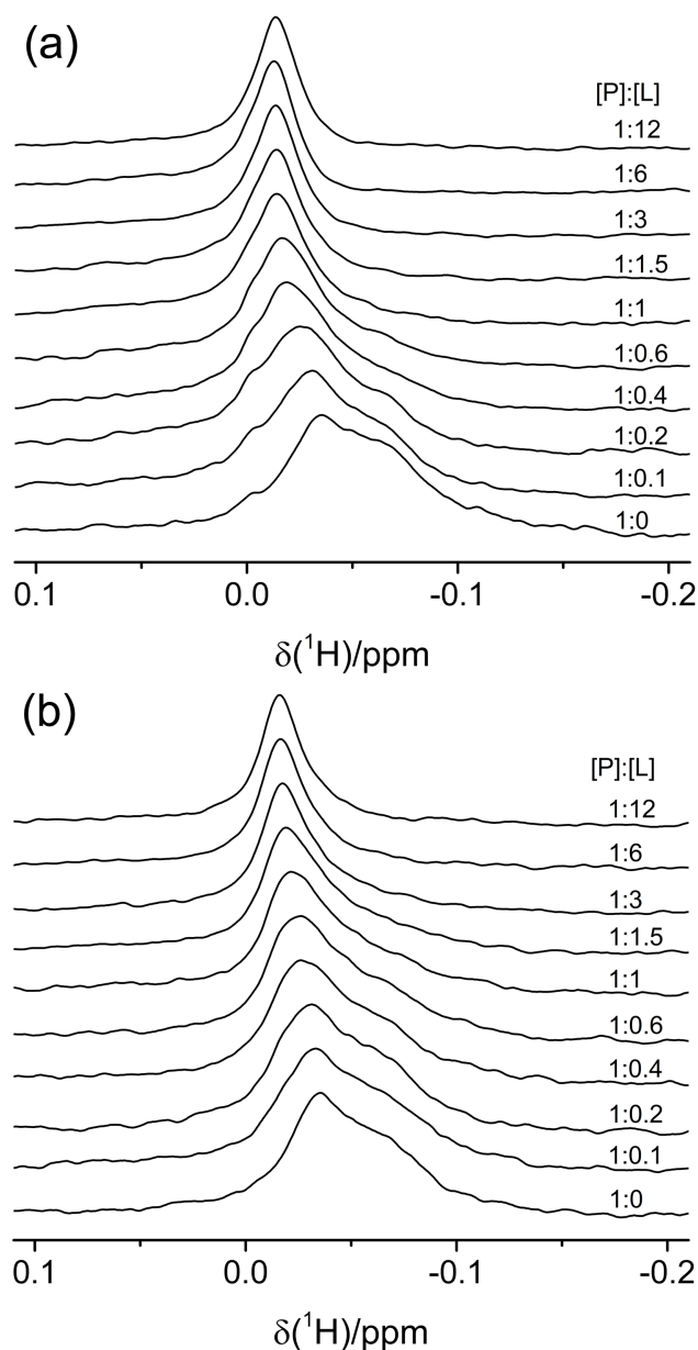
Figure 6. Titration of CNRS N117TMSK in NMR buffer with (a) CNF and (b) AcF. The spectra were recorded at 25 °C on a 800 MHz NMR spectrometer in about 4 minutes each. The protein concentration [P] was 100 \mu\text{M} and the ligand concentration [L] was as indicated.
