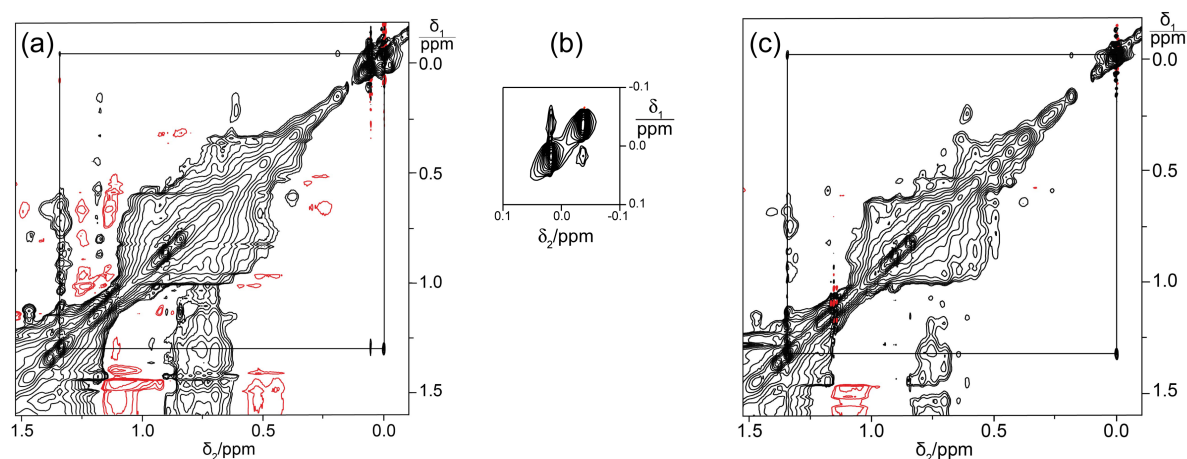
Figure 12. NOEs and exchange cross-peaks of the TMS resonance in a 0.6 mM solution of AncCDT-1 P57TMSK/N151Tby in 50 mM HEPES, pH 7.5, 150 mM NaCl at 25 °C. Jump-return delay 88 \mu\text{s} , 200 ms mixing time, t_{1\text{max}} = 25 ms, t_{2\text{max}} = 0.56 s, 600 MHz NMR spectrometer, total recording time 17 h. (a) 2D NOESY spectrum of the protein after denaturation and refolding. Vertical and horizontal lines drawn from the diagonal peaks of the tert -butyl and TMS groups meet at the cross-peaks between these two groups. (b) Spectral region of the TMS signals plotted at higher contour levels to highlight the exchange cross-peaks. (c) Same as (a) but after addition of an equimolar amount of arginine.
