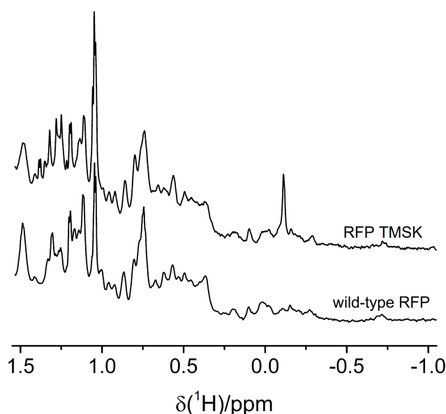
Figure 10. High-field spectral region of the 1D 1 H NMR spectra of wild-type RFP and RFP with a TMSK residue incorporated following the initiating methionine residue. The spectra were recorded in 25 mM Tris-HCl, pH 7.5, 150 mM NaCl at 25 °C using a 800 MHz NMR spectrometer. Protein concentrations were about 50 μM. The total recording time per spectrum was about 4 minutes.
