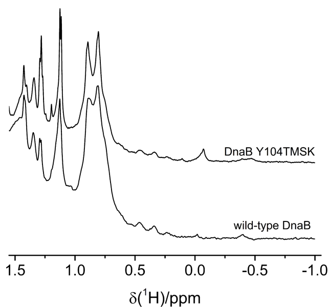
Figure 3. 1D ^1\text{H} NMR spectra of a 100 \mu\text{M} solution of Bst DnaB and 25 \mu\text{M} solution of its mutant Y104TMSK. The spectra were recorded in 25 mM Tris-HCl, pH 7.5, 150 mM NaCl, at 25 ^\circ\text{C} using a Bruker 600 MHz NMR spectrometer. The total recording time per spectrum was 4 and 30 minutes, respectively.
