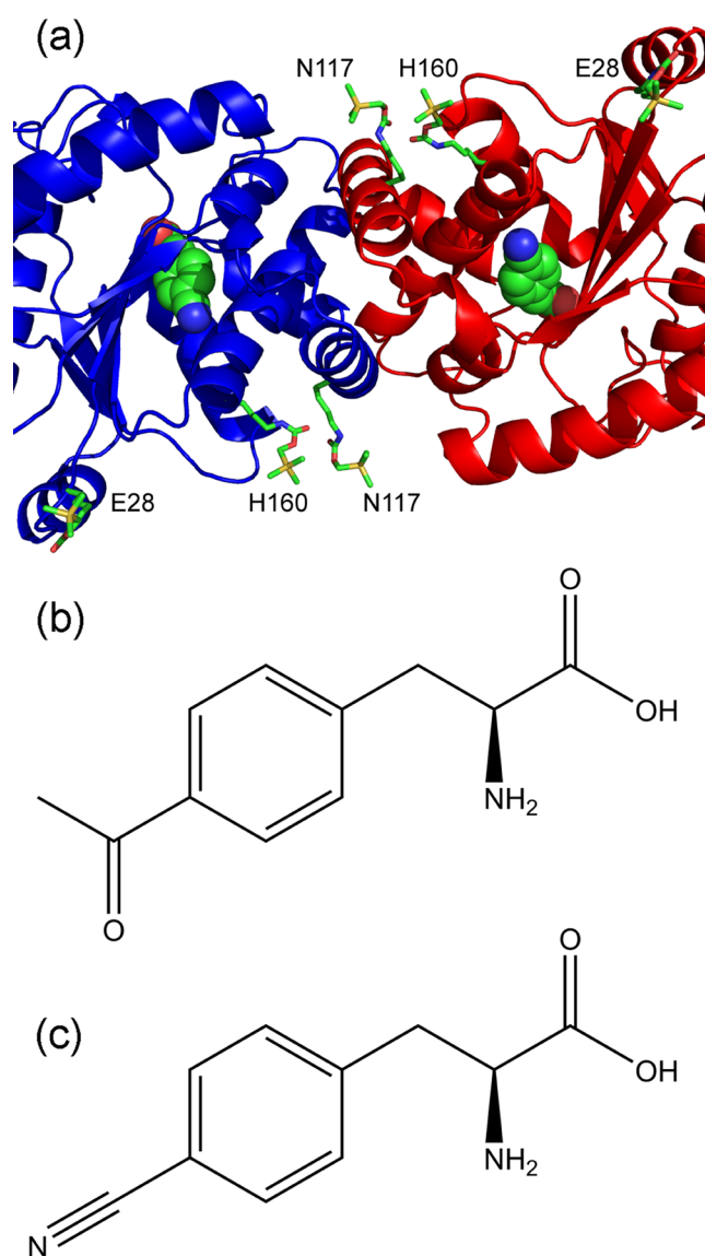
Figure 4. Homodimer interface of CNRS with locations of mutation sites and chemical structures of amino acid ligands. (a) Ribbon representation of the homodimer interface of CNRS (PDB: 3QE4) 16 showing the monomeric subunits in blue and red, respectively. TMSK residues modeled at the positions indicated are shown in stick representations. CNF in the active sites is highlighted by spheres. (b) Chemical structures of p -acetyl- L -phenylalanine (AcF) and (c) p -cyano- L -phenylalanine (CNF).
