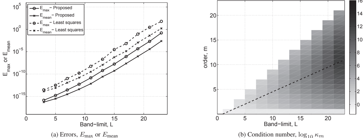
Fig. 2: (a) The reconstruction errors, E_{\max} and E_{\text{mean}} , for the proposed SHT and the least squares based computation for odd band-limits in the range 2 \leq L \leq 23 . (b) The condition number as \log_{10} \kappa_m , of the matrix \mathbf{P}_m for 0 \leq m < L and odd band-limits in the range 2 \leq L \leq 23 . The condition number \kappa_m is maximum for m = \frac{L+1}{2} and m = \frac{L-1}{2} for the band-limit L as indicated by a dashed line.
