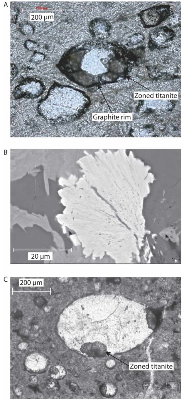
Fig. 5 (A) Photomicrograph in plane polarised light showing spheroids in OU 74178. Note dark black graphite rim on edge of spheroids and titanite growing from edges of spheroid towards centre. (B) SEM backscattered electron photomicrograph showing radial morphology of a titanite grain contained within a spheroid. Titanite appears to nucleate from a point on the bottom right of photomicrograph. (C) Photomicrograph in plane polarised light showing spheroids in OU 74178. Note zoning within titanites and both quartz (dominant infilling material in large, central spheroid) and potassium feldspar (right-hand side of large, central spheroid).
