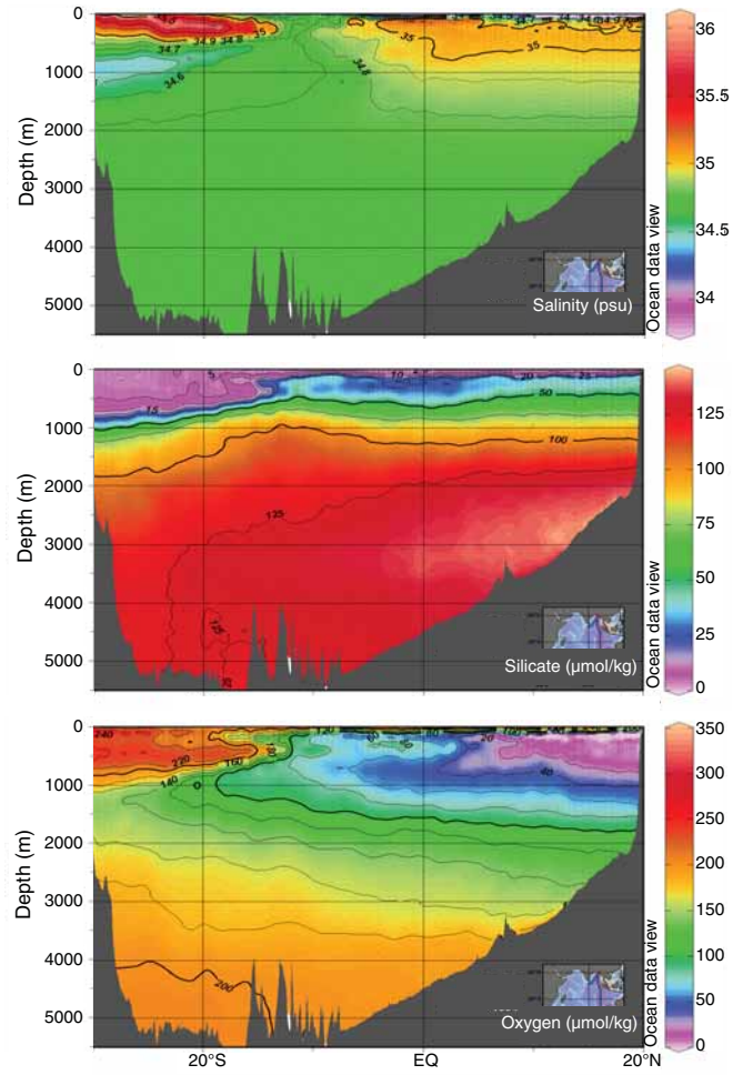
Figure F13. Salinity, silicate, and oxygen from eastern Indian Ocean WOCE meridional Transect 109, eastern Indian Ocean (from eWOCE Gallery, www.ewoce.org/gallery [Schlitzer, 2000]).
