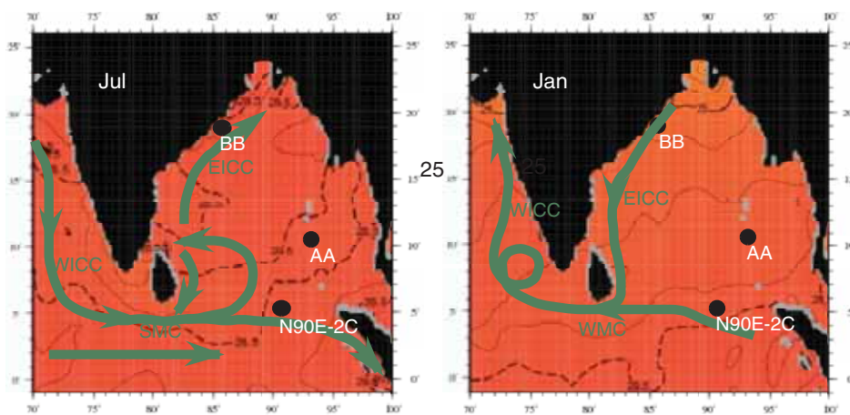
Figure F10. World Ocean Atlas Monthly Mean Temperature (°C) for 1955–2006 (Locarnini et al., 2010). Summer and winter monsoon current systems follow Schott and McCreary (2001). Proposed site locations in the Andaman Sea (AA), Mahanadi basin, Bay of Bengal (BB), and N90E-2C (redrill ODP Site 758) are shown. EICC = East Indian Coastal Current, WICC = West Indian Coastal Current, SMC = Southwest Monsoon Current, WMC = Winter Monsoon Current.
