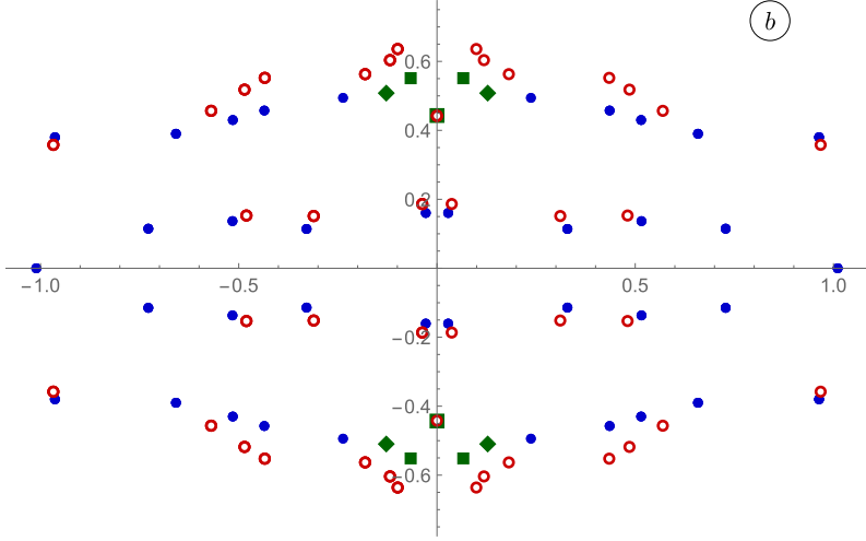
Fig. 15. The open circles depict the distribution of b(N) = \frac{n}{4\pi} \log(B) in the complex plane, where B is the eigenvalue of the quasi-shift operator, for the 42 = 34 + 8 states with L = 3 , \bar{L} = 0 and w = 0 as indicated in Table 1. The filled circles, squares and diamonds correspond to the solutions b_* of eq. (18.14). For the circles \lim_{N \rightarrow \infty} \Im m(b_*(N)) = 0 , while for the squares, b_*(N) \rightarrow \pm \frac{9i}{20} as N \rightarrow \infty . The filled diamonds form two pairs which have the same value of \Im m(b_*(N)) and opposite real part. At large but finite N the diamonds from the upper pair collide at the imaginary axis at which point for one of the diamonds b_*(N) \rightarrow +\frac{9i}{20} while for the other one b_*(N) \rightarrow 0 . The N dependence of b_*(N) for the lower pair of diamonds is obtained from that of the upper pair via complex conjugation.
