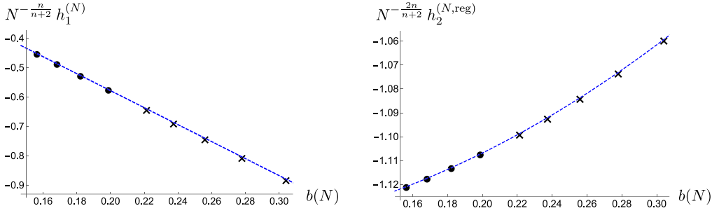
Fig. 10. The sums h_1^{(N)} and h_2^{(N,\text{reg})} \equiv h_2^{(N)} + \frac{N}{4 \cos(\frac{2\pi}{n+2})} were computed by solving the Bethe ansatz equations with the value of the parameters n = \frac{3}{2} , k = \frac{1}{10} and S^z = 0 . The solution sets were taken to be the ones corresponding to the primary Bethe states, which were discussed at the beginning of sec. 9. For the black dots, the integer m = M_- - M_+ was set to m = 2 , while N = 100, 200, 400, 800 . For the crosses m = 3 and N = 102, 202, 402, 802, 1602 . The numerical data is plotted versus b(N) . The latter was computed from the Bethe roots via eqs. (8.5) and (8.6). The dashed blue lines come from the predictions (11.13), (11.14) with the vacuum eigenvalues J_{1,2}^{(\text{vac})}(p, s) calculated through eq. (11.11). Note that the relative error between the numerical data and the analytical formula is of the order of 10^{-4} - 10^{-6} .
