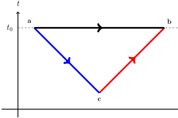
Fig. 17. The integration along the time slice t = t_0 (the segment \vec{ab} ) for the path ordered exponent \mathbf{M} in eq. (24.12) can be replaced by an integration along the characteristics: u = t_0 with t_0 < \bar{u} < t_0 - 2\pi ( \vec{ac} ) and \bar{u} = t_0 - 2\pi with t_0 < u < t_0 + 2\pi ( \vec{cb} ).
