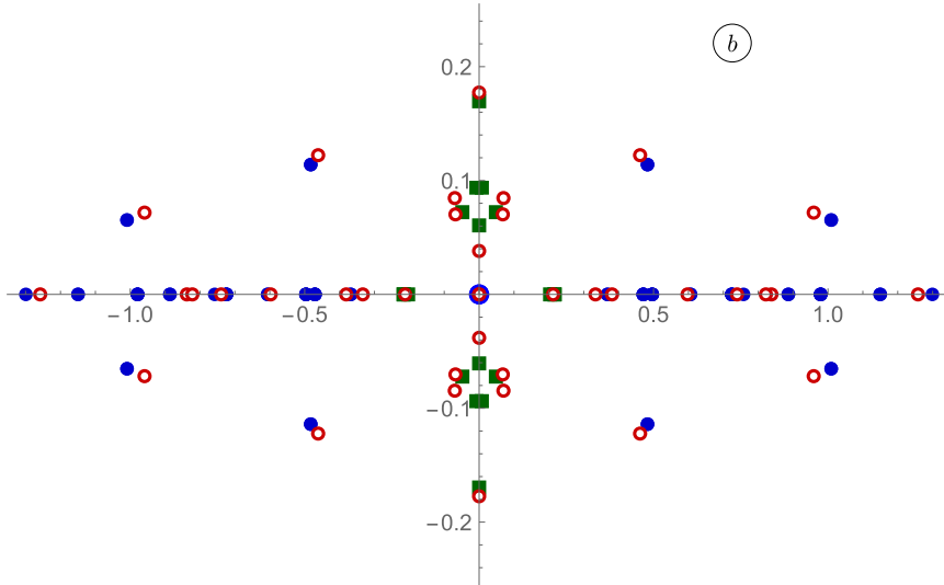
Fig. 26. The value of b(N) for the 37 = 21 + 16 states (open circles) with w = 1 and any values of L and \bar{L} .
