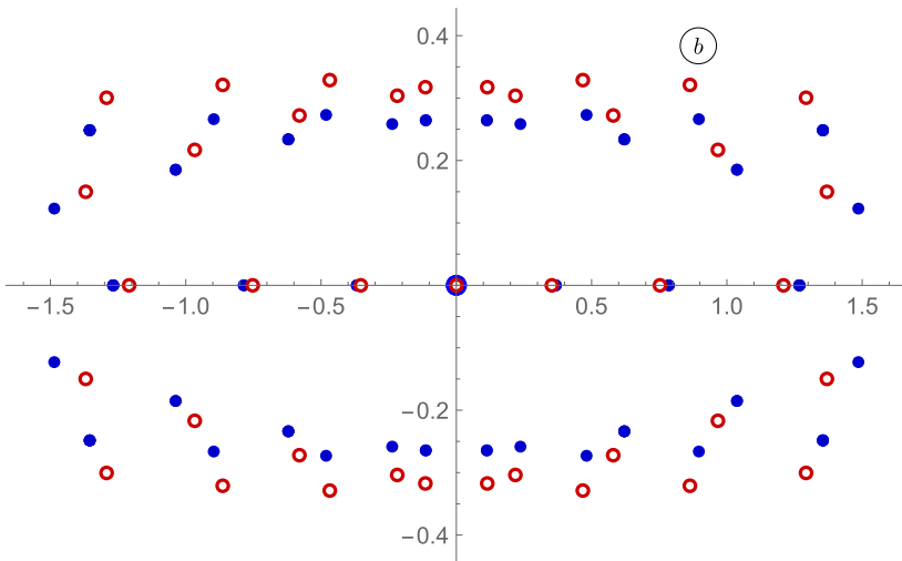
Fig. 22. The value of b(N) for the 40 = 40 + 0 states (open circles) having w = 0 and (\mathbb{L}, \bar{\mathbb{L}}) = (0, 2) .
