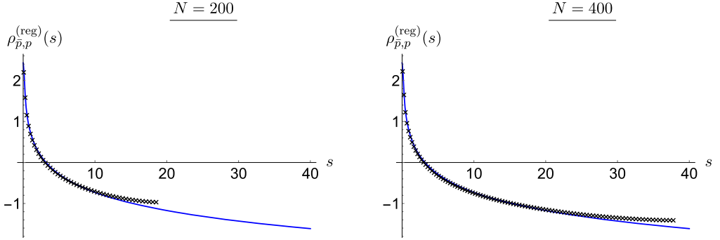
Fig. 6. For the two cases N = 200, 400 with the parameters taken to be S^z = 0 , k = \frac{1}{10} , n = 3 , the Bethe states were constructed for which the Bethe roots are real with M_+ of them being positive and M_- being negative, i.e., \{\zeta_m\}_{m=1}^M = \{\zeta_m^{(+)} > 0\}_{m=1}^{M_+} \cup \{\zeta_m^{(-)} < 0\}_{m=1}^{M_-} . Note that when |M_- - M_+| \ll N these states are part of the low energy spectrum with \mathbb{L} = \bar{\mathbb{L}} = w = 0 . The corresponding values of b = b_m were computed for m \equiv M_- - M_+ = 0, 2, 4, \dots, \frac{N}{2} and the crosses on the plots represent (b_{m+1} - b_m)^{-1} - \frac{2}{\pi} \log\left(\frac{N}{2N_0}\right) as a function of s = (b_{m+1} + b_m)/2 . The blue line depicts \rho_{\bar{p},p}^{(\text{reg})} = \rho_{\bar{p},p}^{(0,0)}(s) - \frac{2}{\pi} \log\left(\frac{N}{2N_0}\right) , where \rho_{\bar{p},p}^{(0,0)}(s) is the density of primary Bethe states given in eq. (9.8).
