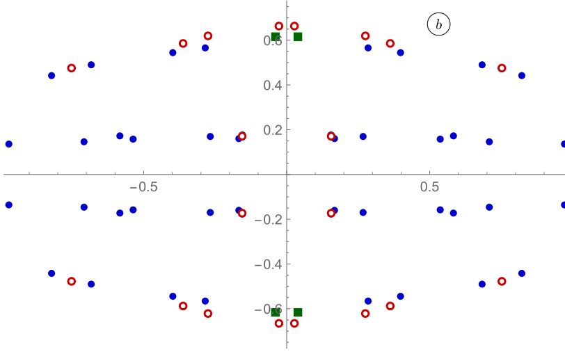
Fig. 23. The value of b(N) for the 20 = 16 + 4 states (open circles) having w = 0 and (L, \bar{L}) = (2, 1) .
