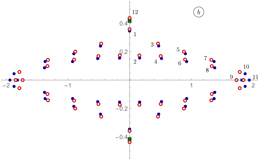
Fig. 20. The value of b(N) for the 40 = 38 + 2 states (open circles) having w = 0 and (\mathbb{L}, \bar{\mathbb{L}}) = (1, 0) , (0, 1) . The 12 states with \Re e(b(N)) \geq 0 and \Im m(b(N)) \geq 0 are numbered consistently with Fig. 9, where the N dependence of b(N) for the corresponding RG trajectories is plotted.
