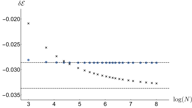
Fig. 7. The value of \delta\mathcal{E} = \frac{N}{4\pi v_F} (\mathcal{E} - e_\infty N) is plotted as a function of \log(N) for two RG trajectories in the case n = 3 and k = 0.235 > \frac{1}{n+2} . The blue dots depict \delta\mathcal{E} for the trajectory having \mathbb{L} = \bar{\mathbb{L}} = S^z = w = 0 and with s = 0 . If \log(N) \lesssim 4.5 the corresponding Bethe state is the ground state of the Hamiltonian \mathbb{H} . For the second RG trajectory (crosses) the RG invariants \mathbb{L} , \bar{\mathbb{L}} , S^z , w are also zero but s = \frac{i}{2}((n+2)k - 1) = \frac{7i}{80} is a pure imaginary number. The dashed lines denote the limiting values \delta\mathcal{E} = -0.0286\dots for the RG trajectory with zero s and \delta\mathcal{E} = -0.0337\dots for the other one.
