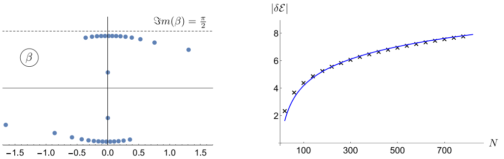
Fig. 3. The typical pattern of Bethe roots \beta_j = -\frac{1}{2} \log \zeta_j for one of the four states having B = K = -1 , with n = 3 , \pi k = 18/100 and N = 60 (left panel). The scaled energy \delta\mathcal{E} = \frac{N}{4\pi v_F} (\mathcal{E} - N e_\infty) for these states grows logarithmically for large N . The crosses in the right figure depict the numerical values of |\delta\mathcal{E}| found via the solution of the Bethe ansatz equations. The solid line comes from the fit \delta\mathcal{E} \approx -4.5702 - 0.2272i + (1.7724 - 0.4110i) \log(N) .
