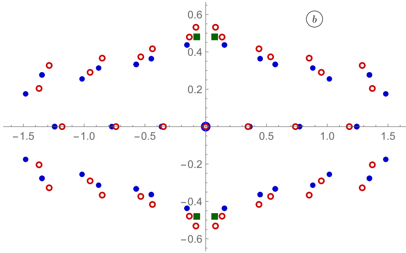
Fig. 21. The value of b(N) for the 40 = 36 + 4 states (open circles) having w = 0 and (\mathbb{L}, \bar{\mathbb{L}}) = (2, 0) .
