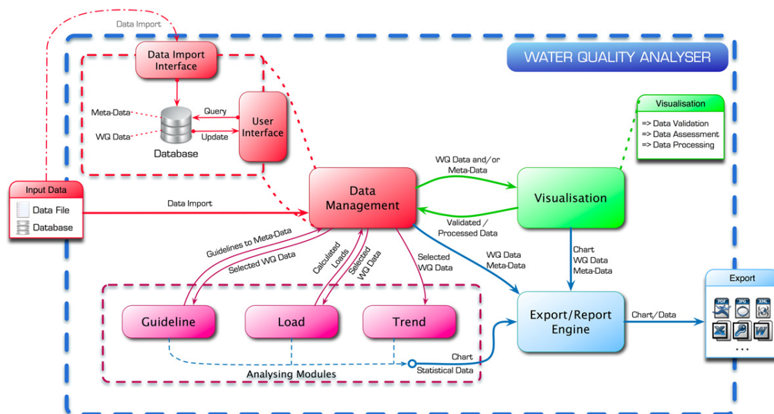
Figure 1. Architecture of the latest version of Water Quality Analyser
