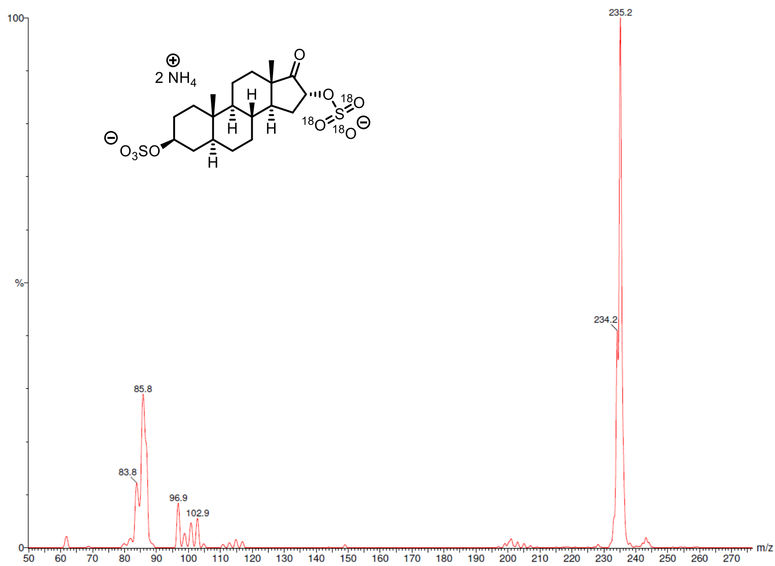
3β,16α-Dihydroxy-5α-androstan-17-one 3,16- 18 O 3 -bis(sulfate), ammonium salt LRMS
