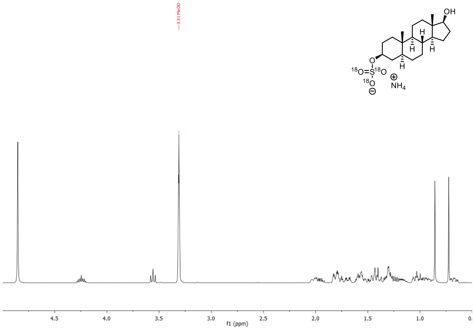
5α-Androstane-3β,17β-diol 3β[ 18 O 3 ]-sulfate, ammonium salt 1 H NMR 400 MHz, CD 3 OD
