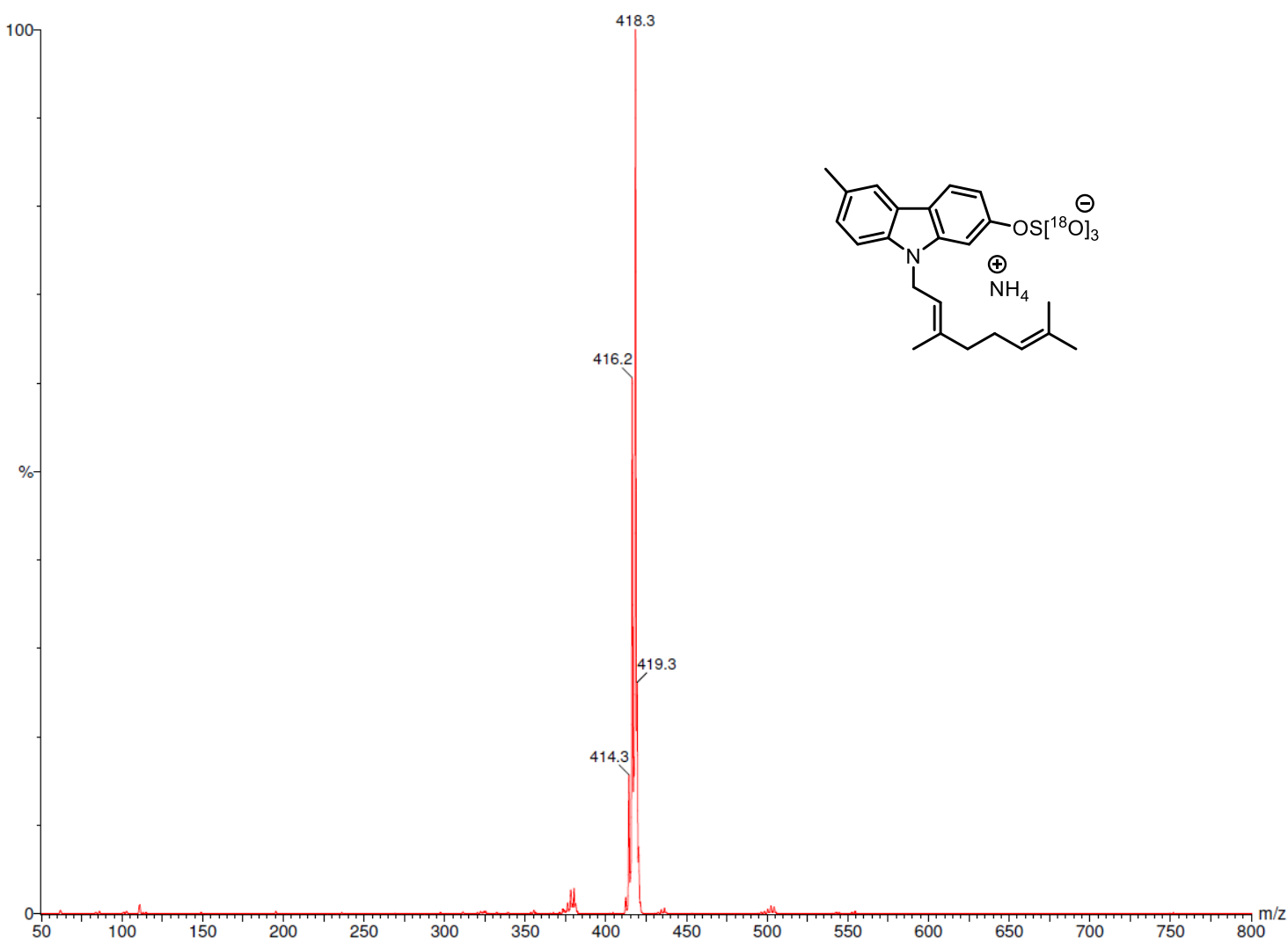
Karapinchamine A [ 18 O 3 ]-sulfate, ammonium salt LRMS
