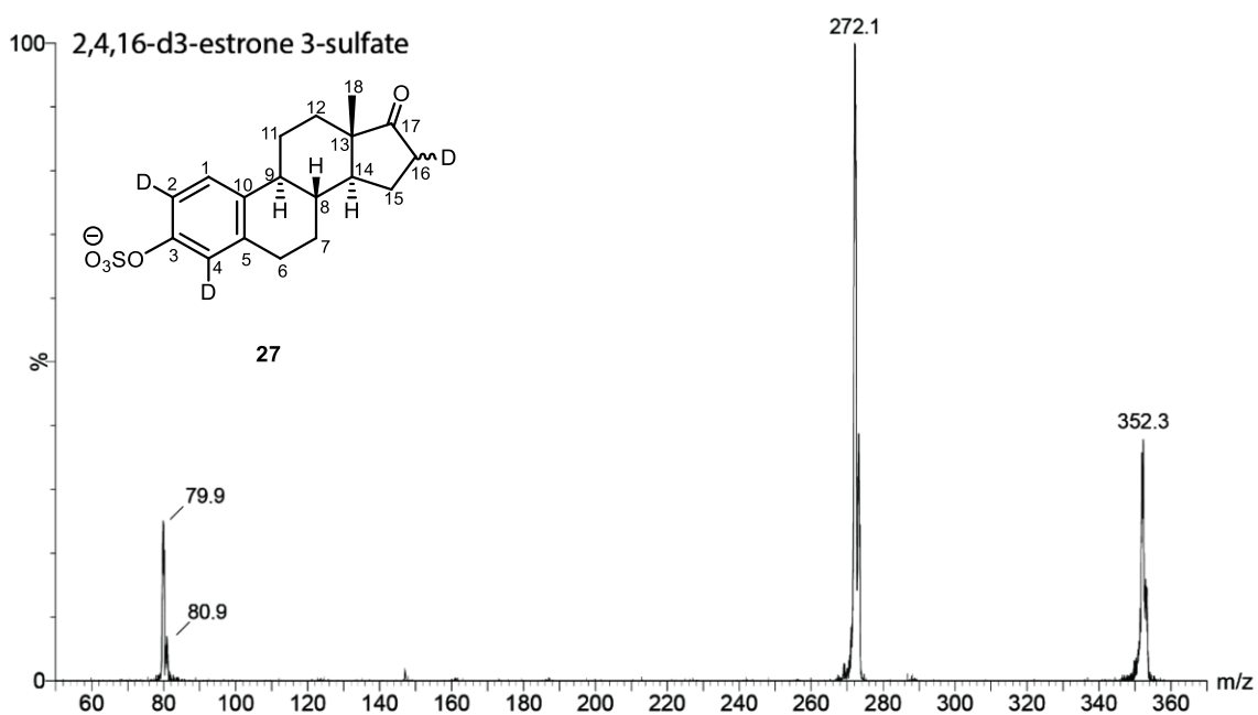
Figure S6: Product ion spectrum of 2,4,16-d 3 -estrone 3-sulfate ( 27 ), at a collision energy of 27 eV. This shows the formation of fragments m/z 80 ( ^*\text{SO}_3^- ) and m/z 81 ( \text{HSO}_3^- ).
