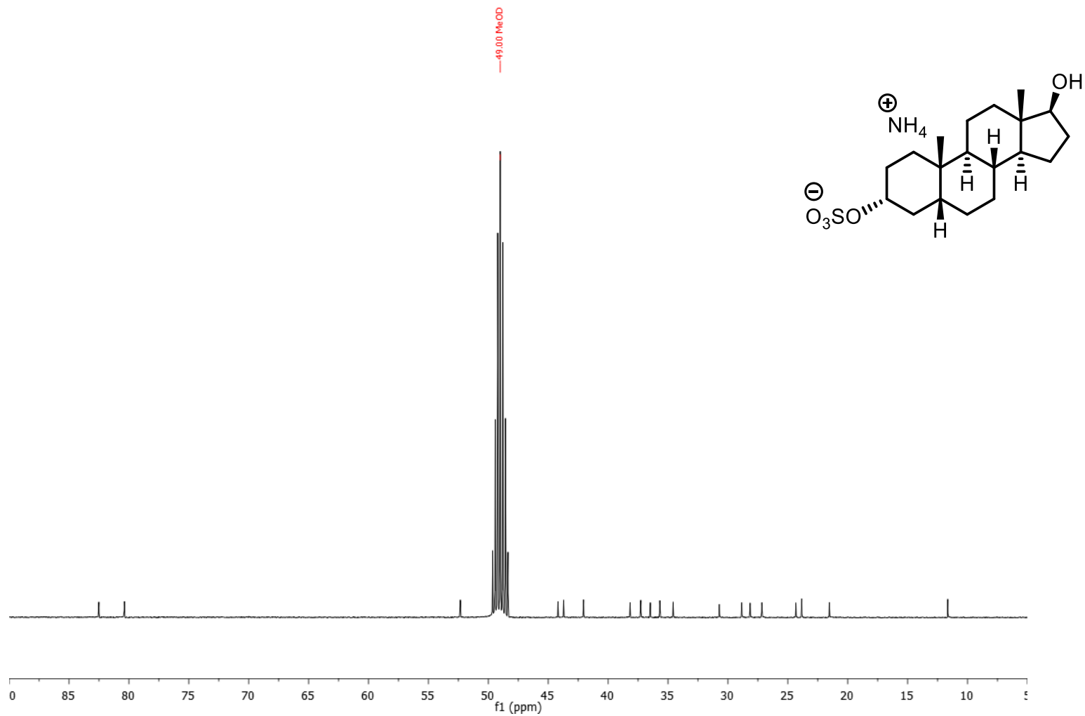
5β-Androstane-3α,17β-diol 3-sulfate, ammonium salt 13 C NMR 151 MHz, CD 3 OD
