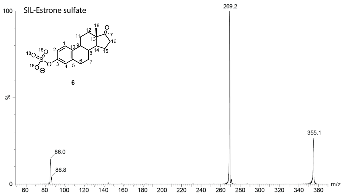
Figure S5: Product ion spectrum of SIL estrone sulfate ( 6 , m/z 355), at a collision energy of 27 eV. This shows the formation of SIL labelled fragments m/z 86 ( ^*\text{S}[^{18}\text{O}_3]^- ) and m/z 87 ( \text{HS}[^{18}\text{O}_3]^- ) in addition to m/z 269.
