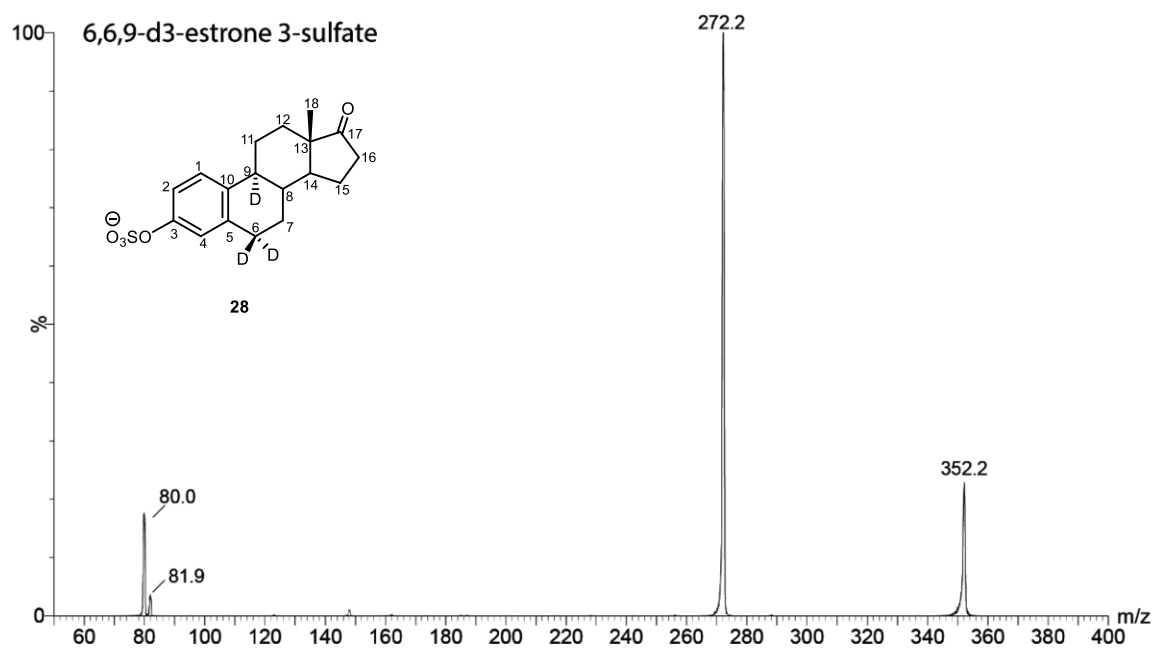
Figure S6: Product ion spectrum of 6,6,9-d 3 -estrone sulfate( 28 ), at a collision energy of 27 eV. This shows the formation of fragments m/z 80 ( ^{\bullet}\text{SO}_3^- ) and m/z 82 ( \text{DSO}_3^- ).
