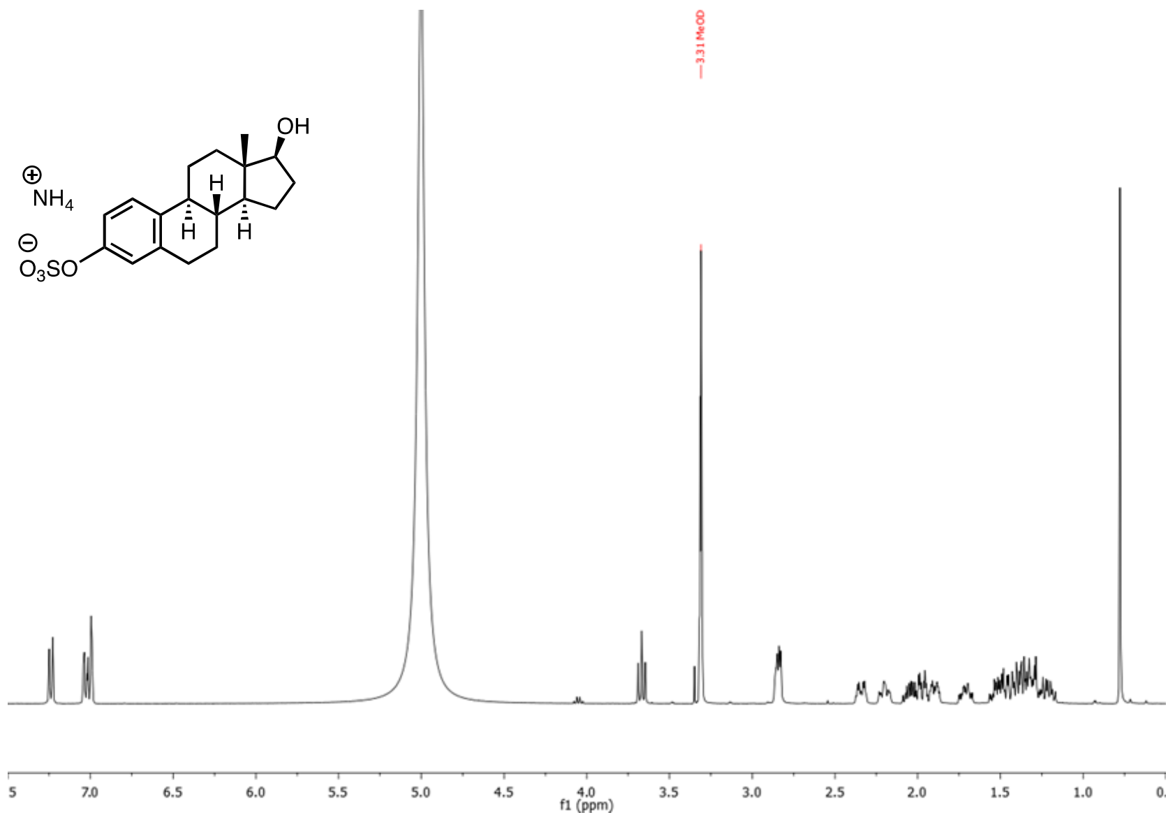
Estradiol 3-sulfate, ammonium salt ^1\text{H} NMR 400 MHz, \text{CD}_3\text{OD}
