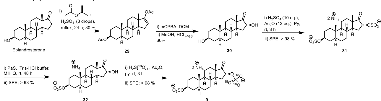
Scheme S 1: Selective labelling for 3 \beta ,16 \alpha -dihydroxy-5 \alpha -androstan-17-one 3,16[ ^{18}\text{O}_3 ]-bis(sulfate), ammonium salt ( 9 ). This commenced through the acetylation of epiandrosterone with isopropenyl acetate to form the corresponding diacetate ( 29 ). This was followed by epoxidation with m CPBA, to form the corresponding epoxide. Without further purification the epoxide was then subjected to acid hydrolysis to form the diol species ( 30 ). 1 This was followed by the formation of the unlabelled bis(sulfate) ( 31 ), using unlabelled sulfuric acid. The bis(sulfate) ( 31 ) was then subjected to selective cleavage of the 16-sulfate through the use of the Pseudomonas aeruginosa arylsulfatase ( PaS ) enzyme. 2,3 Hydrolysis at the 16 position was indicated by the up-field shift of the C16-H doublet, from \delta 4.93 to 4.31, which has previously been reported. 2 This gave the diol mono-sulfate ( 32 ), which was subjected to sulfation using labelled sulfuric acid to give compound ( 9 ).
