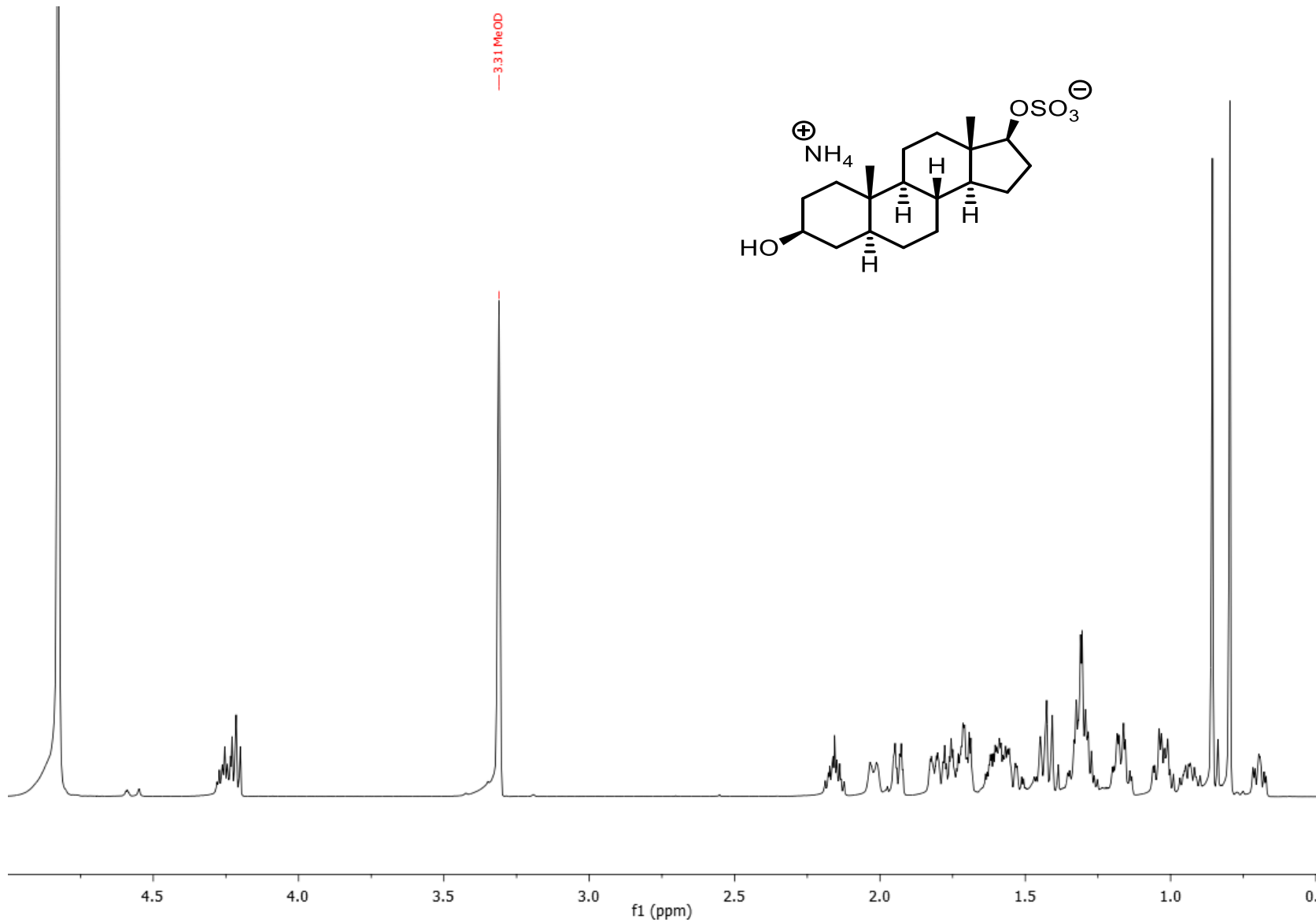
5 \alpha -Androstane-3 \beta [ ^{18}\text{O}_3 ],17 \beta -diol bis(sulfate), ammonium salt ^1\text{H} NMR 400 MHz, \text{CD}_3\text{OD}
