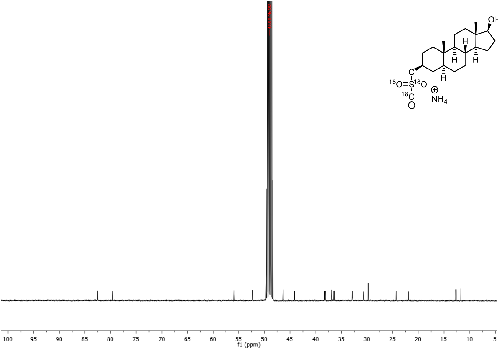
5α-Androstane-3β,17β-diol 3β[ 18 O 3 ]-sulfate, ammonium salt 13 C NMR 176 MHz, CD 3 OD
