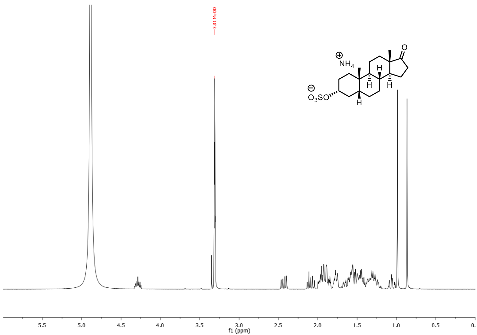
Etiocholanolone 3-sulfate, ammonium salt (3a) ^1\text{H} NMR 400 MHz, \text{CD}_3\text{OD}
