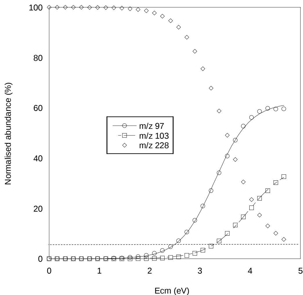
Figure S9: Breakdown curves modelled by Eq.1, for 5 \alpha -androstane-3 \alpha ,17 \beta -diol 3,17[ ^{18}\text{O}_3 ]-bis(sulfate) ( 12 ) ( m/z 228) and product ions hydrogen sulfate ( m/z 97 and m/z 103). The dissociation threshold E_{5\%} for each product ion is calculated from the model as described by Eq.1, as the energy E_{cm} when the normalised area is equal to 5% (Eq. 2). The E_{5\%} displayed are provided for visual demonstration. Fitting parameters, m/z 97 (BR = 63, Chi Squared, \chi^2 = 7 ) and m/z 103 (BR = 37, Chi Squared, \chi^2 = 1 ). Line indicates 5% normalised abundance.
