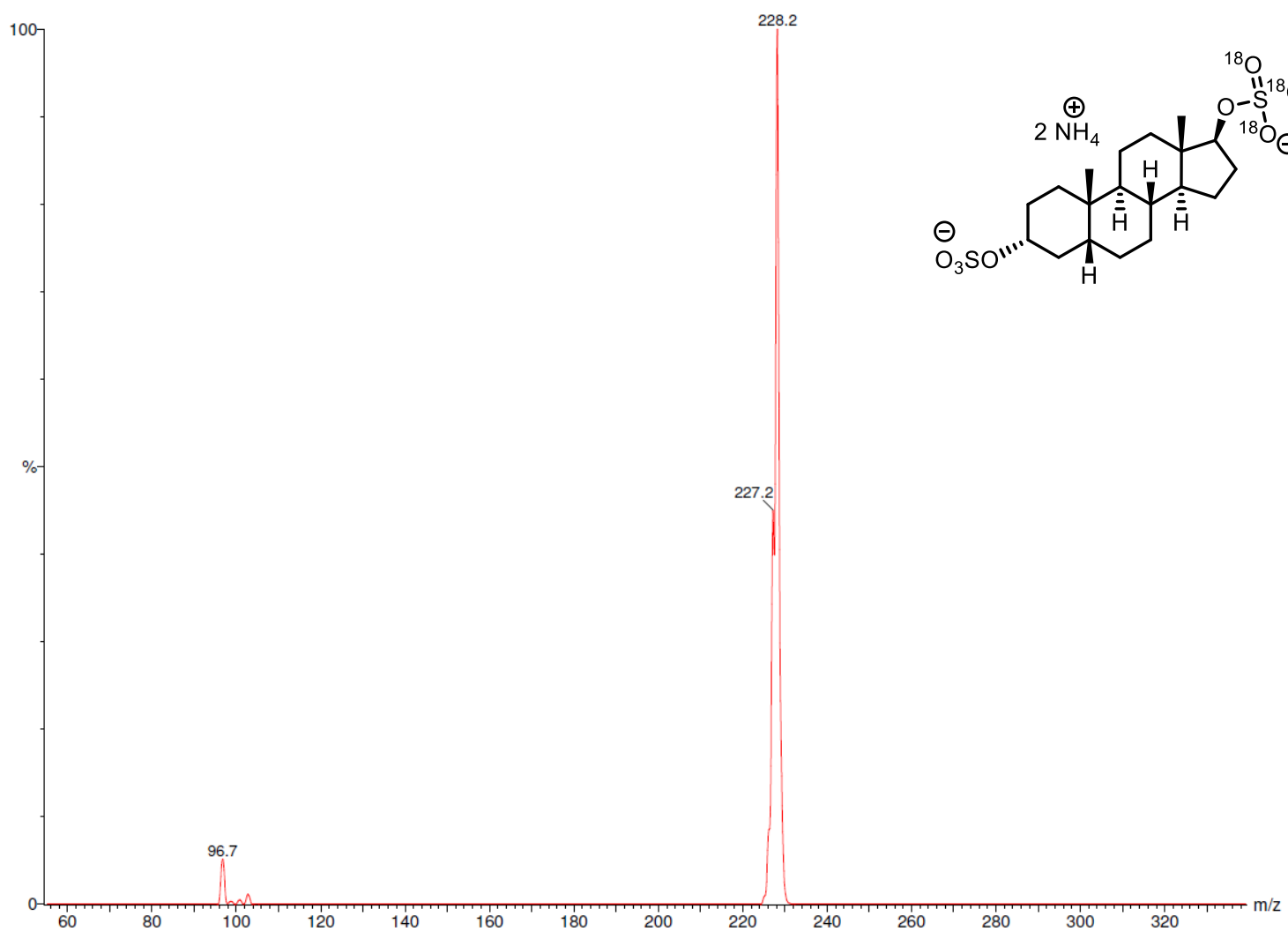
5β -Androstane-3α,17β[ 18 O 3 ]-diol bis(sulfate), ammonium salt LRMS
