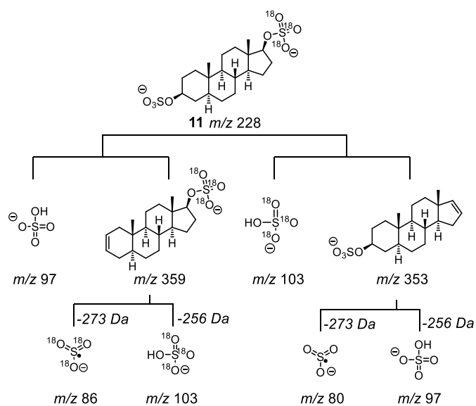
Figure S2: Fragmentation pathways for 5 \alpha -androstane-3 \beta ,17 \beta -diol bis(sulfate) ( 11 ) based on MS/MS and pseudo MS 3 CID experiments.
