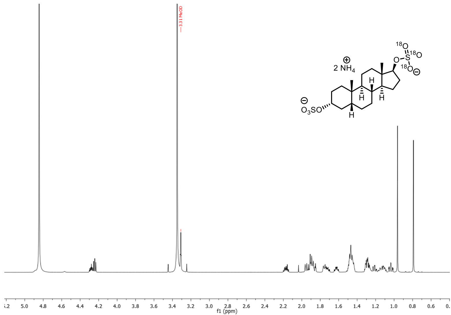
5 \beta -Androstane-3 \alpha ,17 \beta [ ^{18}\text{O}_3 ]-diol bis(sulfate), ammonium salt ^1\text{H} NMR 400 MHz, \text{CD}_3\text{OD}
