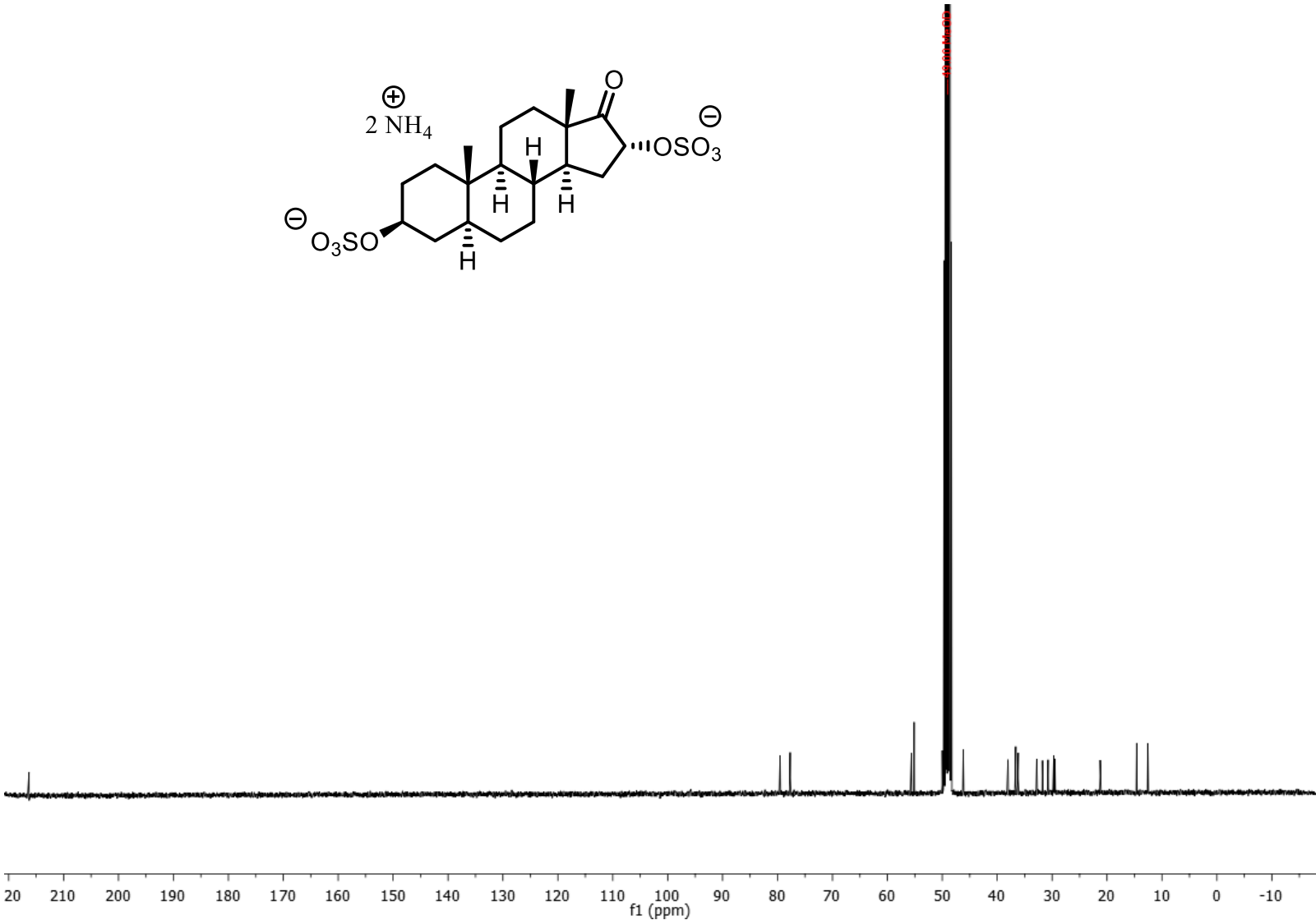
3β,16α-Dihydroxy-5α-androstan-17-one 3,16-bis(sulfate), ammonium salt 13 C NMR 101 MHz, CD 3 OD
