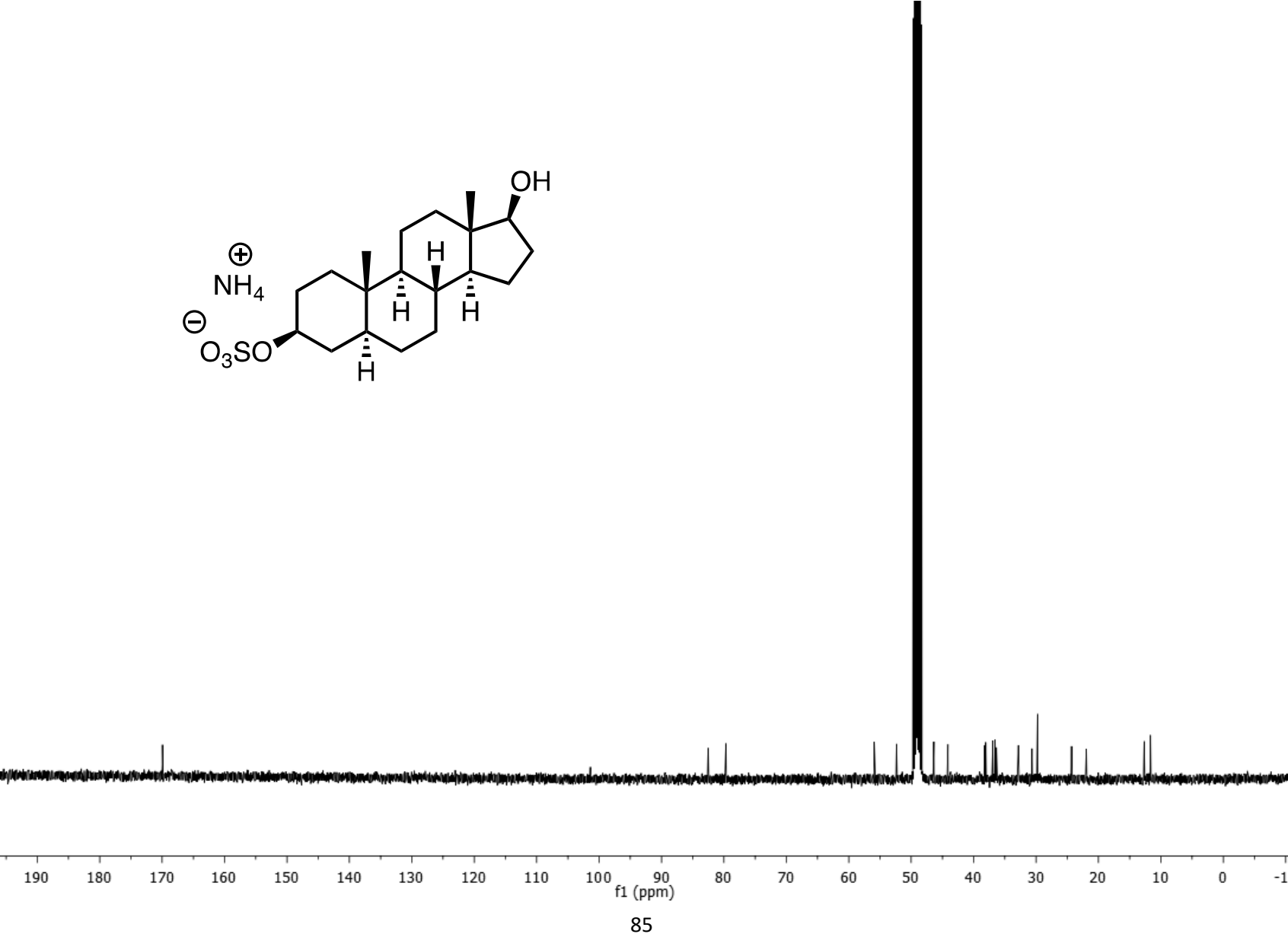
5 \alpha -Androstane-3 \beta ,17 \beta -diol 3-sulfate, ammonium salt ^{13}\text{C} NMR 101 MHz, \text{CD}_3\text{OD}
