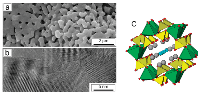
Figure 1. Morphology of HAP: (a) SEM, (b) TEM, and (c) structure drawings of \text{P63/m} [\text{Ca}_4\text{Ca}^{\text{II}}_6](\text{PO}_4)_6(\text{OH})_2 hydroxyapatite. The green polyhedra indicate \text{CaO}_6 metaprisms, the yellow polyhedra indicate \text{PO}_4 tetrahedra, gray spheres correspond to \text{Ca}^{\text{II}} , and blue spheres correspond to OH.
