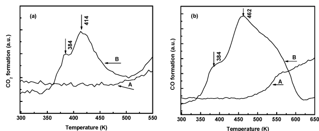
Figure 3. TPSR spectra of (a) \text{CO}_2 formation and (b) \text{CO} formation obtained from the reaction between \text{HCHO} and pre-adsorbed oxygen over (A) HAp and (B) \text{Pd} (3 wt %)/ \gamma\text{-Al}_2\text{O}_3 catalysts.
