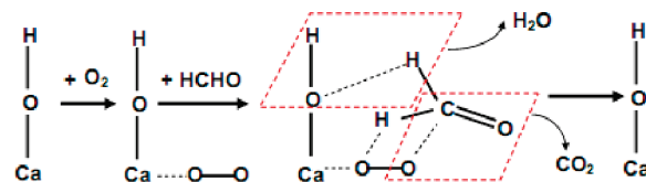
Figure 4. Scheme of \text{HCHO} combustion on HAp while hydroxyl groups connected to \text{Ca}^{2+} serve as active sites.
