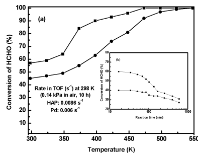
Figure 2. (a) HCHO combustion in the temperature range 298–550 K. (b) HCHO combustion at 298 K for 10 h. Catalysts, (■) Pd (3 wt %)/ \gamma - \text{Al}_2\text{O}_3 or (●) HAP; feed gas, 0.14 kPa HCHO, 2.6 kPa \text{H}_2\text{O} in air; GHSV, 36000 \text{ h}^{-1} . HCHO conversion was calculated on the basis of \text{CO}_2 formation.
