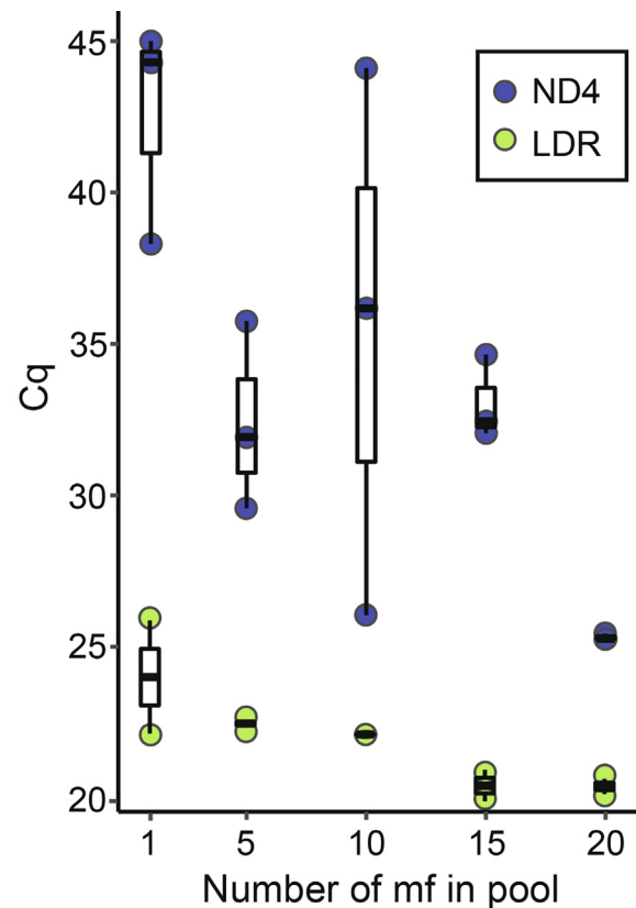
Fig. 2. Results of quantitative PCR for two primer sets using DNA extracted from pools of 1, 5, 10, 15, or 20 Wuchereria bancrofti microfilariae. Each point represents the cycle quantification, C_q , value, which is the cycle number at which a sample's fluorescence reaches the threshold for real signal. Smaller C_q values indicate earlier amplification, which can indicate higher concentrations of template DNA. Two runs are represented here: one targeting a nuclear repeat called LDR and the other targeting a portion of a mitochondrial gene ND4. Two replicates per sample were performed for LDR, while three were performed for ND4.
