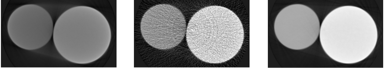
Figure 2: Tomographic reconstruction of (L) mean data, P , (C) BH correction of mean data as P(E_0/E)^3 , (R) Linearisation BHC of mean by power law as 1.39P^{1.25} . Greyscale [-0.05, 0.35)\text{mm}^{-1} .
