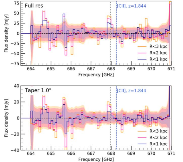
Figure 2. ALMA Band 9 spectrum of SL2S 0217 at 100 MHz ( 45 \text{ km s}^{-1} ) resolution, extracted for the full-resolution and 1''.0 taper images, and the three source-plane apertures. The shaded regions indicate \sigma_{\text{rms}} for each channel. We obtain a tentative ( 3\sigma – 4\sigma ) [C II] 158 \mu\text{m} detection at 667.97 GHz (offset from the systemic velocity by \sim 50 \text{ km s}^{-1} ).
