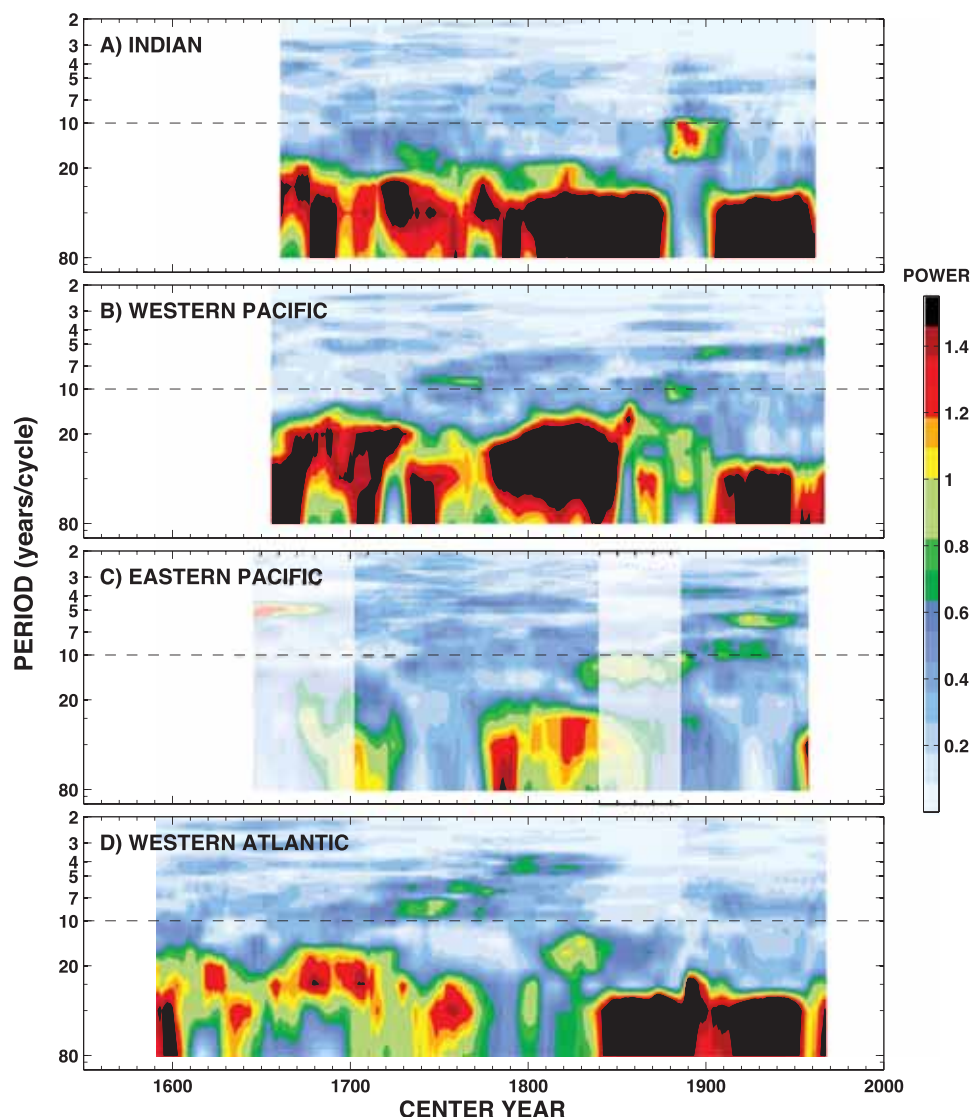
Figure 7. (a–d) Evulsive (50 year window) multitaper method spectra of the best reconstructions for each basin. Portions of the reconstruction where RE \leq 0 are shaded in white. The black dashed horizontal line in each panel indicates the 10 year periodicity.
