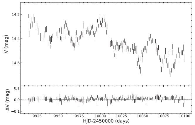
Figure 2. The final calibrated and binned V-band light curve for NGC 3227. For comparison with the AGN variations and uncertainties, the bottom panel shows the scatter in residuals for a non-varying field star of similar brightness.
