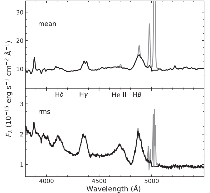
Figure 3. Mean (top) and rms (bottom) spectra of NGC 3227 based on the observed-frame spectra obtained throughout the monitoring program. The strong broad emission lines are labeled for ease of identification. The spectra traced in black (gray) have the narrow lines subtracted (included).
