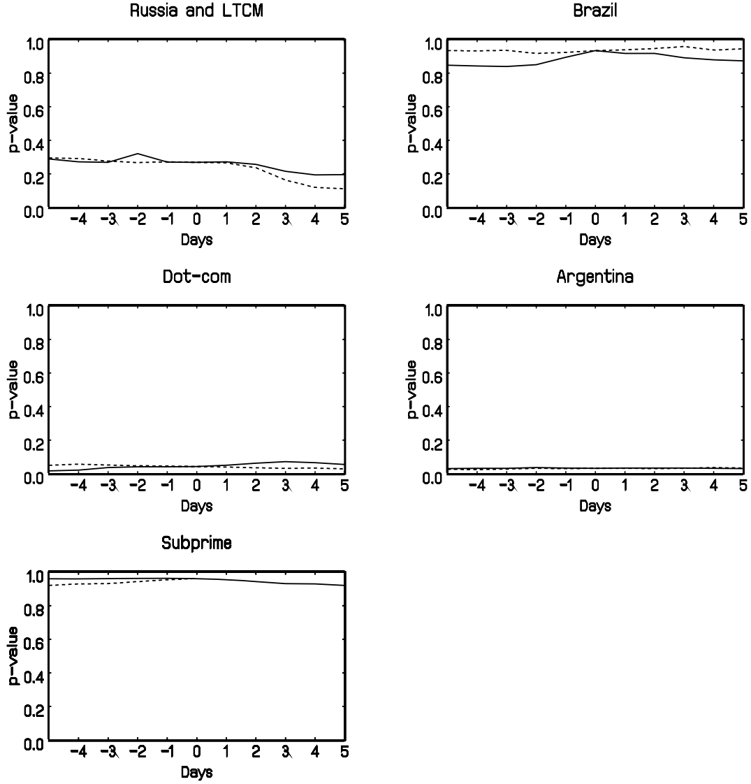
Figure 2: Model over-identification test p-values for sensitivity to crisis date selection: -5,4,...0,...+4,+5 days. Continuous (dashed) line represents the start (end) of the crisis period. The p-values at zero correspond to the values reported in Table VII. where the number of common factors is three.
