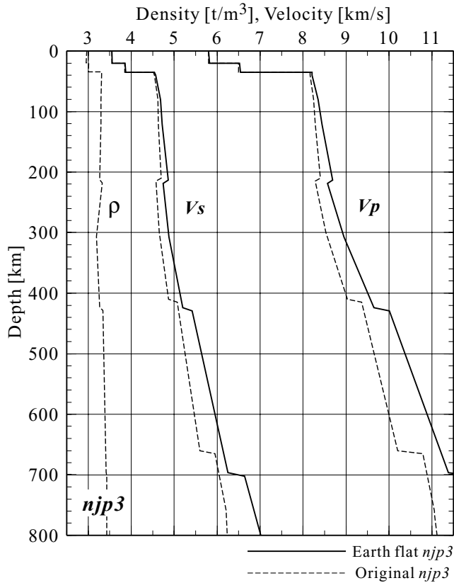
Figure 9. The depth variation of P - and S -wave velocity and density of Australian lithosphere ( njp3 ; dashed lines) used in the 2-D numerical modelling and modified V_p and V_s by using the Earth flattening technique (solid lines).
