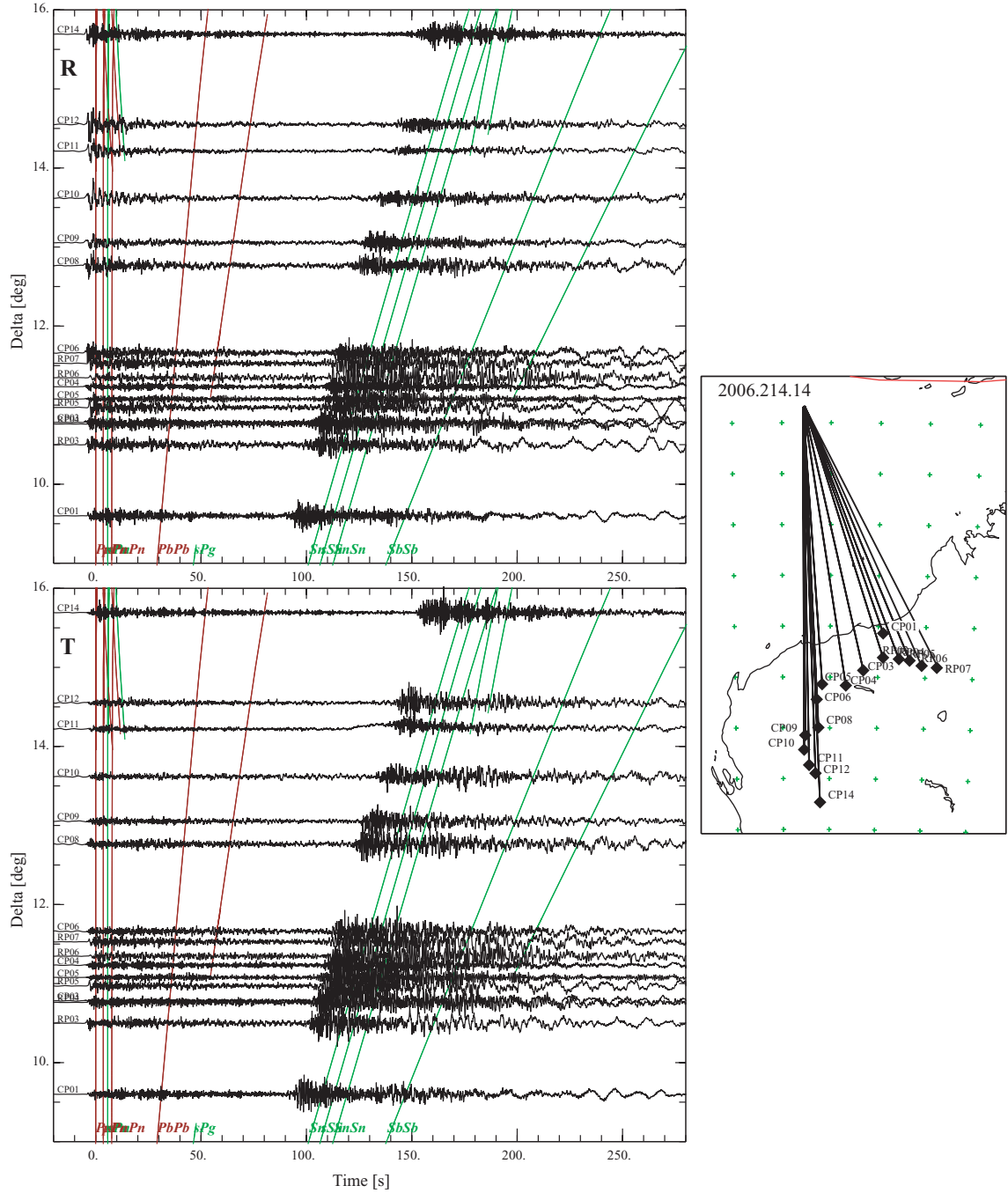
Figure 5. Record sections of radial and transverse component seismograms for a shallow event (15 km deep) at the front of the Java trench ( -11.17^{\circ}\text{S} 116.85^{\circ}\text{E} ) recorded across a network of portable seismic stations in northern Western Australia as shown in the map insert to the right. The seismograms are aligned on the expected P arrival times for the ak135 model, and the time trajectories of other phases are indicated. The ground velocity traces are unfiltered and normalized with respect to the three-component energy in the 5 min window.
