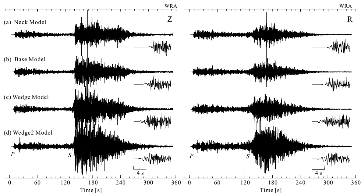
Figure 19. Synthetic seismograms for a receiver at WRA illustrating the change in the wave shape as the nature of the transition zone between the subduction zone and the Australian lithosphere changes for model (a)–(d); see Fig. 7.
