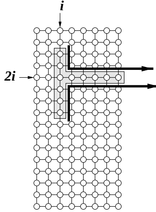
Figure 5: Development of queues in greedy transposing.
