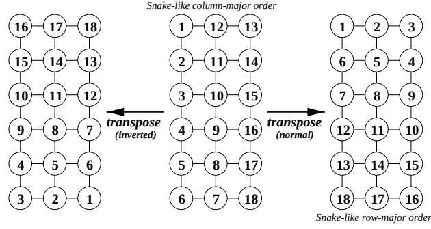
Figure 4: The transpose permutation.
