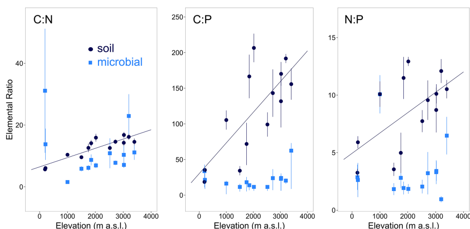
Figure 2. The relationships between soil and microbial C : N : P stoichiometry with elevation (194–3400 m a.s.l.). Total soil C : N, C : P and N : P all significantly varied with elevation ( R^2 = 0.45, 0.36, 0.28 , respectively p < 0.05 ; see Table 2). Microbial C : P, C : N and N : P ratios did not vary with elevation. Values are means \pm 1 SE ( n = 5 replicates, which represents the spatial variation within a 1 ha plot).
