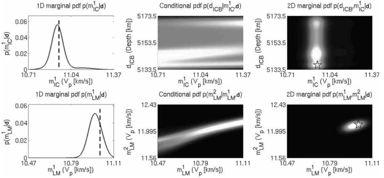
Figure 14. Construction of 2-D marginal posterior pdfs via eq. (9) for (first row) V_p at the top of the inner core ( m_{IC}^1 ) and the ICB depth ( d_{ICB} ) and (second row) V_p in the lower mantle ( m_{LM}^1 and m_{LM}^2 ). See Tables 1 and 2 for the model parametrization. The three panels in each row show (left-hand panel) the 1-D marginal pdf, (middle panel) the conditional pdf and (right-hand panel) the 2-D marginal pdf for one of the patterns in the test set. Lighter colours denote higher probabilities. The corresponding target values are denoted by the black line (left-hand panel) and the cyan star (right-hand panel).
