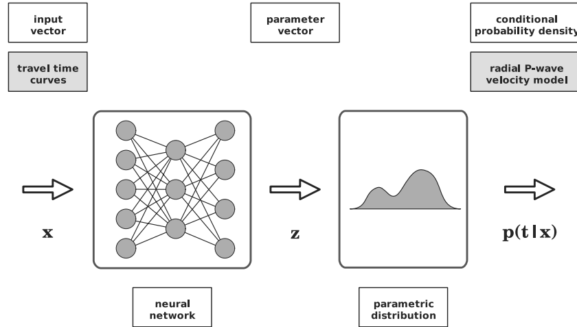
Figure 2. A Mixture Density Network (MDN), as introduced by Bishop (1995). The output of an MDN approximates a parametric distribution p(\mathbf{t}|\mathbf{x}) for the target \mathbf{t} , conditioned on the input \mathbf{x} . The parameters describing this distribution are given by the output \mathbf{z} of a neural network, such as the MLP shown in Fig. 1. In this study, the input consists of traveltime data \mathbf{d} , while the target represents the parameters of interest \mathbf{m}' , which form a subspace of the l -dimensional radial P -wave velocity earth model \mathbf{m} (eqs 1 and 2).
