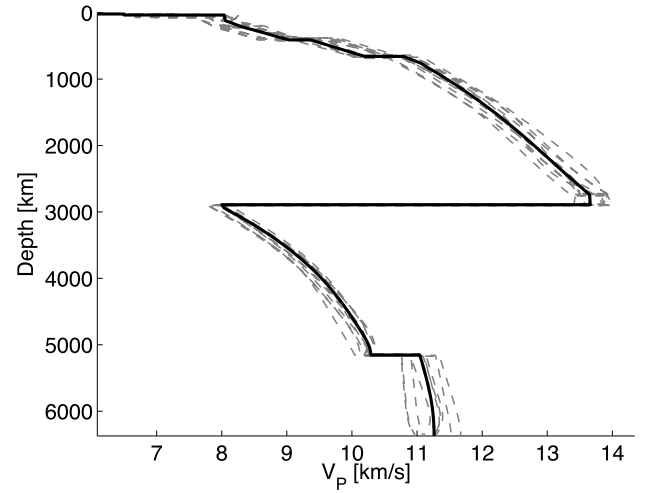
Figure 4. Ten model realizations (red), drawn from the prior distribution \rho(\mathbf{m}) and ak135 (black) for V_P .
