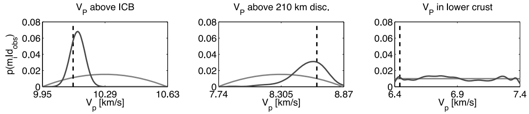
Figure 10. 1-D marginal posterior pdf (blue line), prior pdf (red) and true model value (black, dashed) for one pattern in the test data set for V_P (left-hand frame) directly above the ICB, (middle frame) directly above the 210 km discontinuity and (right-hand frame) in the lower crust.
