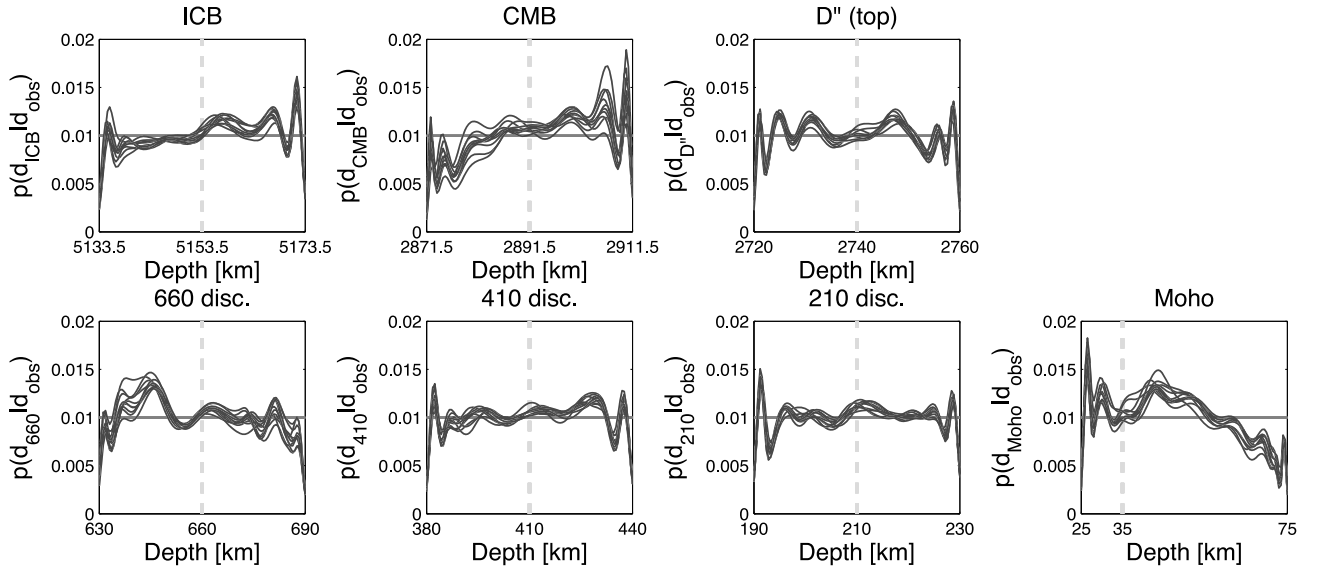
Figure 13. 1-D marginal posterior pdf (blue line), prior pdf (red) for the seven discontinuity depths (Table 1). Trained networks are applied to 10 different EHB input patterns (Fig. 9).
