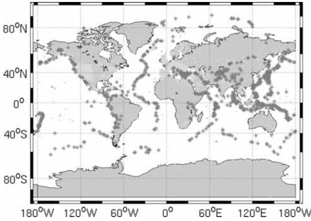
Figure 6. Locations of 1100 sources (red asterisks) and 5268 stations (green dots) in the EHB data for 2001–2008. Event depths are restricted to lie between 14 and 16 km.
