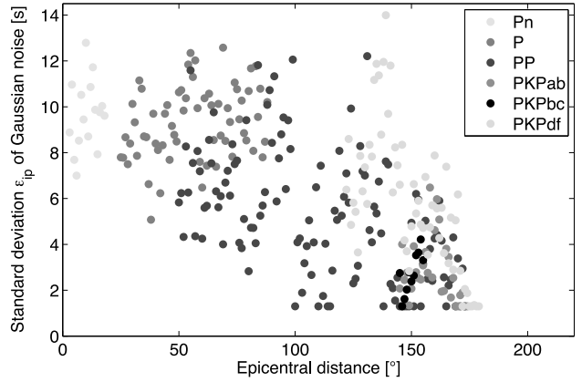
Figure 7. The half-width of the spread in the observed traveltimes \epsilon_{ip} is used as the standard deviation of the Gaussian noise model, which differs for every phase p and epicentral distance i . Different colours denote different phases.
