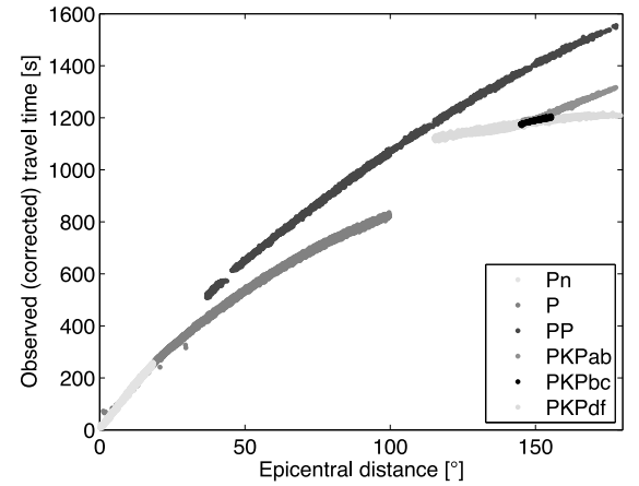
Figure 5. Travel time measurements in the EHB bulletin for 2001–2008. Event depths are restricted to lie between 14 and 16 km.
