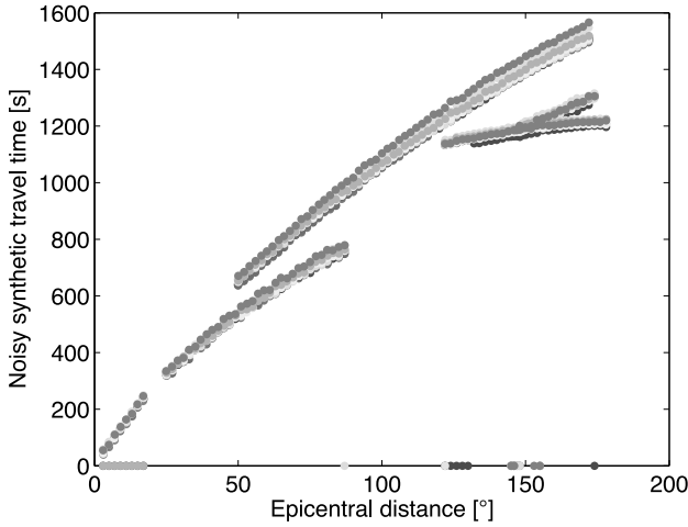
Figure 8. Examples of noisy synthetic traveltime data that form the input to the network. The synthetic data are sampled at distance intervals of 2^\circ for the epicentral distance ranges specified in Table 3. Note the zeros in the traveltime curves, which indicate that TauP did not compute an arrival at the corresponding distance.
