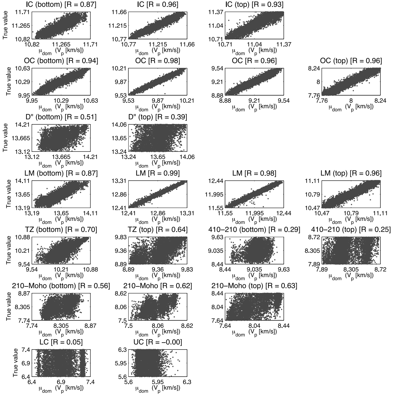
Figure 11. Mean \mu_j (eq. 6) of the dominant Gaussian kernel (maximum \alpha_j in eq. 5), labelled \mu_{dom} in the figure, versus the true synthetic value for all patterns in the test data set for the 22 V_P parameters (Tables 1 and 2). The regions where discontinuities are displayed on different rows. For every region, depth decreases from left to right in the figure. The corresponding correlation coefficient R is given above each frame.
