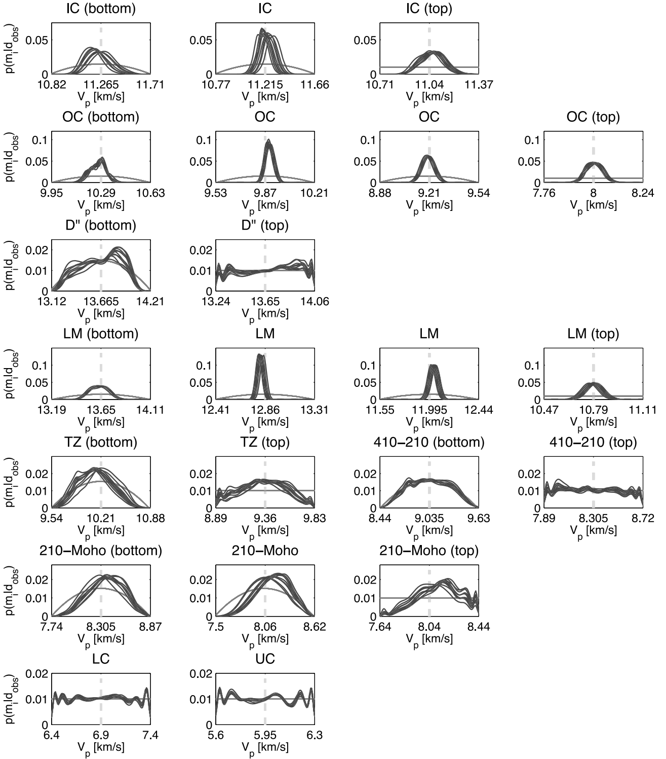
Figure 12. 1-D marginal posterior pdf (blue line), prior pdf (red) for the 22 V_p parameters (Tables 1 and 2). The same trained networks as used for Fig. 10 are applied to ten different EHB input patterns (Fig. 9). The regions between discontinuities are displayed on different rows. For every region, depth decreases from left to right in the figure. Note that the range of the vertical axis, that is, normalized probability, differs between rows.
