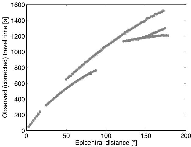
Figure 9. Ten input patterns, which are constructed from the EHB data (Fig. 5). Note that the variation in these real data vectors is significantly smaller than the variations between synthetic training patterns (Fig. 8).
