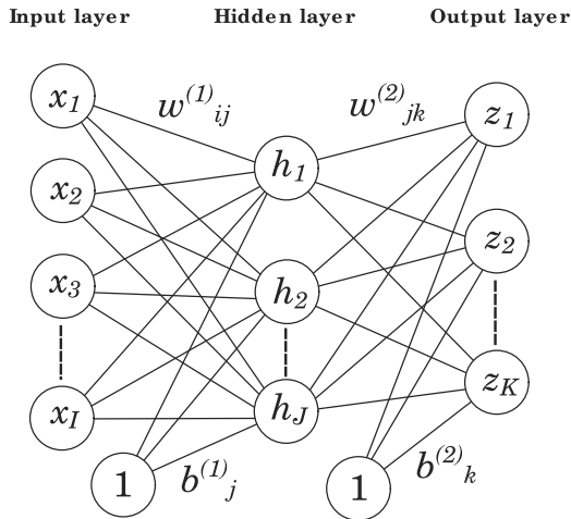
Figure 1. A two-layer feed-forward Multilayer Perceptron (MLP). The lines represent the two layers of free parameters in the network, represented by the weights w_{ij}^{(1)} and w_{jk}^{(2)} and biases b_j^{(1)} and b_k^{(2)} . The I input neurons x_i feed into the J hidden neurons h_j , which form the input to the K output units z_k . An additional input of value 1 feeds into the hidden and output layer, which is associated with the biases. Information flows only from the input to the output neurons (feed-forward).
