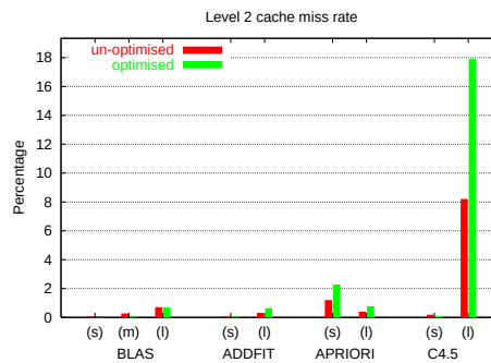
Fig. 5. Level-2 cache miss rates.
