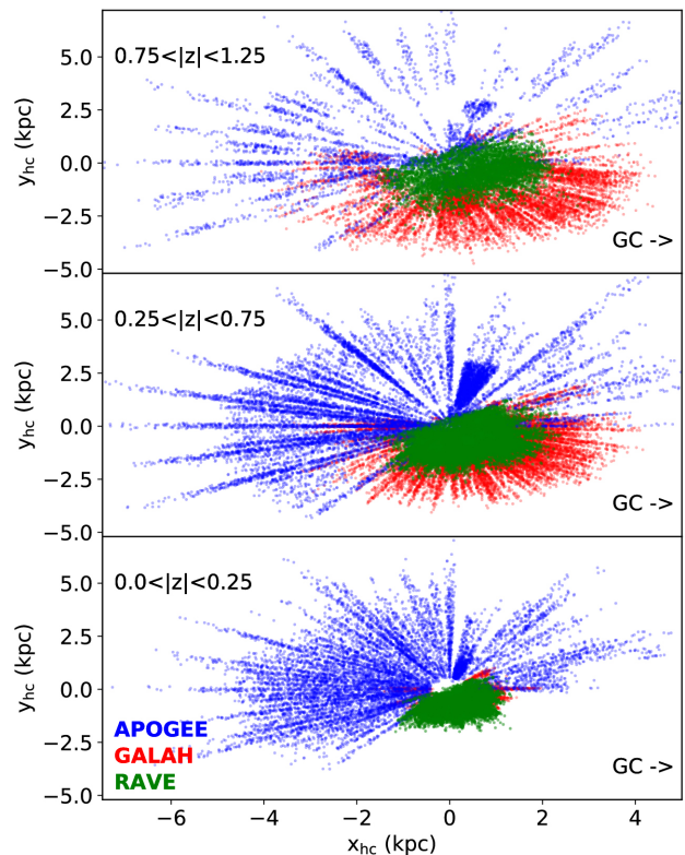
Figure 3. Distribution of GADR14RC in heliocentric (x, y) coordinates where the symmetrical regions above and below the plane have been merged together in slices in z (kpc). APOGEE probes deep into the disc while GALAH provides good coverage moving away from the plane, and to illustrate this also shown is the coverage of RAVE DR5.
