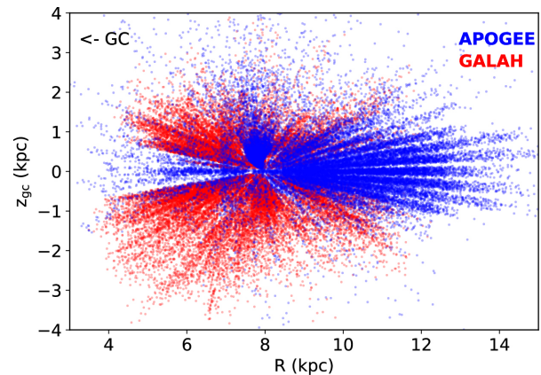
Figure 2. Distribution of the combined Red Clump dataset GADR14RC in Galactocentric R – z plane. While the APOGEE coverage dominates in plane and towards the anticentre, GALAH surveys the off-plane region more extensively.
