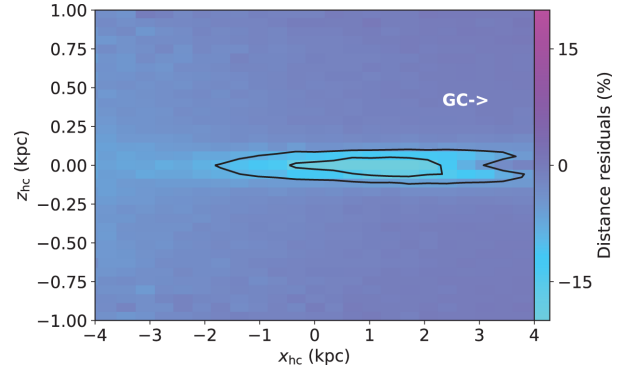
Figure 8. Properties of Red Clump stars for a H < 13.8 sample simulated with GALAXIA. We show the map of mean distance residuals (d_{RC} - d_{True})/d_{True} . It can be seen that close to the plane and towards the Galactic Centre, the distance is underestimated. The contours indicate the fraction of Red Clump stars (10 per cent and 40 per cent levels shown) that are unusually luminous, identified using M_{K_s} < -2.0 . This suggests that distance errors are due to luminous Red Clump stars.
