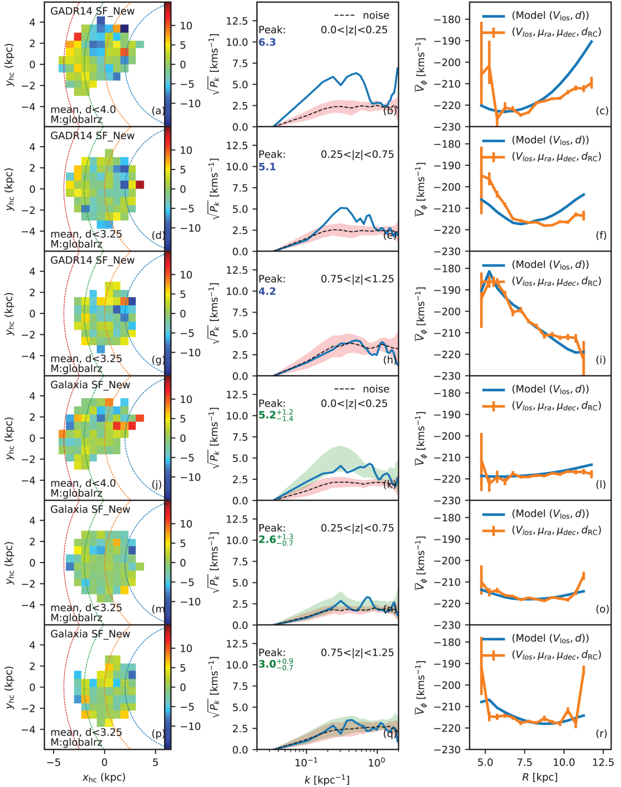
Figure 12. Residual V_{\text{los}} velocity maps, power spectrum, and \bar{V}_\phi profiles for observed and simulated data for different slices in z . The top three panels correspond to GADR14RC while the bottom three panels correspond to mock GALAXIA . In each case, the power spectrum corresponding to the velocity map is shown in blue, the 1\sigma noise spread based on 20 random realizations in pink, and median noise in dotted black. For GALAXIA the green region represents the stochastic spread over 100 realizations, in power spectrum with the same selection function as data. We find that except for the case of mid-plane the \bar{V}_\phi profiles are captured well by the globalRz models and the power spectrum of residual V_{\text{los}} velocity approaches noise with amplitude \approx 2 \text{ km s}^{-1} .
