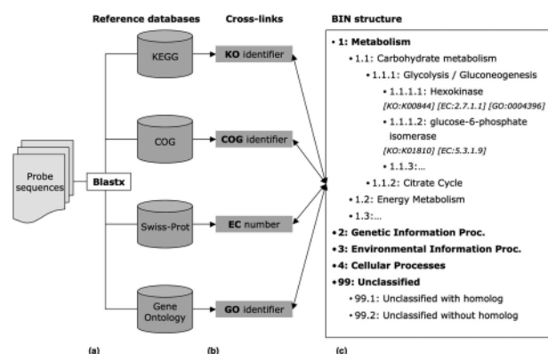
Fig. 1. The classification of new sequences is composed of three steps. First, using Blast, best matches are identified in reference databases for each sequence (a). Then, cross-links are extracted from the description of these database entries (b). Finally, sequences are assigned into the BIN Structure based on the relationship between cross-links and BINs (c).
