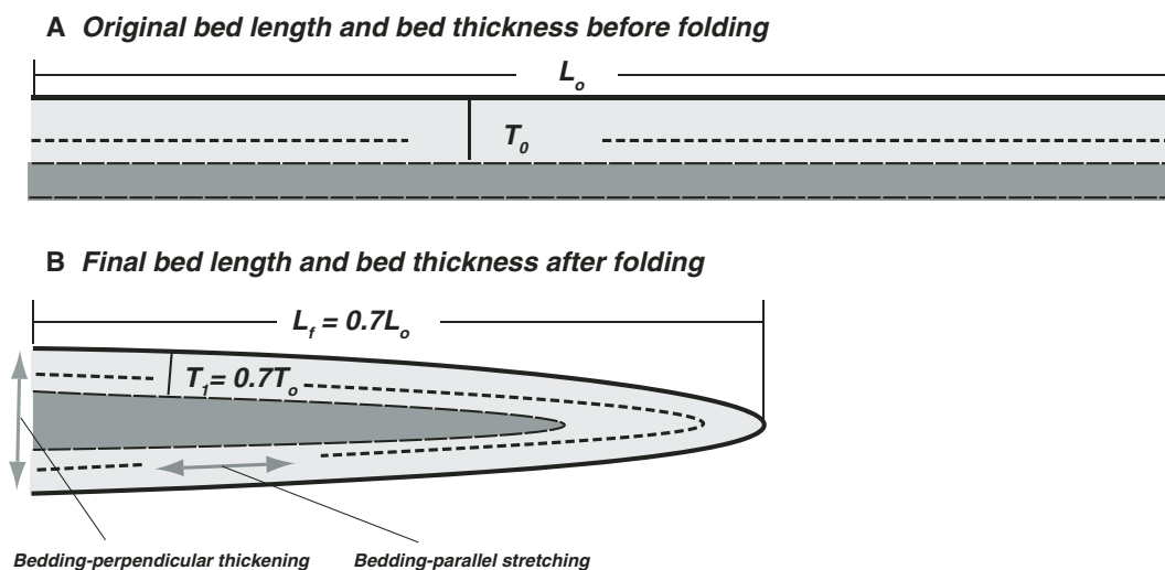
Figure 11. Schematic diagram showing the relationship between bedding-perpendicular thickening and bedding-parallel thinning during folding: (A) Bed before folding. (B) Bed after folding. Note that the overall section is thickened by 140%, while the marker bed in the fold limbs is thinned by 70%.
