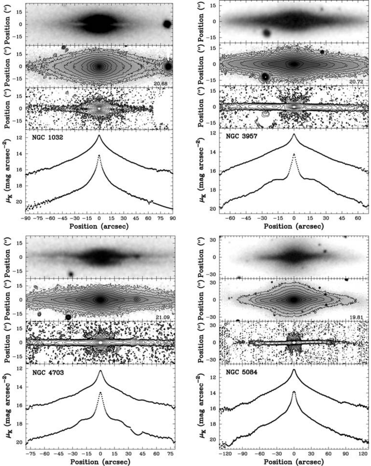
Figure 2. Same as Fig. 1 but for the control sample galaxies.
