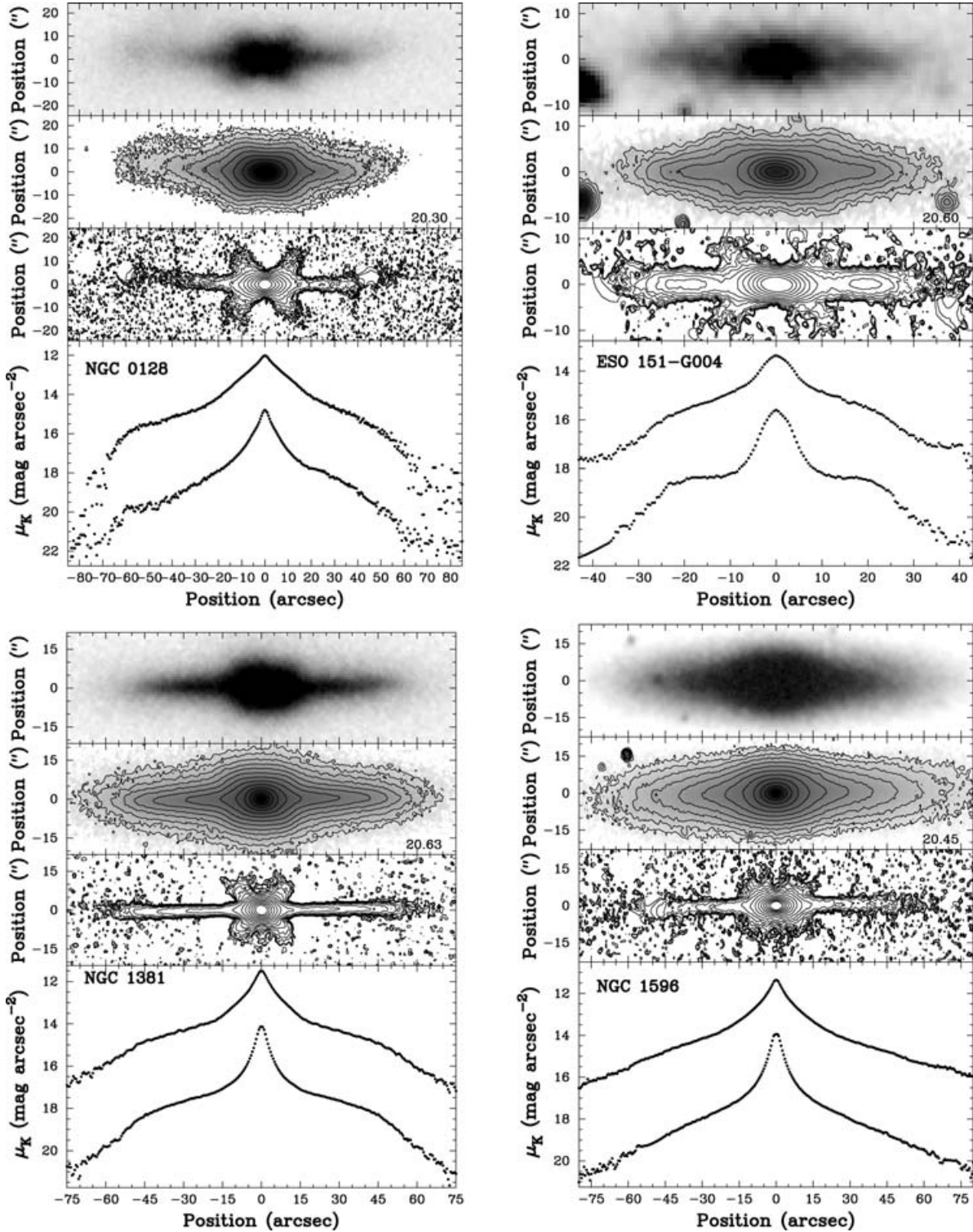
Figure 1. Images and surface brightness profiles of the galaxies with a B/PS bulge. From top to bottom, each panel shows, first, a DSS image of the galaxy, secondly, our K -band image, thirdly, an unsharp-masked K -band image, and lastly, major-axis (fainter) and summed (brighter) surface brightness profiles, all spatially registered. Contours for the K -band image are spaced by 0.5 \text{ mag arcsec}^{-2} and the faintest contour is indicated in the bottom right-hand corner of the panel.
