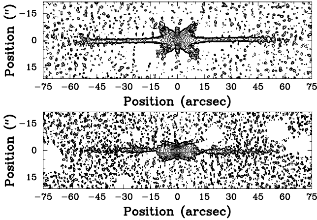
Figure 3. Kn-band images of NGC 1381 (top panel) and NGC 3203 (bottom panel) unsharp-masked on a scale of 2.5 arcsec. A long and narrow extremum is clearly seen along the minor-axis of NGC 1381, while a weaker one is observed in NGC 3203. We dub both features a minor-axis extremum. NGC 3203 also reveals weak bisymmetric elongated maxima slightly offset from the major-axis, which we associate with spiral arms in a nearly but not exactly edge-on disc. Those spiral arms are not as apparent in images unsharp-masked on larger scales.
