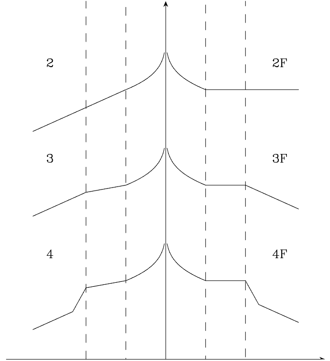
Figure 4. Cartoon description of our surface brightness profiles, as tabulated in Table 2. Two-, three-, and four-region surface brightness profiles are shown, with or without a flat intermediate region (denoted by the letter ‘F’). Note that no ‘2F’ profile was actually observed.
