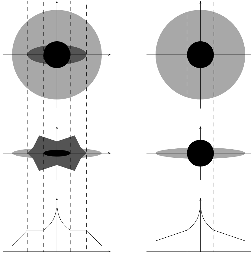
Figure 5. Cartoon description of our B/PS bulge model (left-hand panel) and the classic bulge model (right-hand panel). From top to bottom, each panel shows the face-on view of the model, the edge-on (side-on) view and the edge-on surface brightness profile, all spatially registered. Galaxies with a classic bulge are generally viewed as having both a thick and steep inner (classic bulge) component within a thin exponential disc. We suggest that galaxies with a B/PS bulge instead harbour a thin and steep inner disc component (disc-like bulge) within a thick and shallow bar (B/PS bulge), followed by an outer exponential disc.
