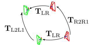
Figure 3. Rig constraint linking the euclidean transformations.
