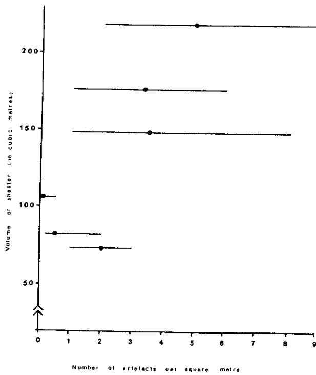
Figure 5. Plot of the relationships between floor area (a) and shelter volume (b) and average artefact density for PH shelters with and without artefacts. Also shows artefact densities in each shelter.
