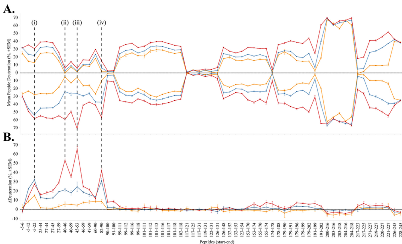
Figure 6. Comparability profiles of HDX of wild-type versus D21N 14-3-3 \zeta . A, mirror plot for visual comparison of averaged deuteration of peptides detected from wild-type 14-3-3 \zeta (above the x axis) and D21N 14-3-3 \zeta (below the x axis). Each point represents a single peptide, and the orange, blue, and red lines represent 1-, 10-, and 60-min time points of HDX, respectively. Error bars, S.E. of triplicate determinations. B, the difference plot calculated from data in A indicates that the main difference in HDX regions is in the N-terminal peptides comprising the first 90 amino acids of the protein, especially peptides from helices \alpha A, \alpha C, and \alpha D of D21N 14-3-3 \zeta . i–iv highlight the peptides showing the greatest difference in HDX between D21N and WT 14-3-3 \zeta .
