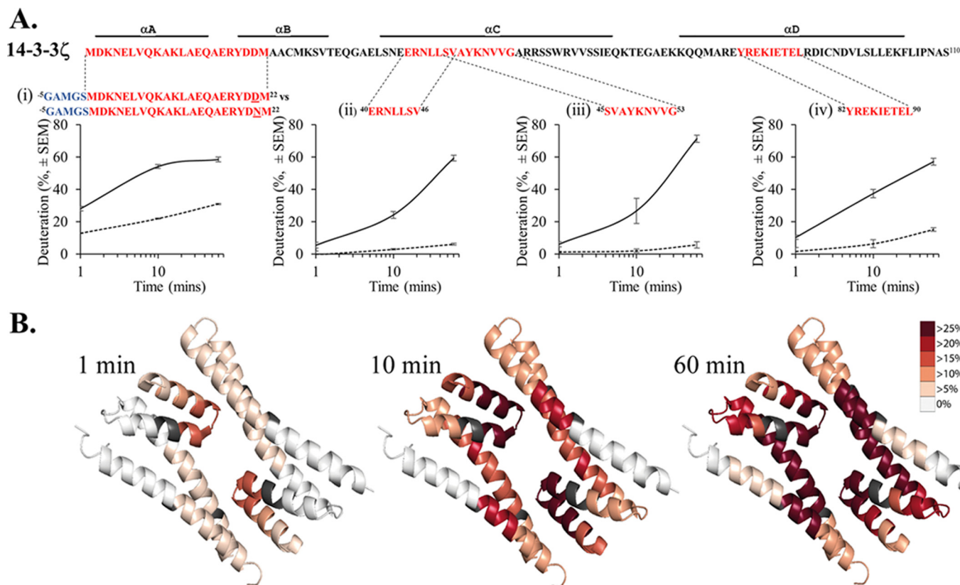
Figure 7. HDX of selected N-terminal peptides of wild-type compared with D21N 14-3-3 \zeta . A, plots show the detail of time-dependent HDX of specific peptides (i–iv), as indicated in red on the primary sequence (and highlighted in Fig. 6). Dashed lines correspond to HDX for wild-type 14-3-3 \zeta , and solid lines are HDX for D21N 14-3-3 \zeta . The average and S.E. of triplicate determinations are shown. B, the ribbon diagrams show the comparative HDX of D21N 14-3-3 \zeta compared with wild-type 14-3-3 \zeta inferred for individual residues across the dimer interface (residues 1–110) at the three different time points (1, 10, and 60 min) and expressed using heat map coloring.
