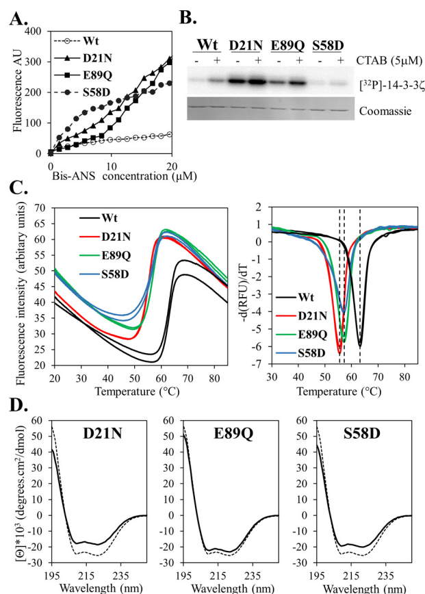
Figure 4. Single amino acid substitutions of 14-3-3ζ cause exposure of the dimer interface and affect protein thermal stability and \alpha -helical organization. A, bis-ANS fluorescence profiles for wild-type and mutant 14-3-3ζ proteins. B, in vitro phosphorylation of wild-type and mutant 14-3-3ζ proteins by PKA in the presence (+) or absence (–) of the sphingomimetic, CTAB. Reactions were separated by SDS-PAGE and analyzed for incorporation of [ ^{32}P ]ATP by autoradiography. The bottom panel shows Coomassie staining of the gel. C, protein thermal shift analysis of wild-type and mutant 14-3-3ζ proteins using SYPRO-Orange. Representative melt curves are shown in the left-hand panel, and first derivatives of those melt curves are shown in the right-hand panel. D, far-UV CD spectra for the indicated mutants (solid line) and wild-type 14-3-3ζ (dashed line). All measurements represent the average of three accumulations.
