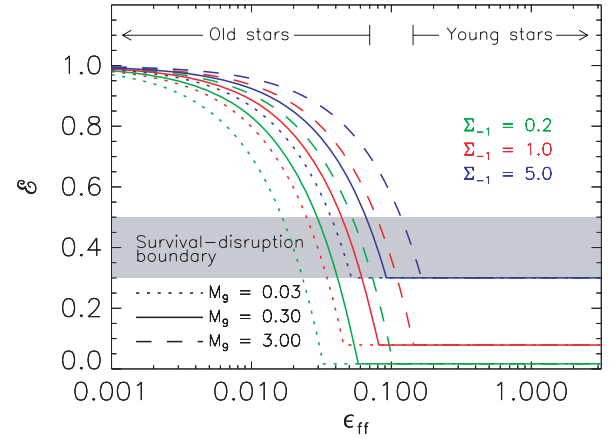
Figure 1. Final stellar fraction \mathcal{E} as a function of star formation rate efficiency \epsilon_{\text{ff}} , computed from equation (7). We show results for giant clump surface densities \Sigma_{-1} = 0.2, 1.0 and 5.0 (green, red and blue lines, as indicated), and for giant clump masses M_9 = 0.03, 0.3 and 3.0 (dotted, solid and dashed lines, as indicated). The arrows schematically indicate the region around \epsilon_{\text{ff}} = 0.1 where we change from the old stars limit (low \epsilon_{\text{ff}} ) to the young stars limit (high \epsilon_{\text{ff}} ). The grey region from \mathcal{E} = 0.3 – 0.5 indicates the rough boundary between stellar fractions \mathcal{E} \lesssim 0.3 , for which no bound stellar system will remain, and \mathcal{E} \gtrsim 0.5 , for which a majority of the stellar mass will remain bound.
