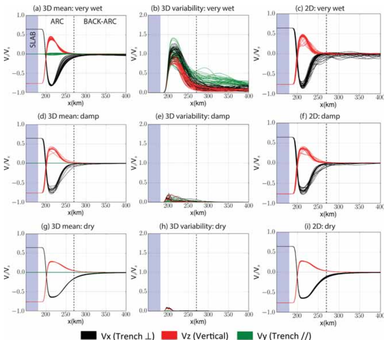
Figure 6. Individual velocity components at 100 km depth, for cases with a very-wet ( C_{OH} = 5000 \text{ H}/10^6\text{Si} ), damp ( C_{OH} = 1000 \text{ H}/10^6\text{Si} ), and dry rheology. All three cases have a 120 Myr old upper plate and V_{slab} = 5 \text{ cm/yr} . Velocities are scaled to the prescribed slab velocity, grey shades indicate the slab region, while the vertical dashed line denotes the boundary between “arc” and “back-arc” regions. Lines represent velocities every 1 Myr, from t = 25 –50 Myr. Figures 6a, 6d, 6g display trench-parallel averages of trench-perpendicular, trench-parallel and vertical velocities, while Figures 6b, 6e, 6h display the trench-parallel variability ( |V_{max} - V_{min}| ) around these 3-D averages. Figures 6c, 6f, 6i show the same lines for corresponding 2-D models from Le Voci et al. [2014].
