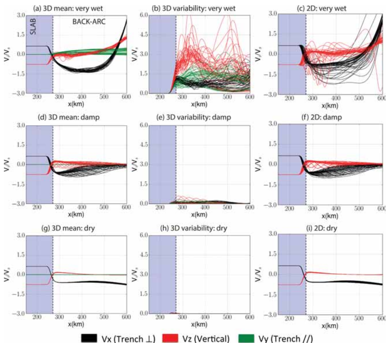
Figure 7. As in Figure 6, but at 150 km depth, illustrating individual velocity components beneath the back arc.
