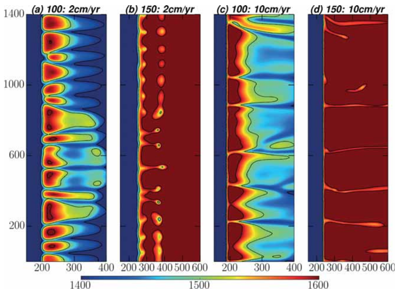
Figure 10. Temperature cross sections at (a,c) 100 and (b,d) 150 km depth, respectively, for very-wet ( C_{OH} = 5000 \text{ H}/10^6 \text{ Si} ) cases with a 120 Myr old upper plate and a subduction velocity of: (a,b) 2 cm/yr; (c–d) 10 cm/yr. All slices shown are at t = 45 \text{ Myr} . The corresponding 5 cm/yr subduction velocity case is shown in Figure 3.
