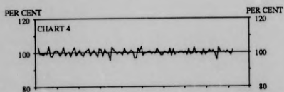
RESIDUAL/IRREGULAR VARIATION
