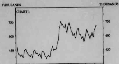
ORIGINAL SERIES
