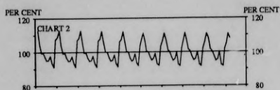
SEASONAL VARIATION
