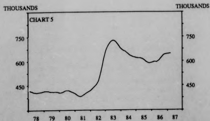
TREND SERIES
