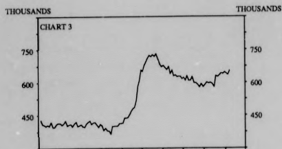
ADJUSTED SERIES
