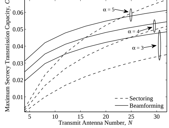
Fig. 6. The maximum secrecy transmission capacity of the sectoring and beamforming schemes versus the number of transmit antennas. Results are shown for the case where \lambda_l = 0.01 , \lambda_e = 0.001 , r = 1 , \sigma = 0.1 and \epsilon = 0.01 .
