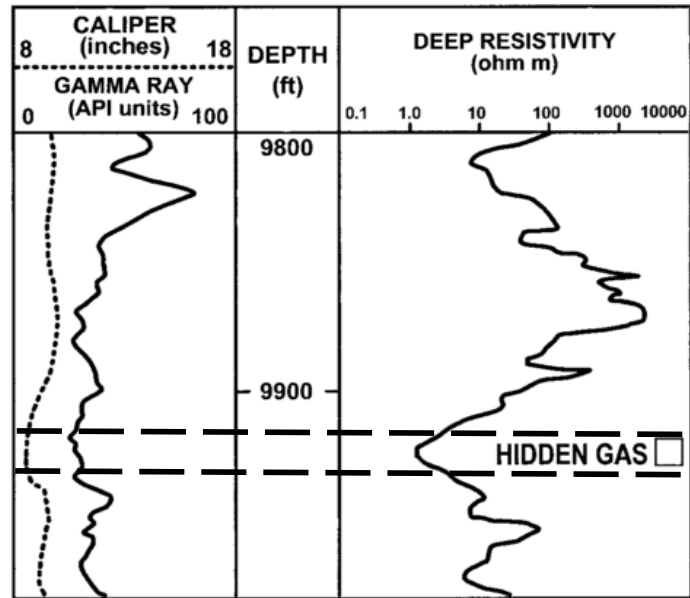
Figure 2.3: A wireline log from a microporous reservoir in the Rodessa Limestone, Texas. The gas interval has low resistivity due to immobile water in intragranular pores (Worthington, 2000). Due to its low resistivity, the gas interval was interpreted as water.
