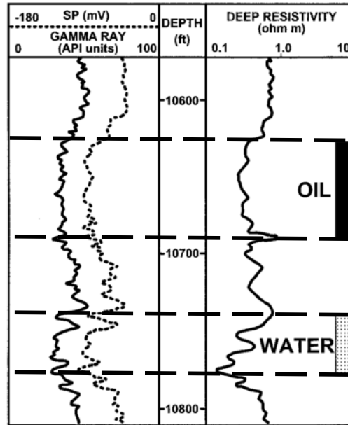
Figure 2.2: A wireline log from a clean and fine sand reservoir in Tertiary Sands, Gulf of Mexico. High capillarity in the fine-grain sediments causes low resistivity and low contrast issues between the water and oil intervals (Worthington, 2000).
