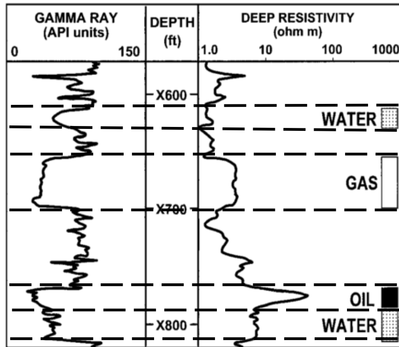
Figure 2.4: Wireline log from a superficially microporous reservoir in the Attaka field, Indonesia. The ‘low resistivity’ upper section gas interval is microporous compared to the ‘high resistivity’ oil interval in the bottom (Worthington, 2000).
