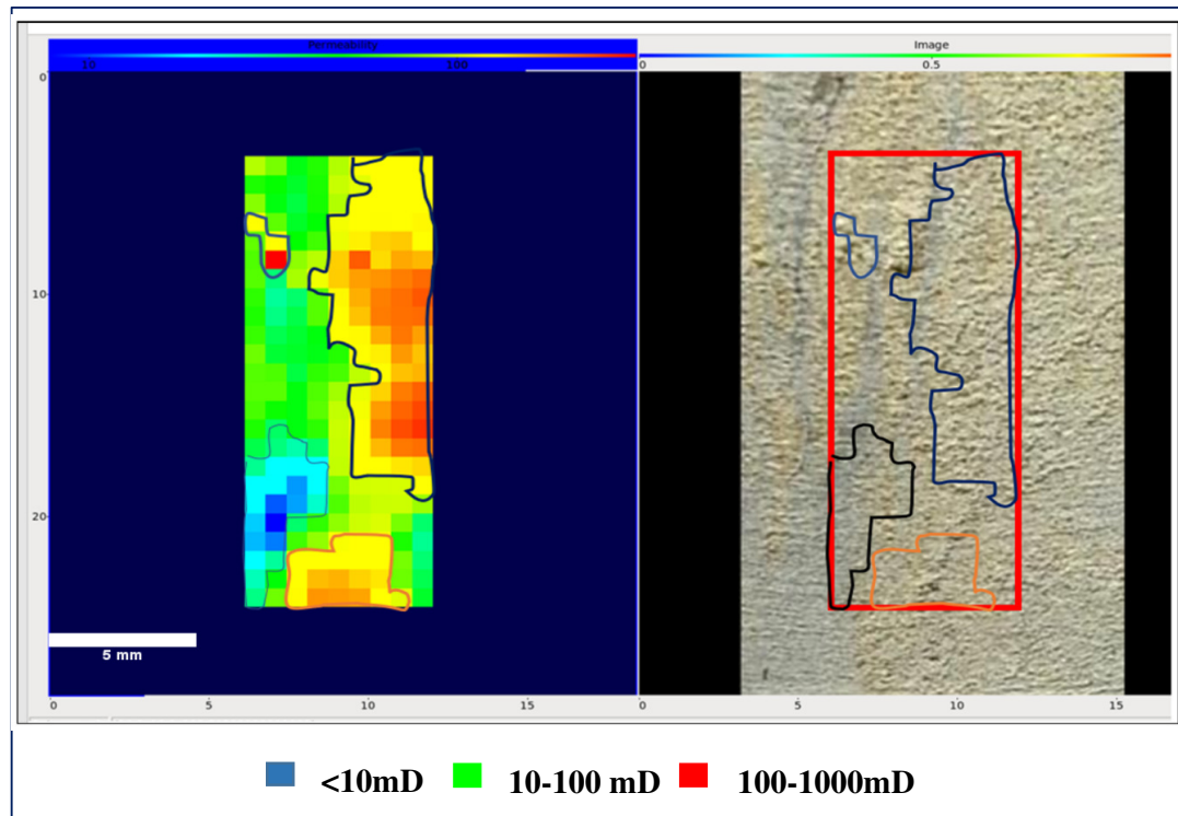
Figure 8.58: Permeability on the surface of the core plug 64 from the NER Gas Probe. The blue/green areas are low permeability mudstone dominated regions that are below 100 mD while the yellow/orange areas and permeable sandstone regions that are between 100-1000 mD.
