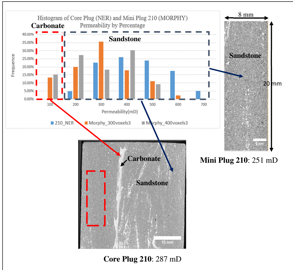
Figure 8.67: Histogram of Permeability results from using MORPHY and the NER Gas Probe of Sample 210. There is some degree inconsistency between the MORPHY computed permeabilities and the NER gas probe measured permeabilities though many of the NER gas probe results are on the higher side. The NER gas probe averaged permeability is at least 60% higher than the averaged computed permeability.
