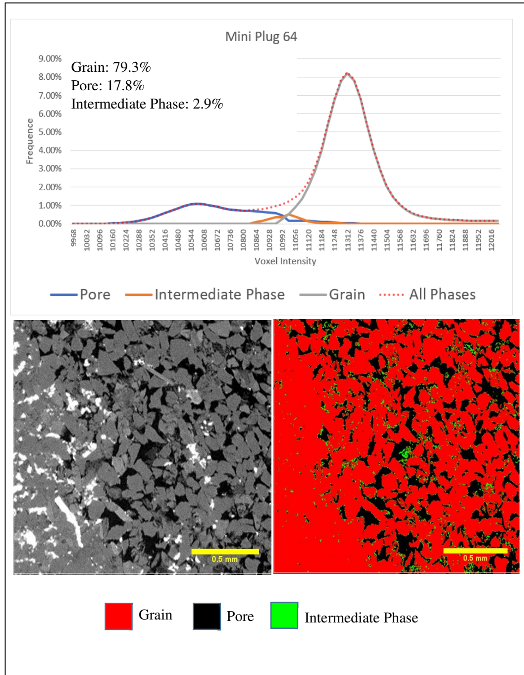
Figure 8.1: Top: Voxel Intensity Histograms of mini plug 64. Bottom: Greyscale and segmented images the mini plug 64
