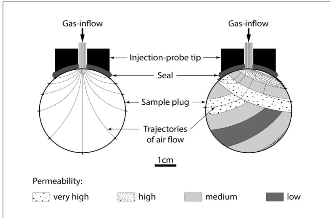
Figure 8.60: Gas-flow trajectories for (a) homogeneous samples and (b) heterogeneous samples. Such structures strongly affect flow geometry by inducing preferential flow, which creates issues in determining volume and area represented by surface permeability measurements.
