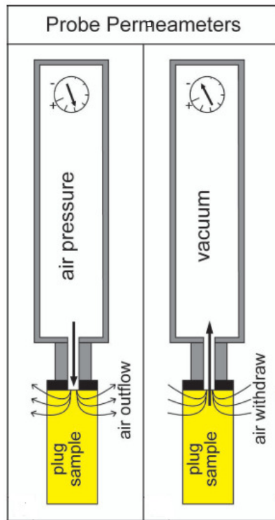
Figure 4.6: Permeability measurement using a New England Research mini-permeameter using air injection principle (Filomena et al., 2013)
