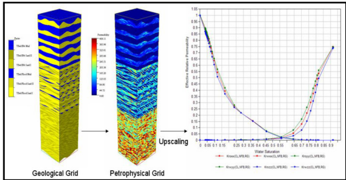
Figure 2.9: Metre scale bedform model of a wellbore above shows the upscaling process from the wellbore scale to the reservoir scale (Alam, 2012).
