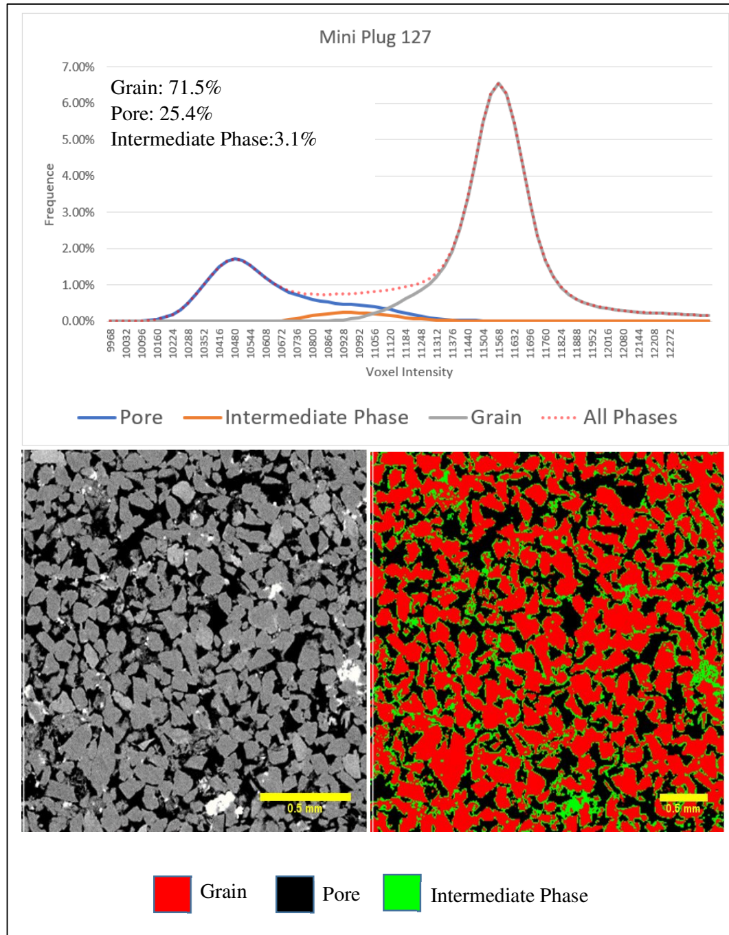
Figure 8.2: Top: Voxel Intensity Histograms of mini plug 127. Bottom: Greyscale and segmented images the mini plug 127.
