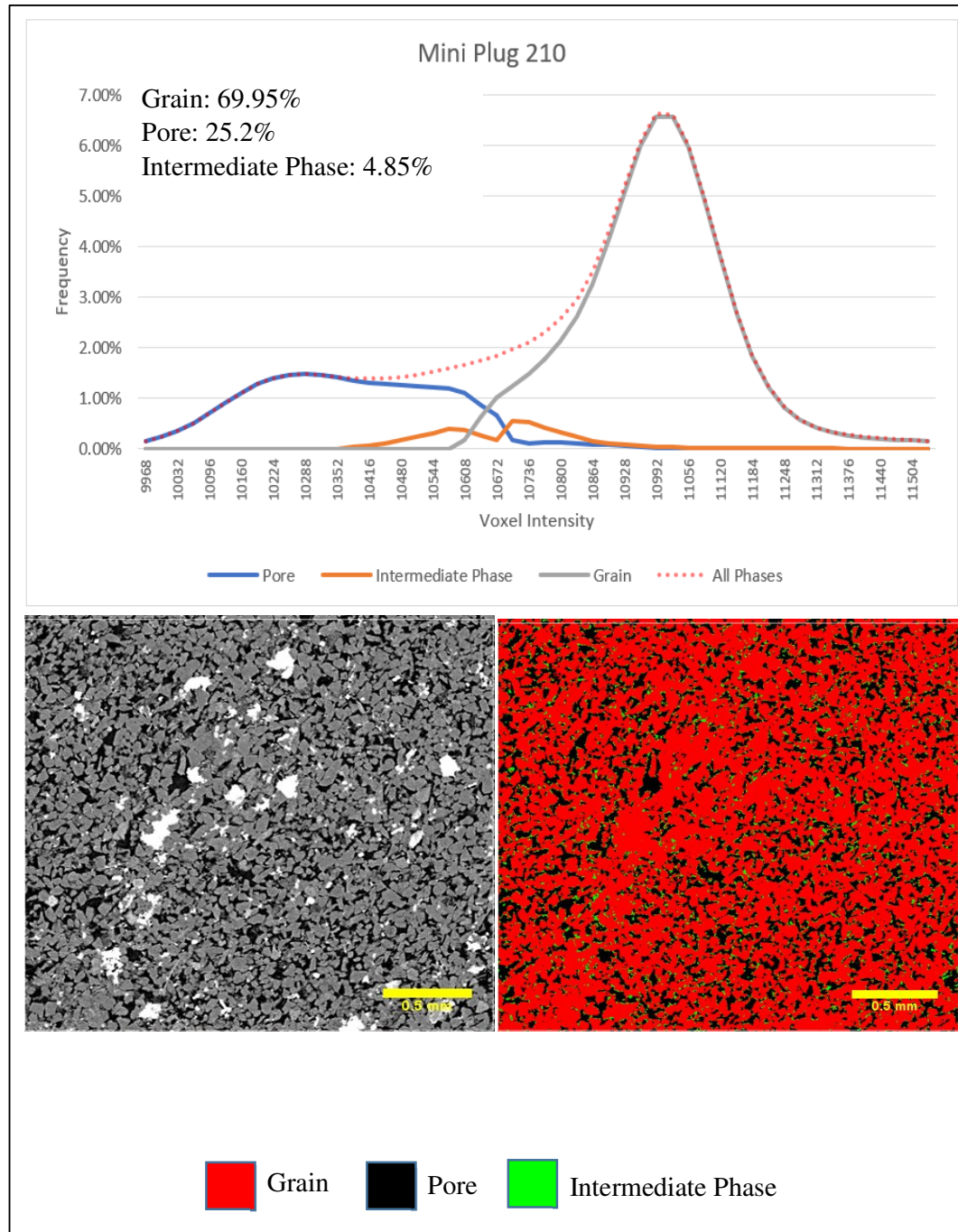
Figure 8.5: Top: Voxel Intensity Histograms of mini plug 210. Bottom: Greyscale and segmented images the mini plug 210.
