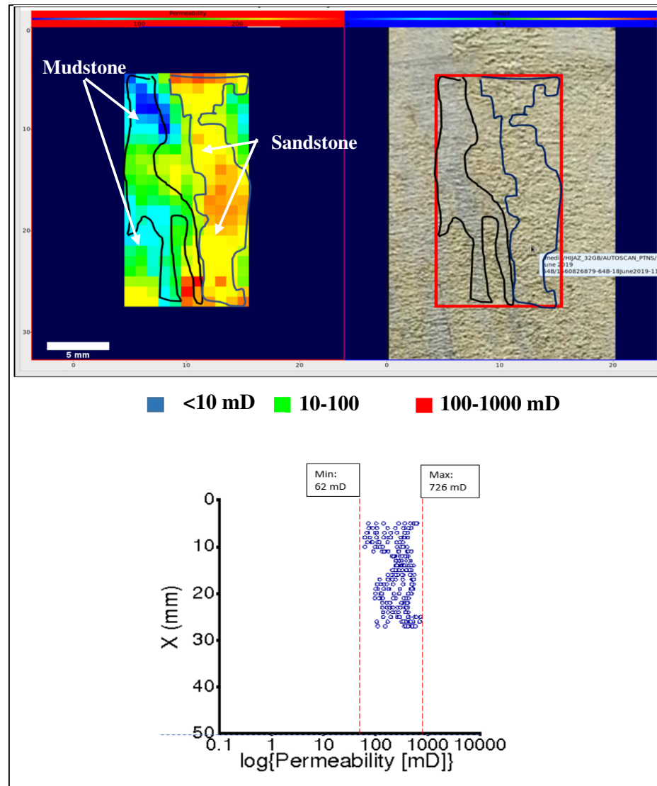
Figure 8.28: Permeability map of core plug 64, side B.
