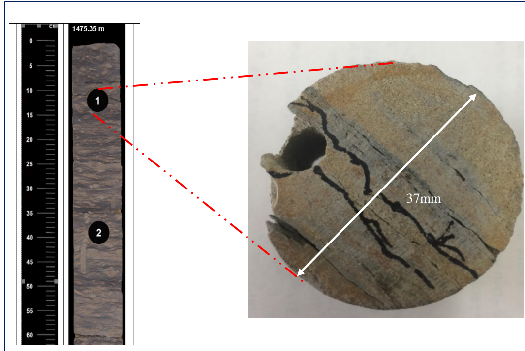
Figure 8.52: A view of one of the faces of core plug 64 (right), indicating distinct layers of dark coloured mudstone and light-coloured sandstone. The numbers in the core slab on the left indicate the order of the core plug. The hole on the core plug in the location from where we extracted a 6 mm mini-plug.
