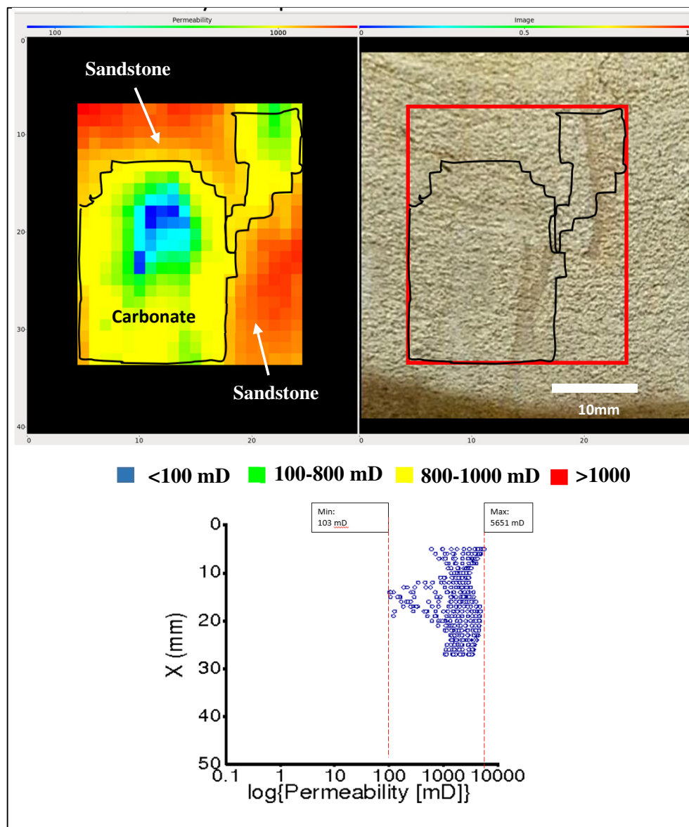
Figure 8.30: Permeability map of core plug 127, side B.
