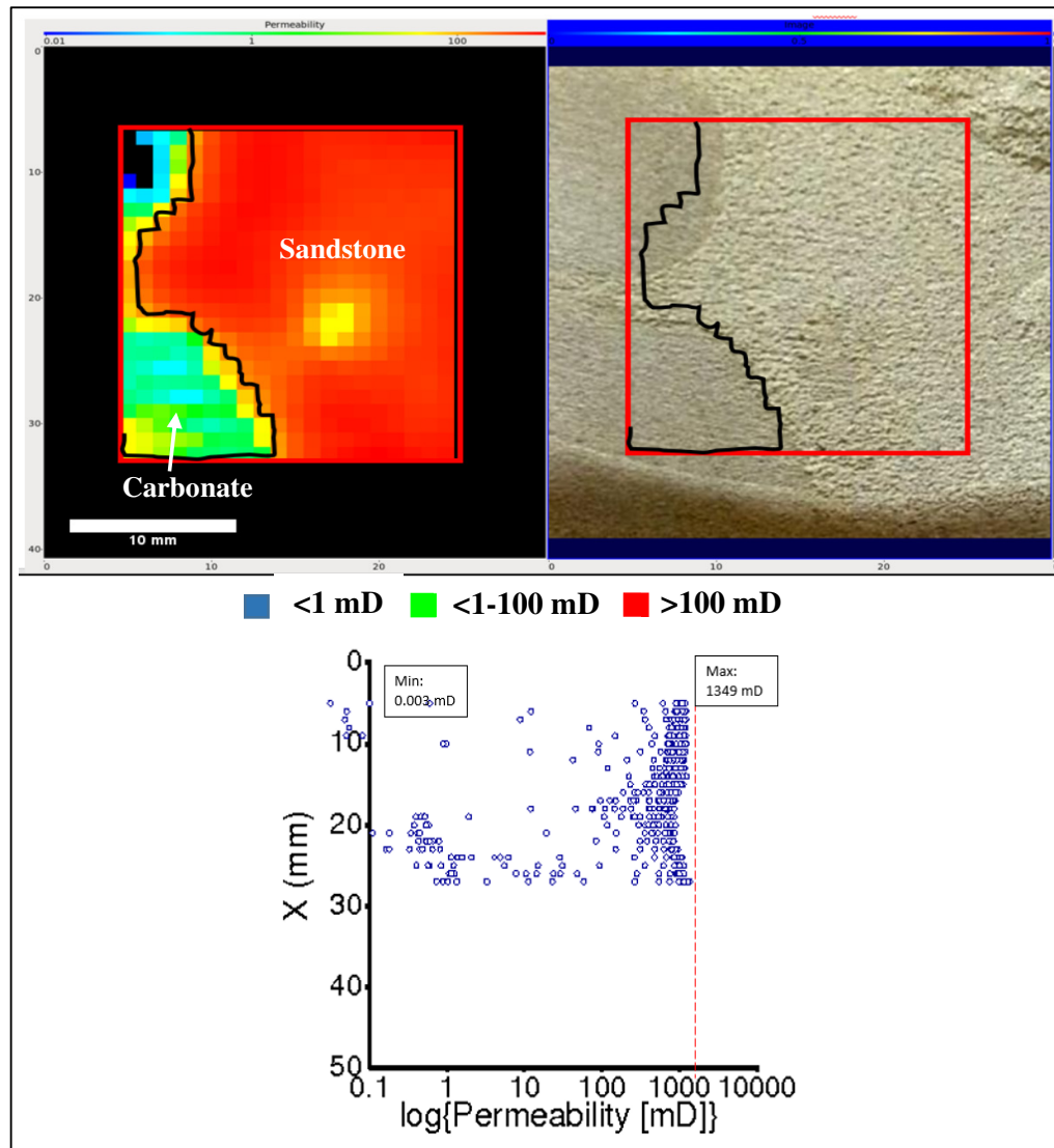
Figure 8.32: Permeability map of core plug 148, side B.
