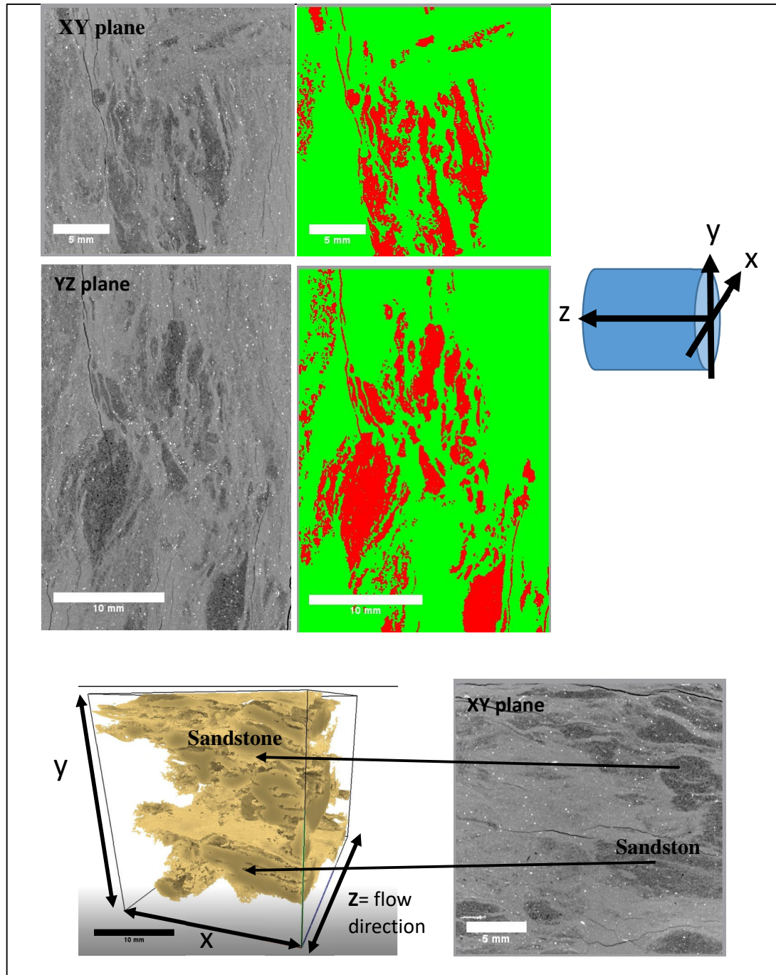
Figure 8.71: Top and Middle Images are greyscaled images and segmented images of core plug 245. The left bottom left image is a rendered 3D volume of core plug 245, showing the sandstone phase tagged in yellow. The segmented mudstone in core plug 245 occupies 17.9% of its volume.
