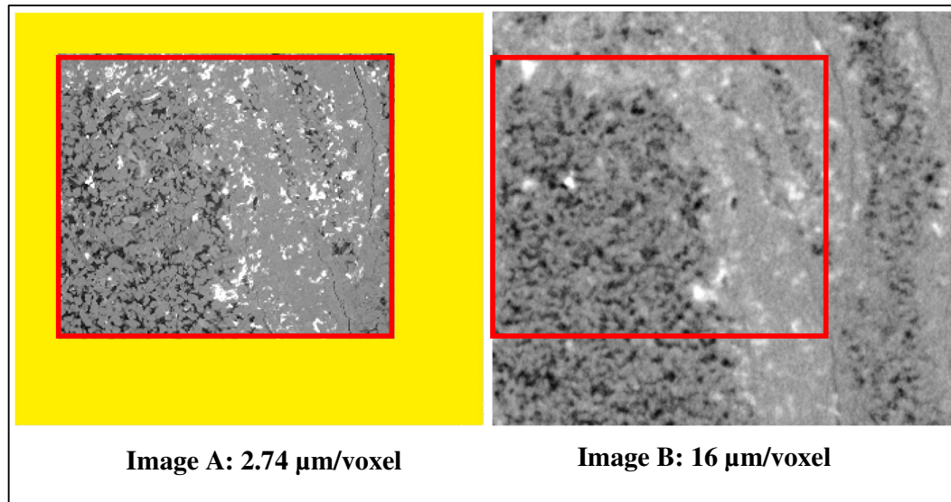
Figure 8.12: Two aligned images from the mini plug (A) and core plug (B) after application of Registration 3D to 3D volume. The mini plug image resolution (left) is reduced from 2.74 microns/voxels to 16 micron/voxels. The red square in image B corresponds to image A.
