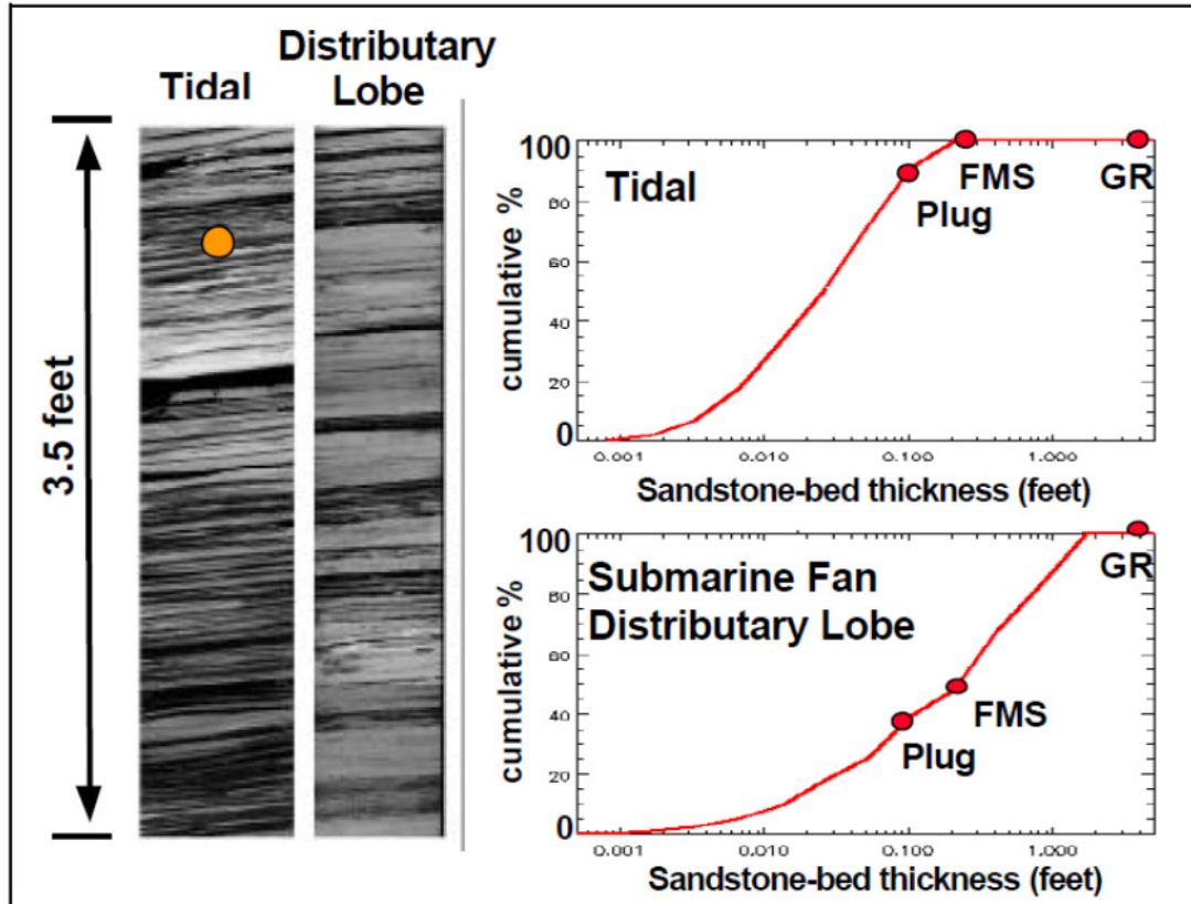
Figure 2.6: Core images from two thin-bed reservoirs and their bed thickness distribution plots showing the approximate resolution of core plugs and Gamma Ray (GR) and borehole image logs (Passey et al., 2006)
