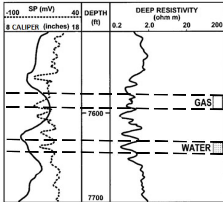
Figure 2.1: An example of a low resistivity reservoir in the Eutaw play, Mississippi. Conductive minerals cause poor resistivity contrast between the gas and water-bearing intervals (Worthington, 2000).
