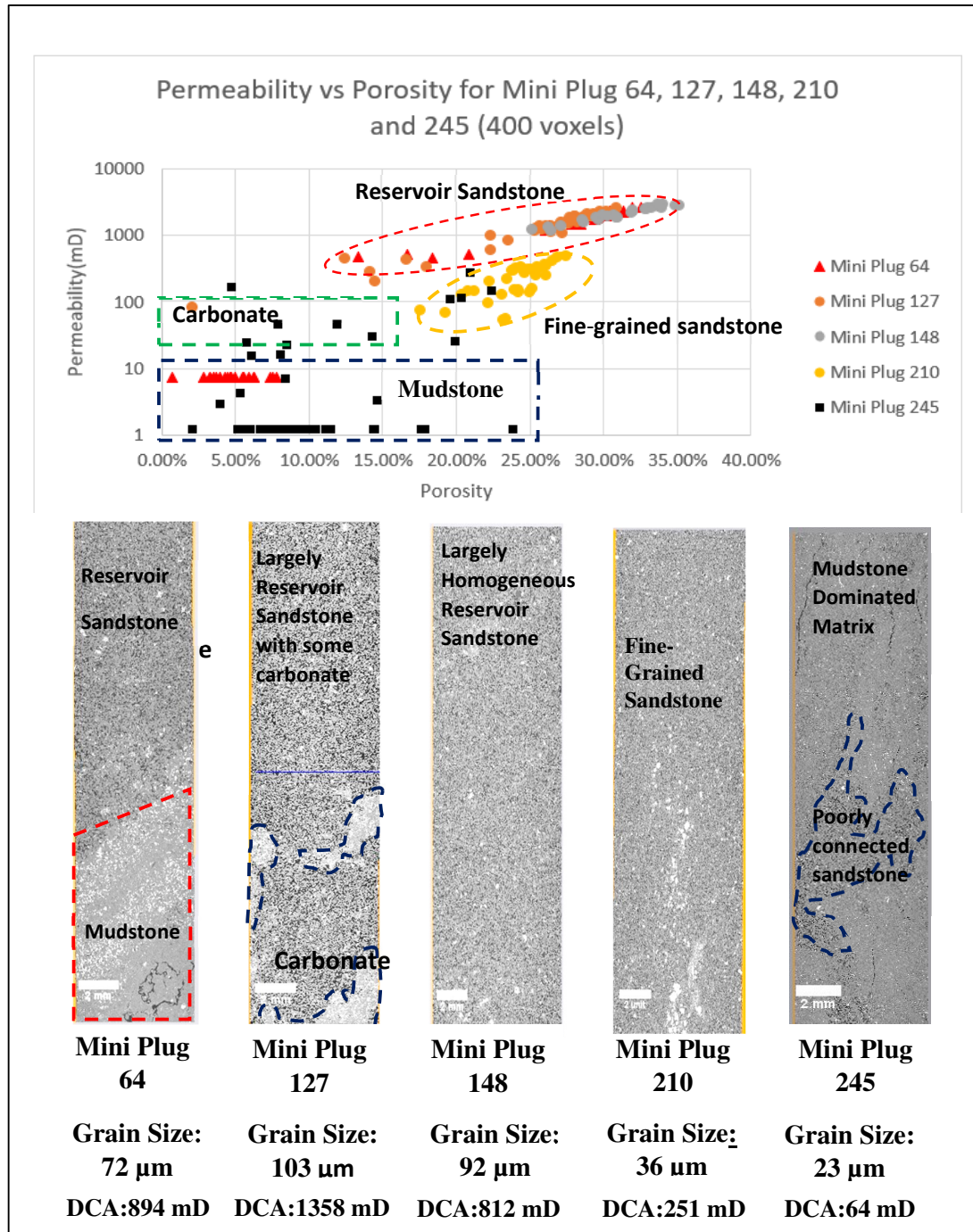
Figure 8.76: Permeability vs. Porosity graph for the five mini plugs. The heterogeneity and median grain size of contributed to varying mini-plug permeability.
