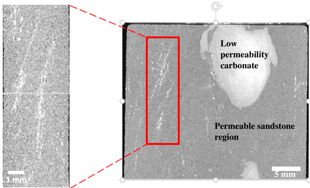
Figure 8.19: Approximated location of mini plug 148 in relative to the volume of core plug 148. We noted there is a white high attenuation region that consists of carbonates that have different permeability compared to the rest of the sandstone region or act a barrier to flow, resulting in lower effective permeability of the core plug.
