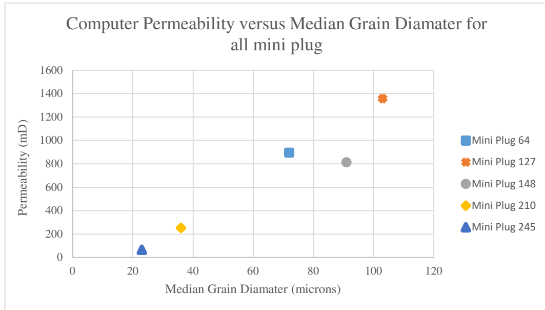
Figure 8.9: The computed permeability of the mini-plugs using digital core analysis for 300 voxels 3 sub-volume sizes versus the median grain diameter of the mini-plugs. The results showed that permeability increases with median grain diameter.
