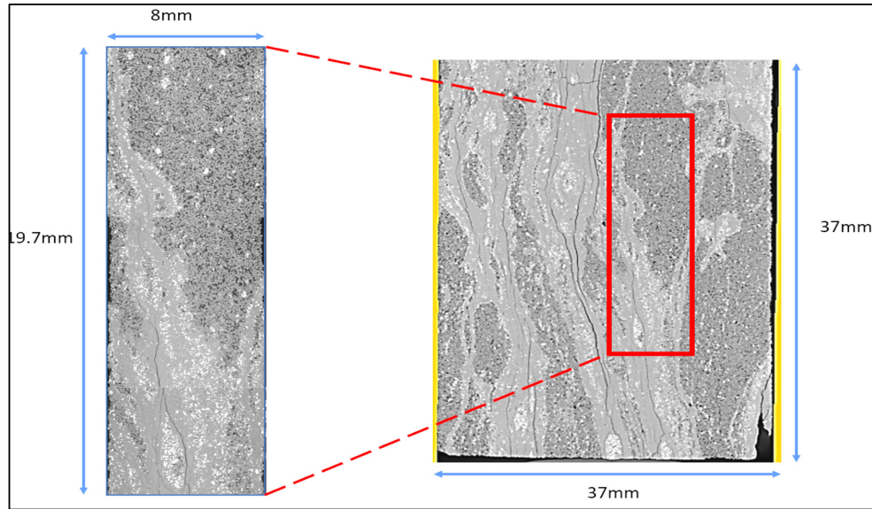
Figure 8.14: Registration of the mini plug to its original location on core plug 64. We observed that sandstone dominates a significant amount of the core plug.
