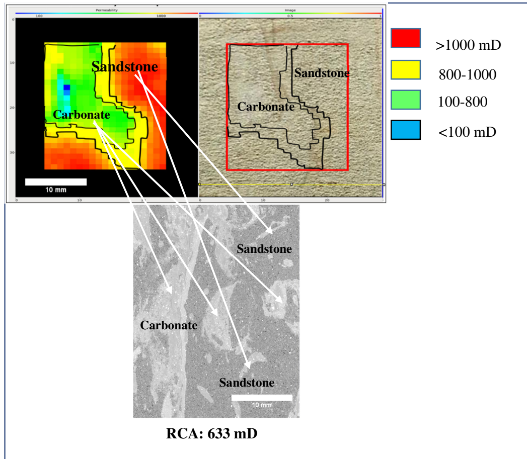
Figure 8.51: Top image: Permeability map on the surface of the core plug 127 from the NER permeameter. The red regions are high permeability sandstone, while the green, yellow and blue regions are carbonate minerals with permeability below 1000 mD. Bottom image: XMCT image of core plug 127 with carbonate laminated correlated to the low permeability regions on the permeability map.
