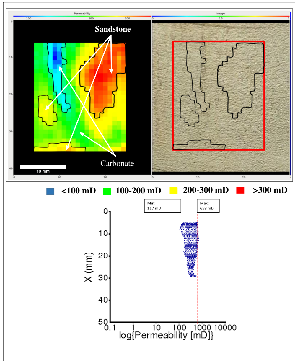
Figure 8.34: Permeability map of core plug 210, side B.
