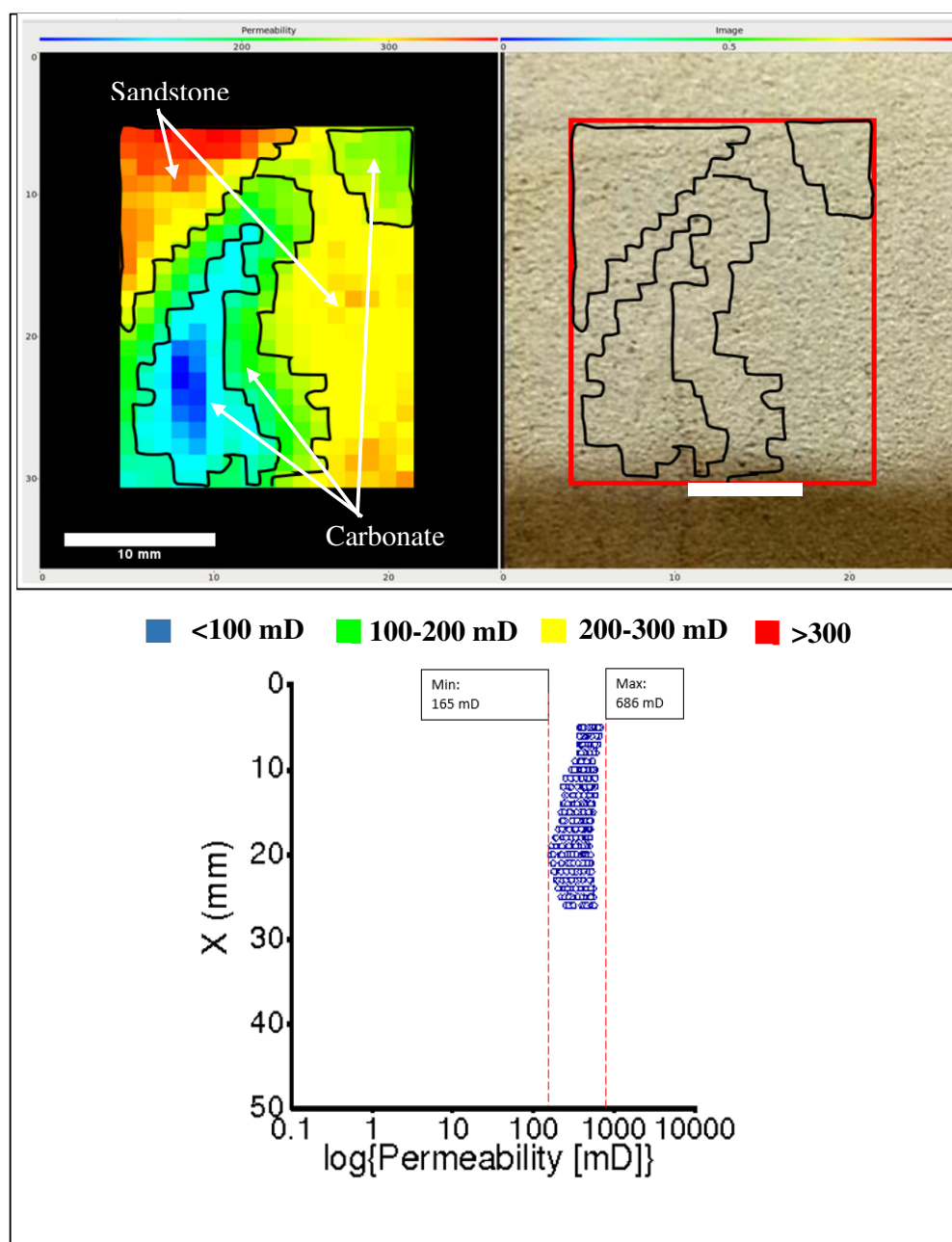
Figure 8.33: Permeability map of core plug 210, side A.
