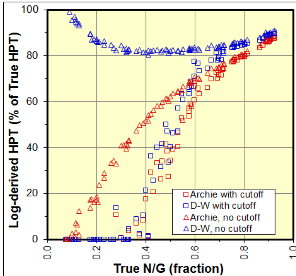
Figure 2.8: Log derived HPT for 130 simulated thin-bed reservoirs
