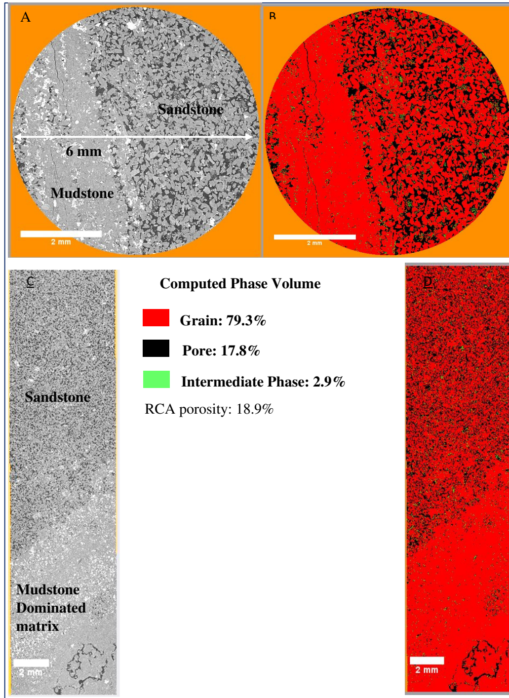
Figure 8.55: Images of mini plug 64. Greyscale and segmented images of Mini Plug 64.
