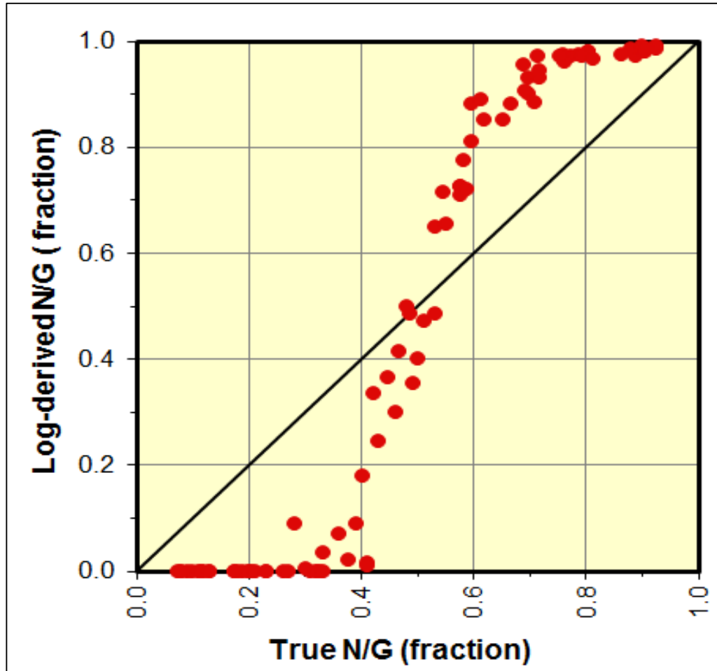
Figure 2.7: Actual Gamma Ray and Well log derived net sand fraction or Net to Gross (N/G) for a 130 feet thin bed-bed reservoir simulation (Passey et al., 2006). This figure shows that log derived net-to-gross is lower compared to actual net-to-gross.
