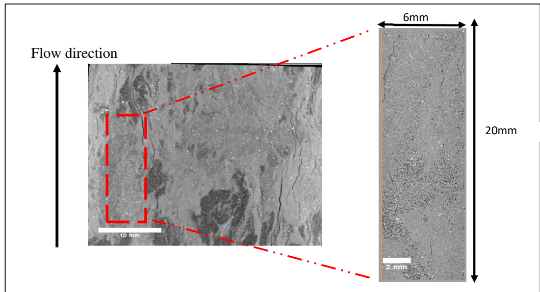
Figure 8.70: Left: Low-resolution image (37 microns/voxel) and Right: High-Resolution image (3.76 microns/voxel) tomograms of Sample 245.
