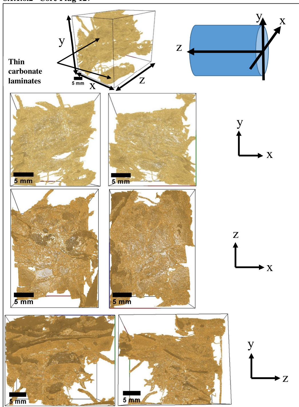
Figure 8.23: 3D volume images of core plug 127 showing the segmented carbonate laminates that could potentially block fluid flow.
