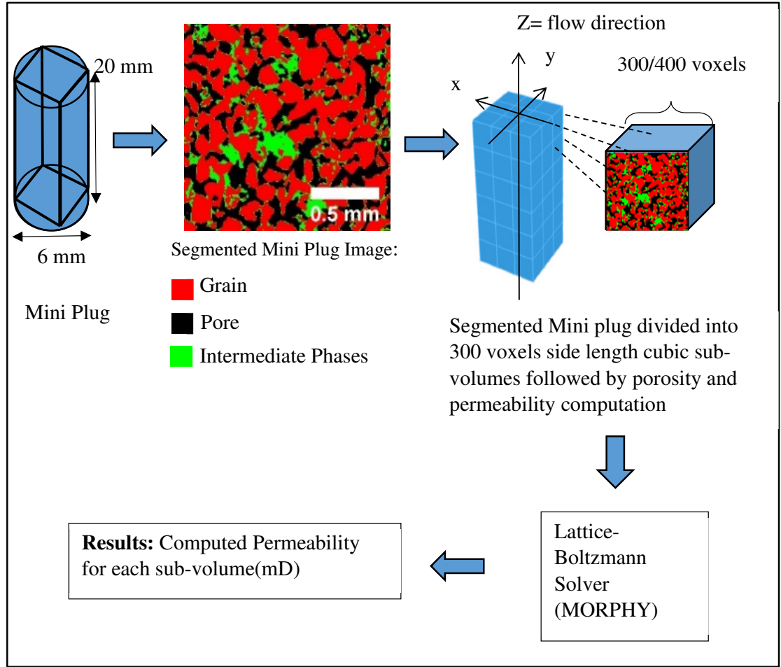
Figure 4.4: Workflow for computing permeability and porosity using a Lattice-Boltzmann method. The direction of simulated flow in the z-direction, which is the same as the direction of the injected fluid in core plug analysis.
