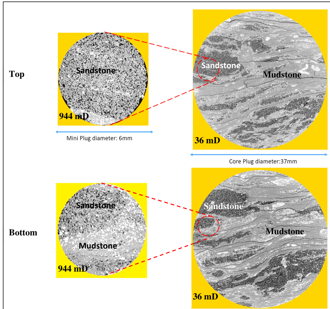
Figure 8.13: We show mini plug 64(left) relative to its original location in the core plug 64 (right). Large sections of the mini-plugs are made up of sandstone.
