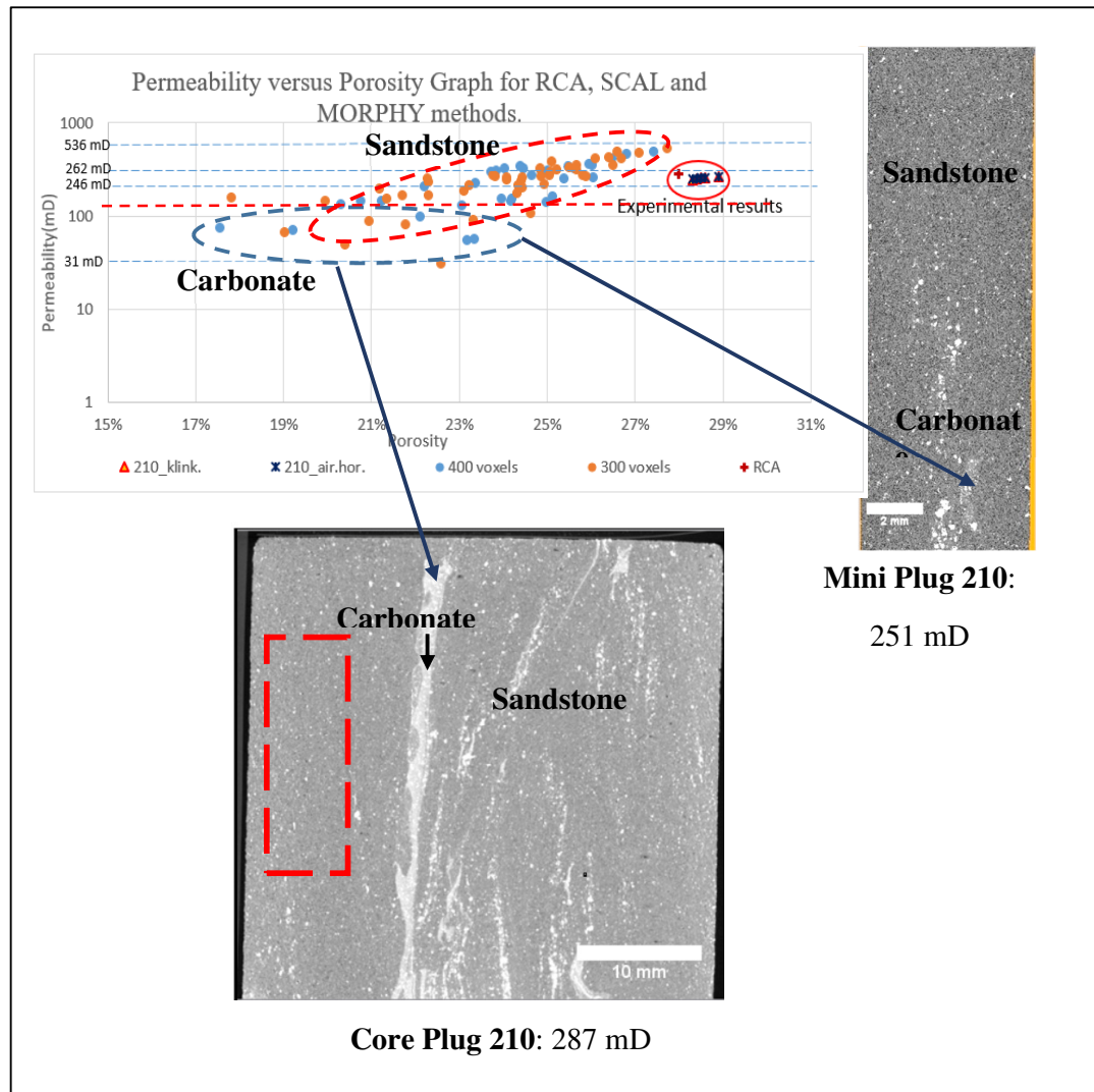
Figure 8.65: Permeability versus Porosity graph of Routine Core (RCA), Special Core Analysis (SCAL), and MORPHY (for 300 voxels and 400 voxels sub-volumes). The Klinkenberg horizontal permeability and horizontal air permeability are the experimental
