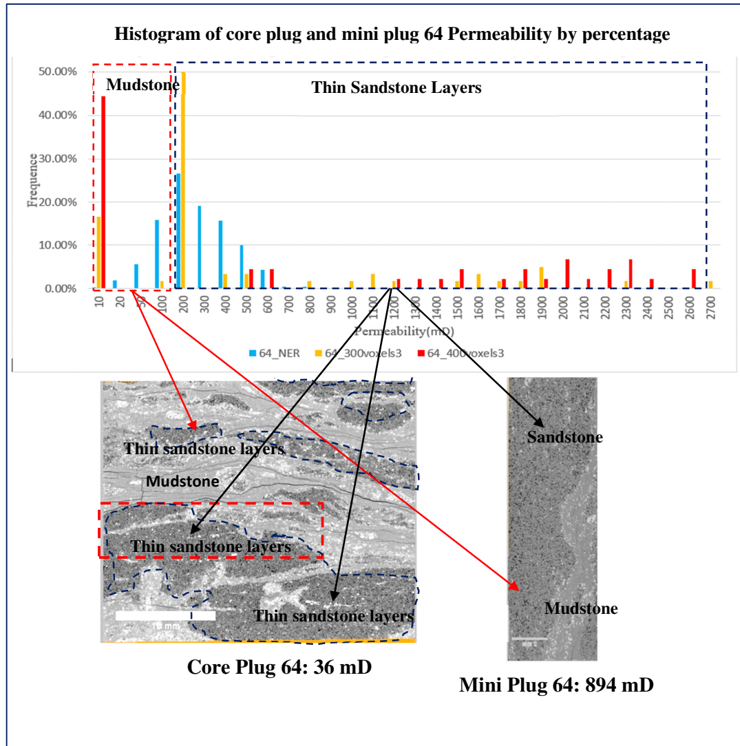
Figure 8.57: Histogram of Permeability results from using MORPHY and the NER Gas Probe. The MORPHY results represent mini plug 64, while the NER results are from core plug 64.
