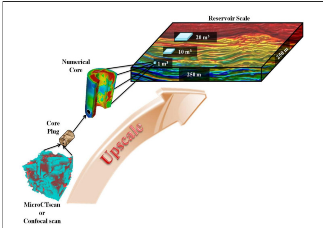
Figure 9.1: Upscaling workflow diagram in heterogeneous rocks. A grid block used in a reservoir simulator is 250 x 250 x 1m in size (right). Borehole-scale numerical cores represent rock volumes on the cubic-meter scale (centre). Core plugs, X-Ray Micro-CT scans, and confocal scans represent even smaller volumes (left). The question is, how representative are these small volumes when compared to coarse grid blocks or full fields? (Hurley et al., 2012)
