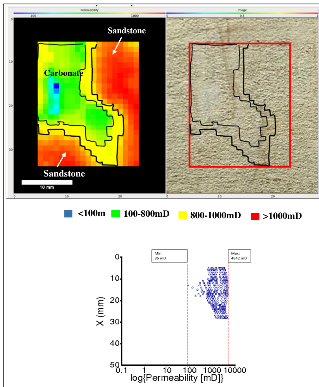
Figure 8.29: Permeability map of core plug 127, side A.
