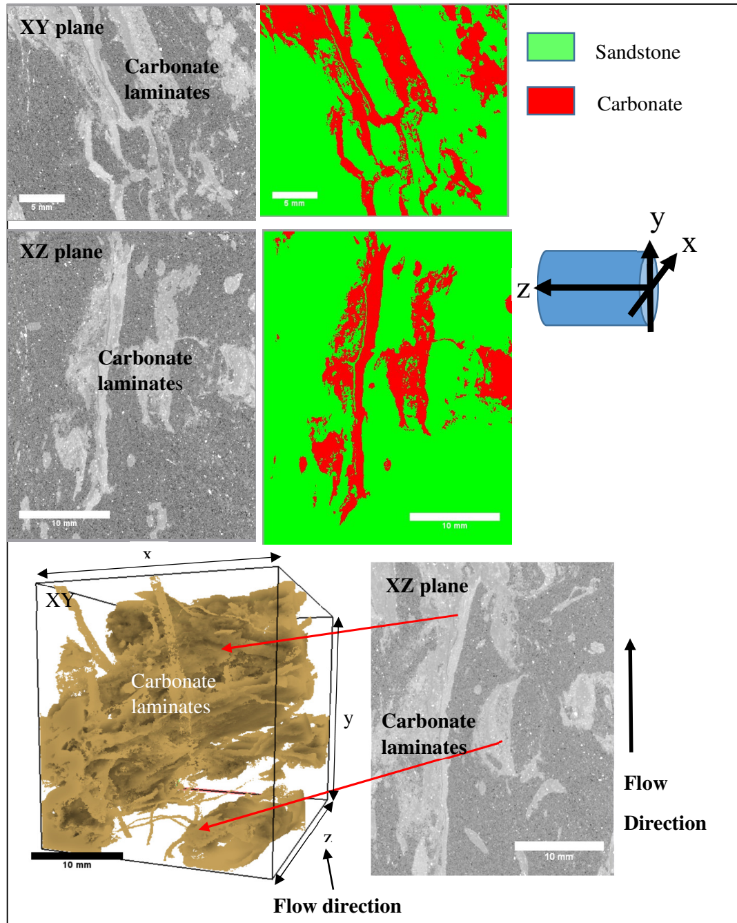
Figure 8.46: Top and Middle Images are greyscaled images and segmented images of core plug 127. The left bottom left image is a rendered 3D volume of core plug 127 showing the calcium carbonate phase tagged in yellow. The segmented calcium carbonate in core plug 127 occupies 16% of its volume. The fluid was injected in the z-direction in the experimental core plug analysis.
