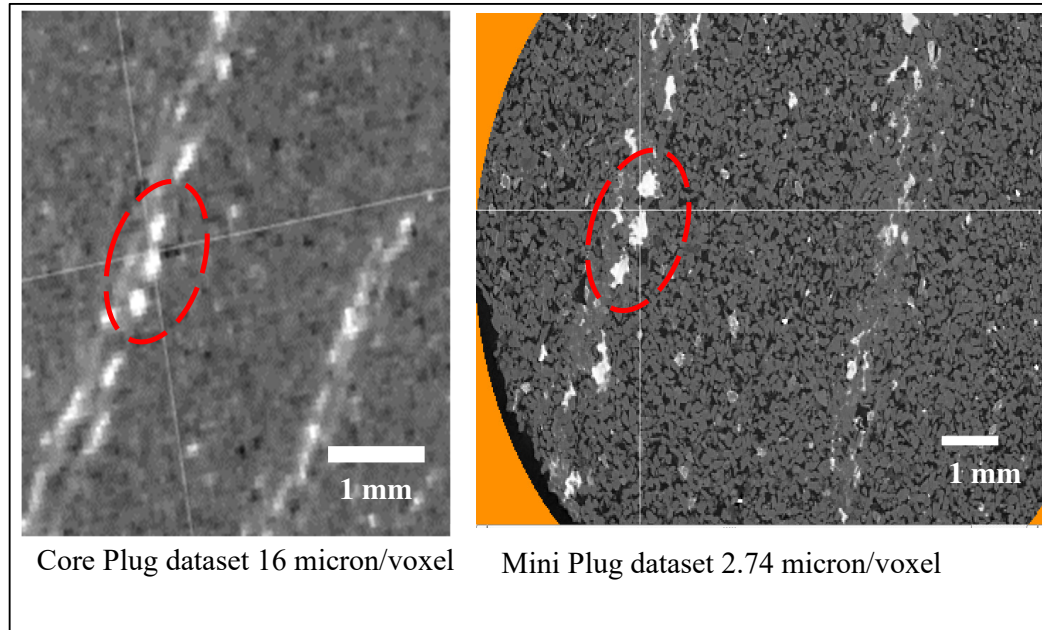
Figure 8.17: We identified Similar features in the mini plug and core plug datasets (in red circles) for ‘3D to 3D’ Image registration process.
