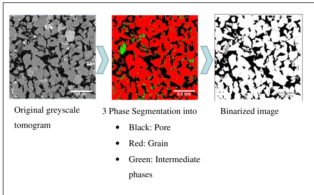
Figure 4.3: Segmented XMCT image of mini plugs using MANGO. The resolution is 2.74 microns/voxel. (Images were taken at Australian National University CTLab and processed using the MANGO software)
