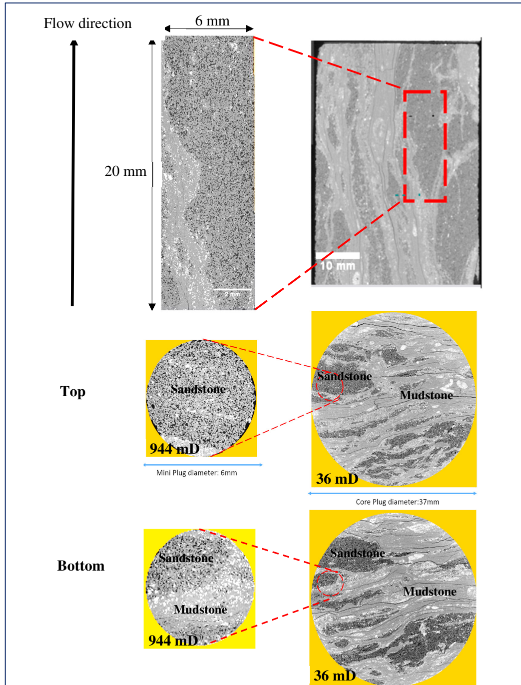
Figure 8.53: Left: High resolution (2.74 microns/voxel) and Right: Low Resolution (16.3 microns/voxel) tomograms of Sample 64 indicating the location of mini plug 64 in core plug 64.
