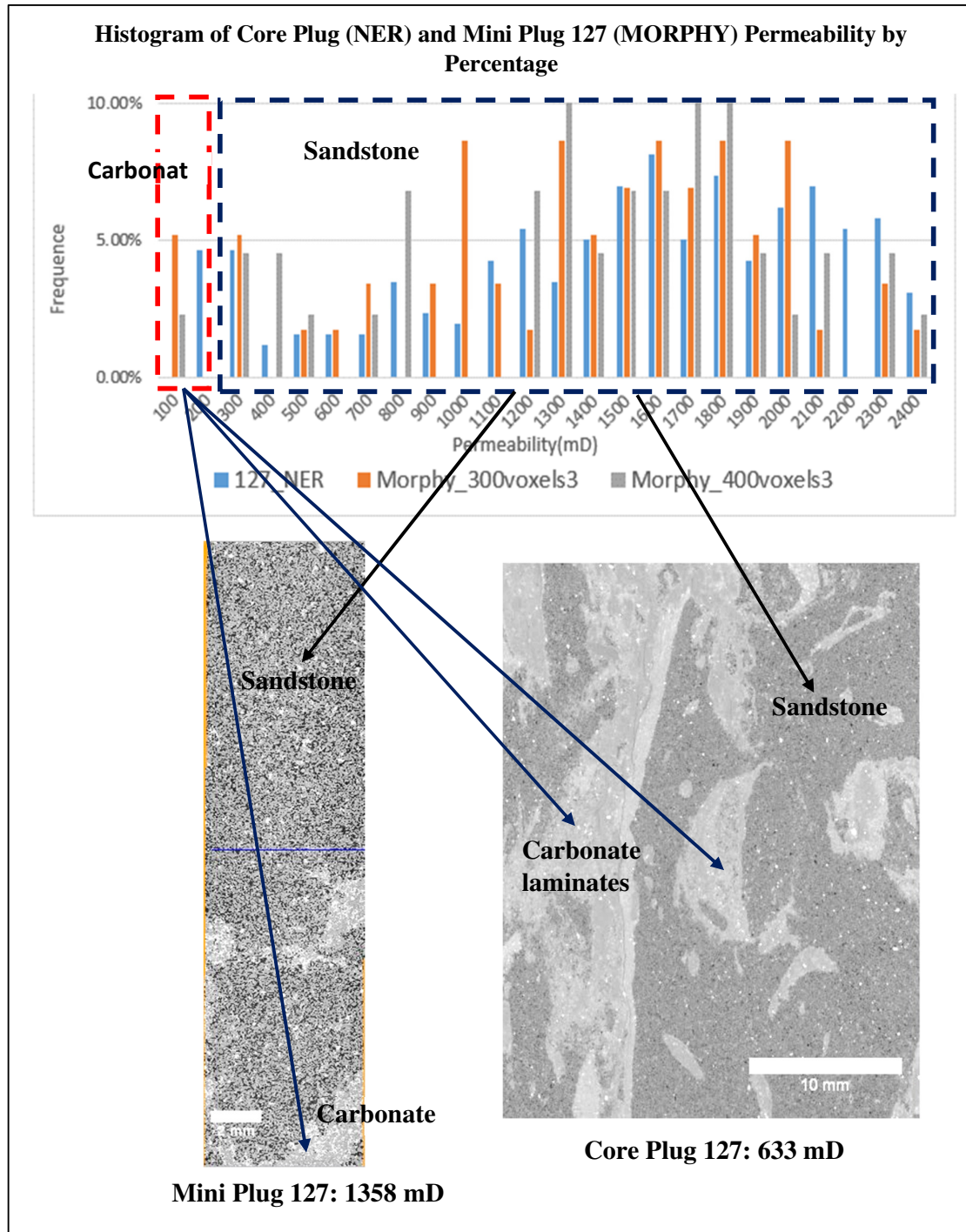
Figure 8.50: Histogram of Permeability results from using MORPHY and the NER Permeability Gas Probe. Images in the bottom are the XMCT images of mini plug 127 and core plug 127. We correlated the low permeability results on the histogram below 100 mD to the carbonate minerals in core plug 127.
