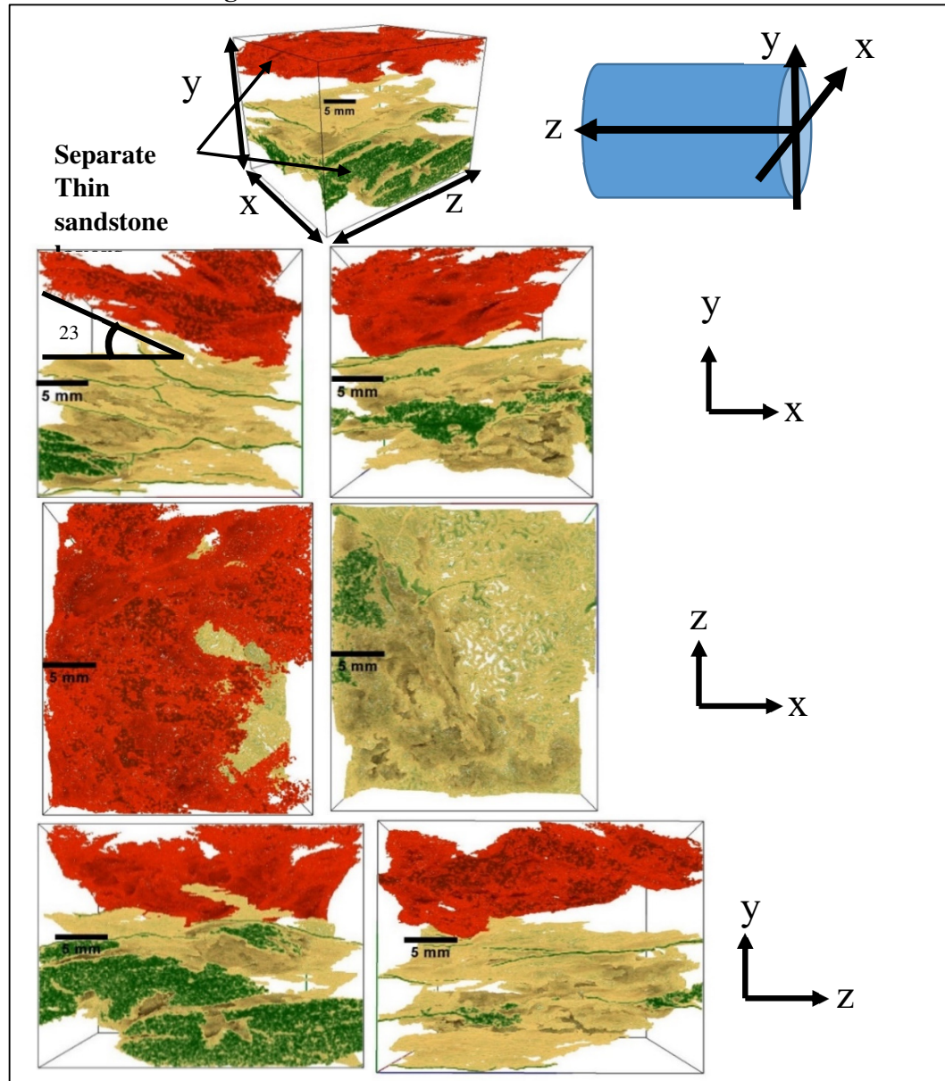
Figure 8.22: 3D volume images of core plug 64, showing two sandstone layers within the core plug. The red phase represents a very thin upper sand layer that is about 1 mm thick while the lower green phase layers consist of several 1 mm to 5 mm sandstone layers connected. The different colors of the sand layers indicate that they are not connected.
