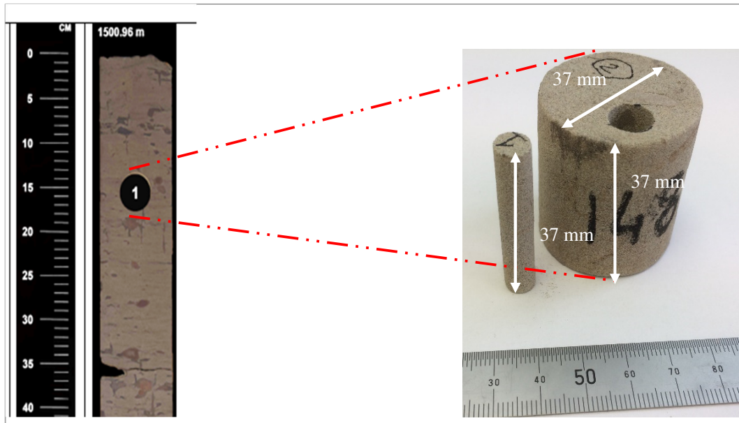
Figure 8.37: A view of core plug 148 and the core slab that indicates light-colored sandstone.
