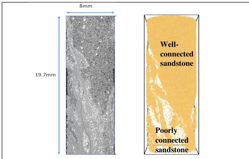
Figure 8.15: The left image is the greyscale tomogram of mini plug 64, while the right image is a corresponding Drishti rendering of the sandstone phase. We observed that the sandstone has good connectivity and spans the mini plug in the axial direction but thins out at the bottom.
