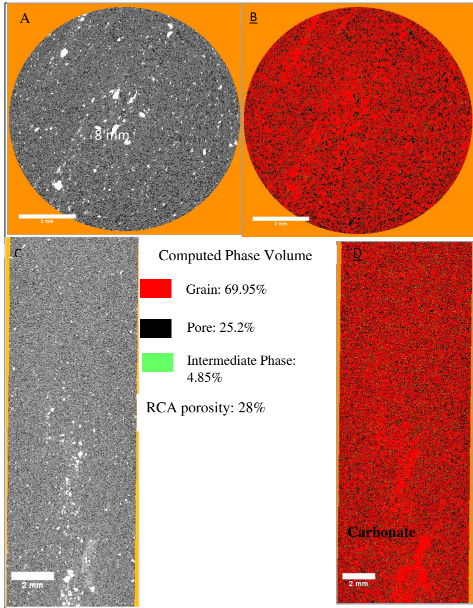
Figure 8.64: Image A and C: Greyscale image of Mini Plug 210. Image B and D: Segmented images of Mini Plug 210. The sandstone grains in mini plug 210 are very fine and well connected with little signs of heterogeneity.
