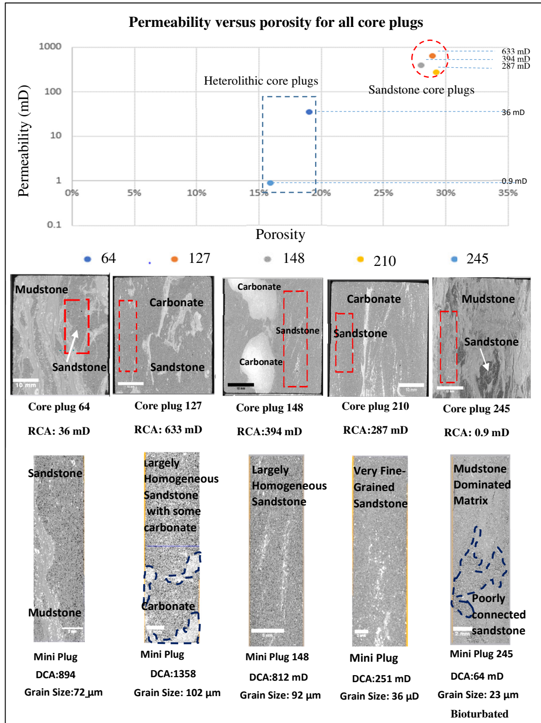
Figure 8.75: Permeability vs. Porosity graph for the five core plugs followed by images of the core plugs and mini plugs indicating the different levels of heterogeneity that affect the measured (RCA) and computed permeabilities(DCA).
