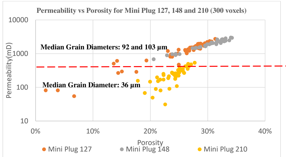
Figure 8.66: The porosity and permeability distribution of mini plug 127, 148, and 210. The results show that the permeability datapoints of mini plug 210 are lower than the other mini plugs. The grain size in mini plug 210 is smaller than in the other mini-plugs by at least 2.5 times that contributed to the lower permeability of mini plug 210.
