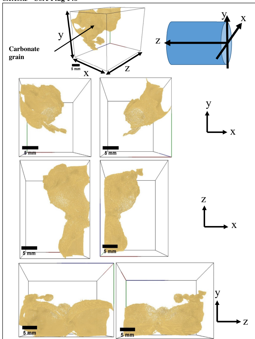
Figure 8.24: 3D volume images of core plug 148 that shows the segmented calcium carbonate that makes up 16% of the core plug volume. The calcium carbonate is a large grain that potentially blocks fluid flow that resulted in lower RCA measured permeability.
