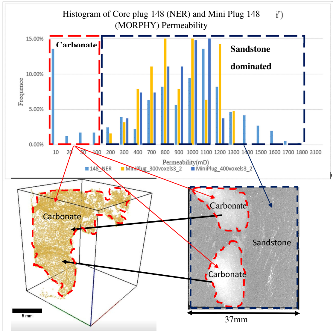
Figure 8.42: Sample 148: Histogram of Permeability results from using MORPHY and the NER Permeability Gas Probe and the 3-D image of the carbonate (bottom left) and the XMCT image (bottom right) with the dashed red and blue lines correlated to the histogram indicating the sandstone dominated matrix and carbonate permeabilities.
