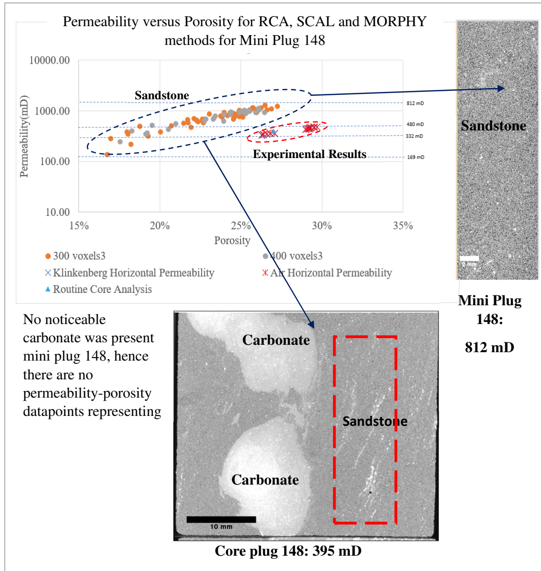
Figure 8.41: Sample 148: Permeability versus Porosity graph of Routine Core (RCA), Special Core Analysis (SCAL), and MORPHY (for 300 voxels and 400 voxels sub-volumes). The Klinkenberg horizontal permeability and horizontal air permeability are the experimental Special Core Analysis results.
