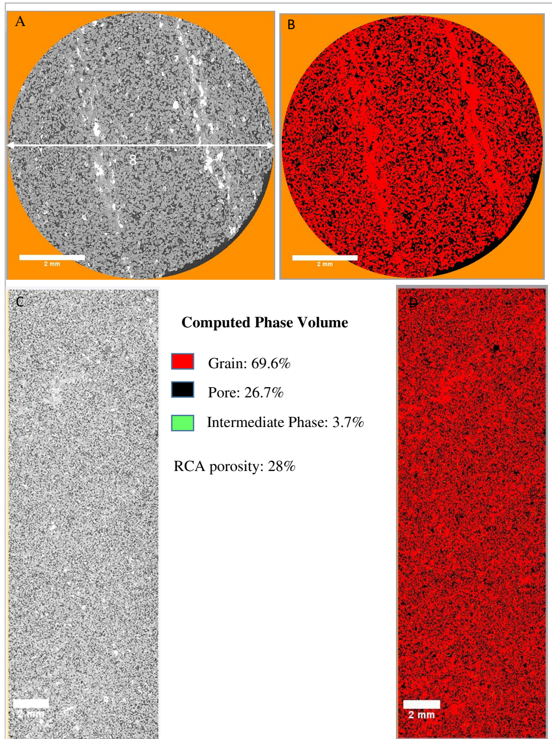
Figure 8.40: Segmented Images of Mini plug 148. A and C: Original unprocessed Greyscale tomogram, B, and D: Segmented tomogram with three-segmented phases (red, green, and black). The green intermediate phase is not visible due to their trace amounts in mini plug 148.
