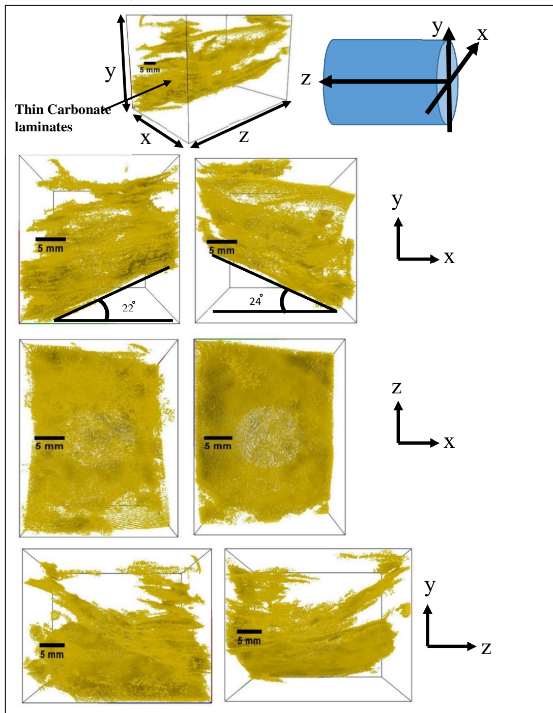
Figure 8.25: 3D volume images of Core Plug 210 showing thin carbonate laminates within the core plug.
