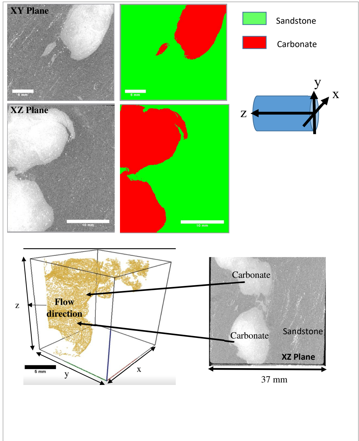
Figure 8.39: Top and Middle Images are greyscaled and segmented images of core plug 148. The left bottom image is a rendered 3D volume of core plug 148, showing the carbonate phase tagged in yellow. The segmented carbonate in core plug 148 occupies 15.8% of its volume.
