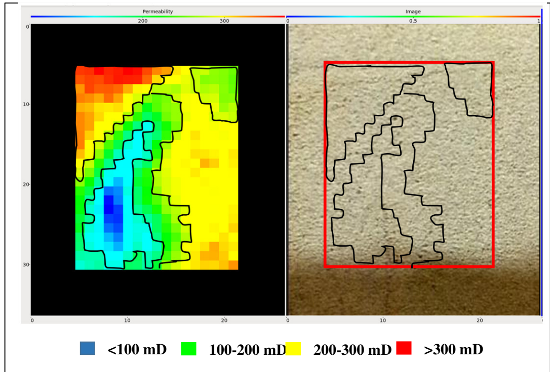
Figure 8.68: Permeability on the surface of the core plug 210 from the NER permeameter. The blue/green areas are low permeability mudstone dominated regions that are below 100 mD while the yellow/green/red areas are permeable sandstone regions that are above 100 mD.
