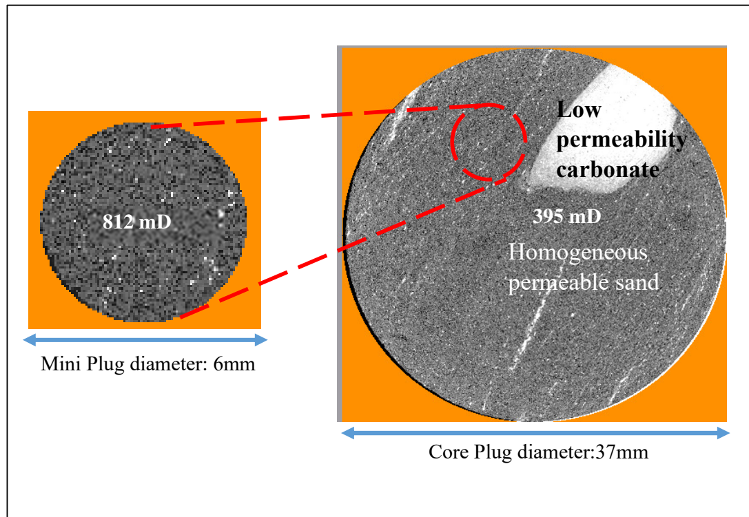
Figure 8.18: Mini plug 148(left) and its location on core plug 148 after 3D to 3D Image Registration. The mini plug is generally sandstone dominated. There is a significant presence of carbonate minerals, as indicated in the image.
