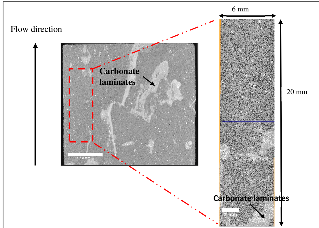
Figure 8.45: Left: Low-resolution image (37 microns/voxel) of core plug 127 and Right: High-Resolution image (3.76 microns/voxel) tomograms of mini plug 127. The location of the mini-plug relative to the core plug is only an approximation.
