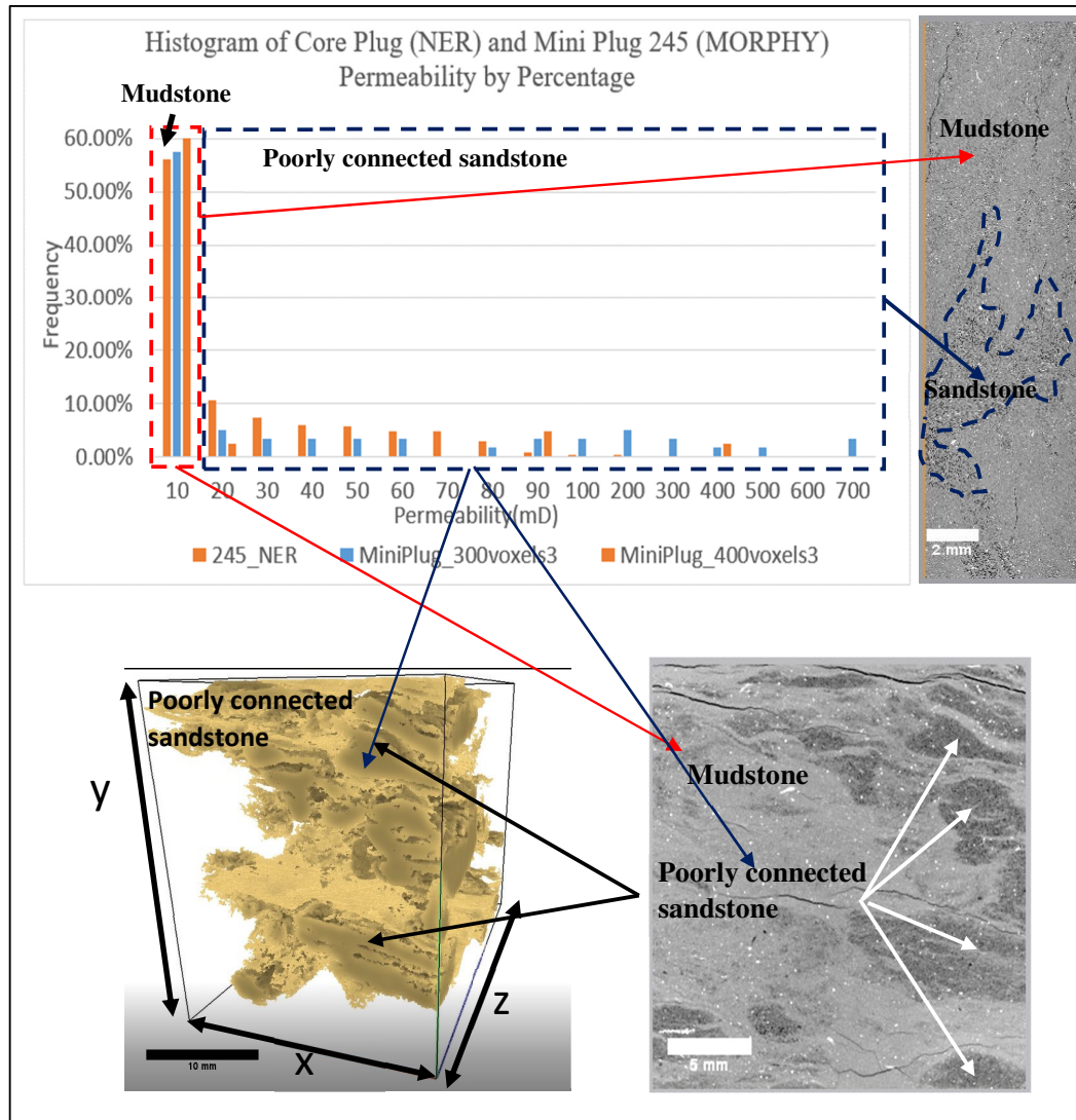
Figure 8.73: Histogram of Permeability results from using MORPHY and the NER Gas Probe. There is a reasonable degree of consistency between the two datasets.
