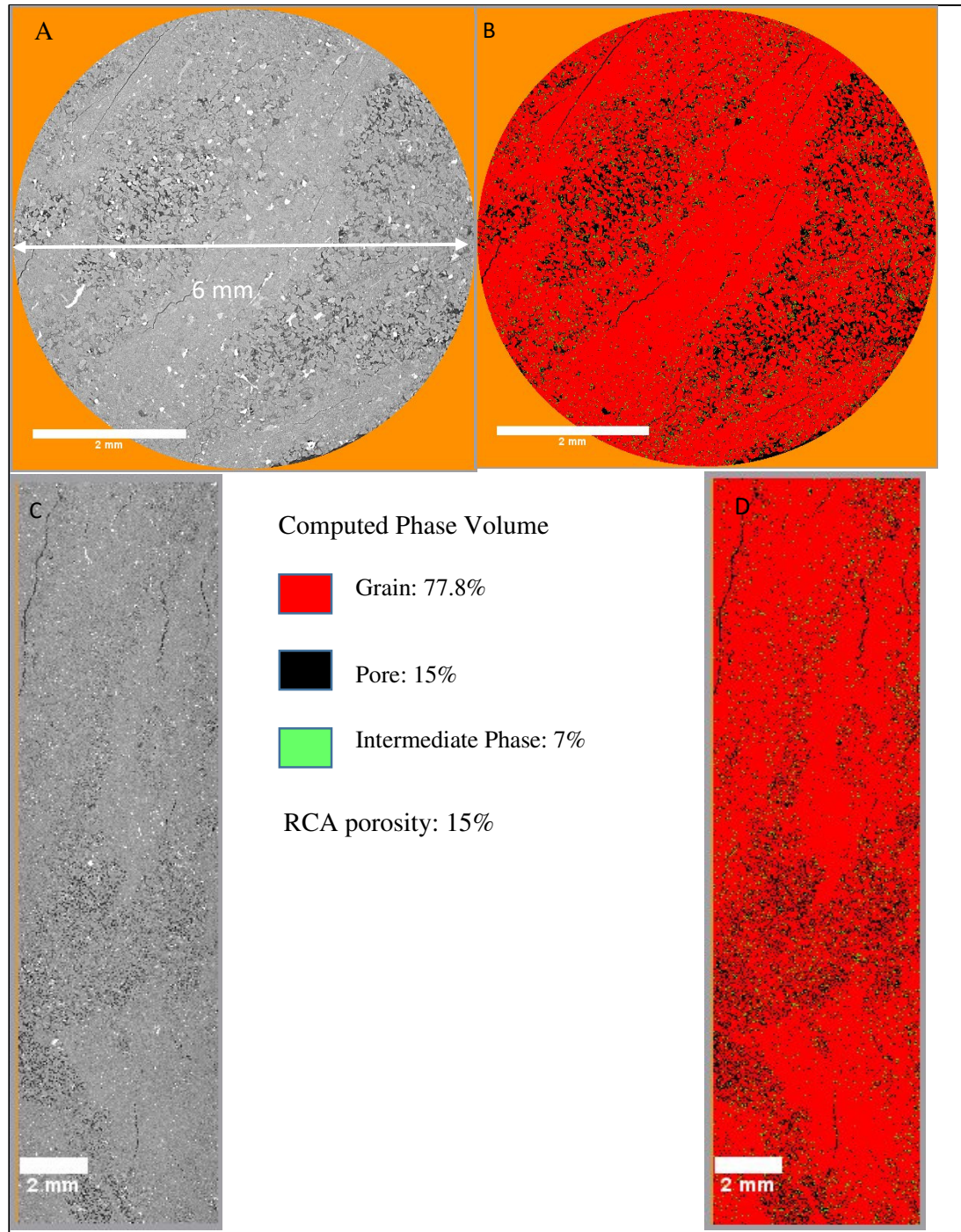
Figure 8.72: Greyscale and segmented images of Mini Plug 245. Image A and C: Greyscale images. Image B and D: Segmented Image and C. It is noted that pores in mini plug 245 are poorly connected and separated by mudstone grains with almost no porosity.
