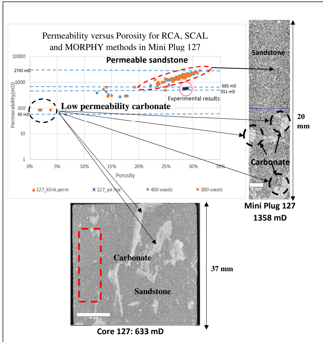
Figure 8.48: Top Left: The permeability-porosity graph of computed permeabilities and experimental permeabilities of sample 127. Top Right: XMCT image of mini plug 127 with sandstone and carbonate phase correlated to the graph to the left. Bottom Middle: XMCT image of core plug 127. We noted that the carbonate has permeability below 100 mD which was validated by the surface permeability map of core plug 127 in Figure 8.16
