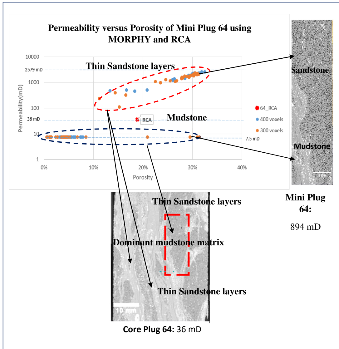
Figure 8.56: The porosity versus permeability of Mini Plug 64 from MORPHY and RCA results. The computed permeabilities in mini plug 64 represent the sandstone and mudstone in core plug 64.
