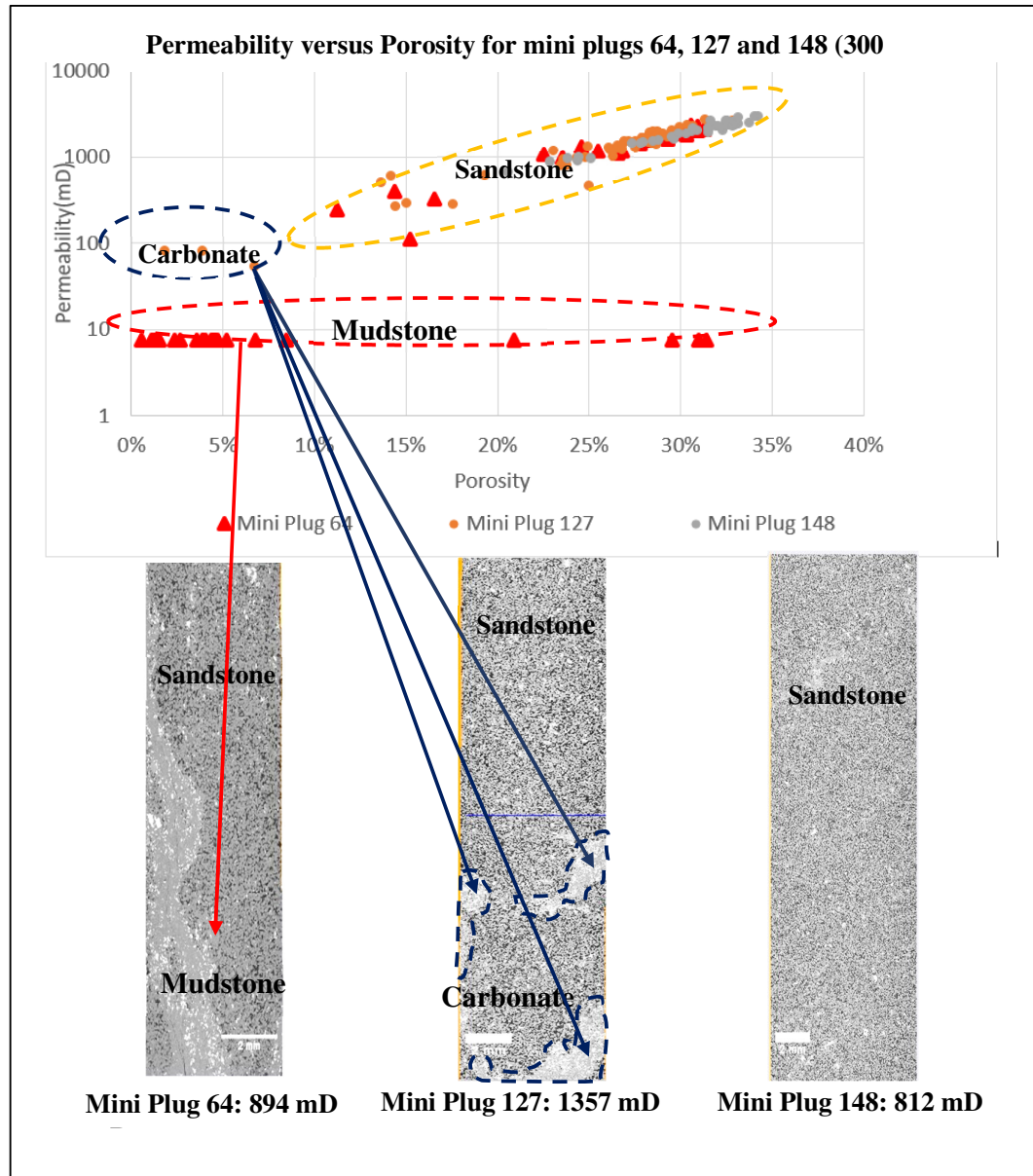
Figure 8.59: Porosity versus Permeability chart of mini plug 64 and mini plug 127 and 148. The sandstone of the three mini-plugs is statistically consistent with similar porosity-permeability gradients.
