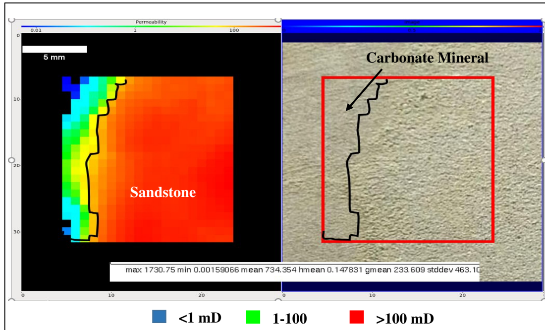
Figure 8.43: Permeability map on the surface of the core plug 148 from the NER Permeability Gas Probe. The blue areas are low permeability carbonate regions.
