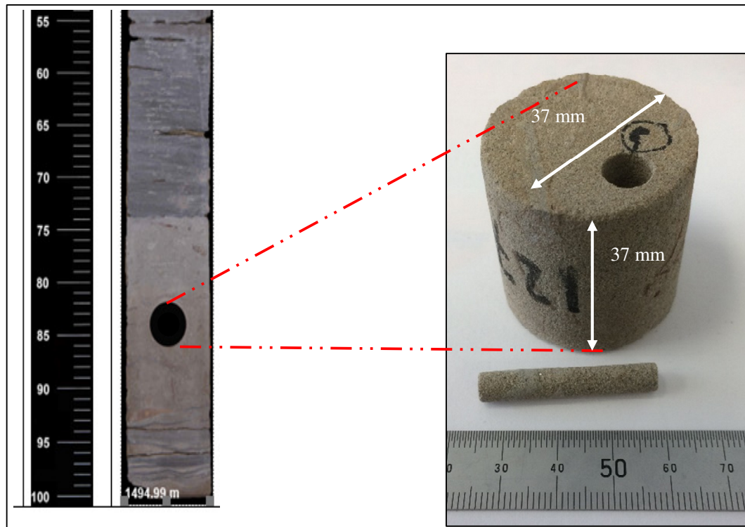
Figure 8.44: A view of the core (left) indicating distinct layers of dark colored mudstone and light-colored sandstone and core plug 127 (right).
