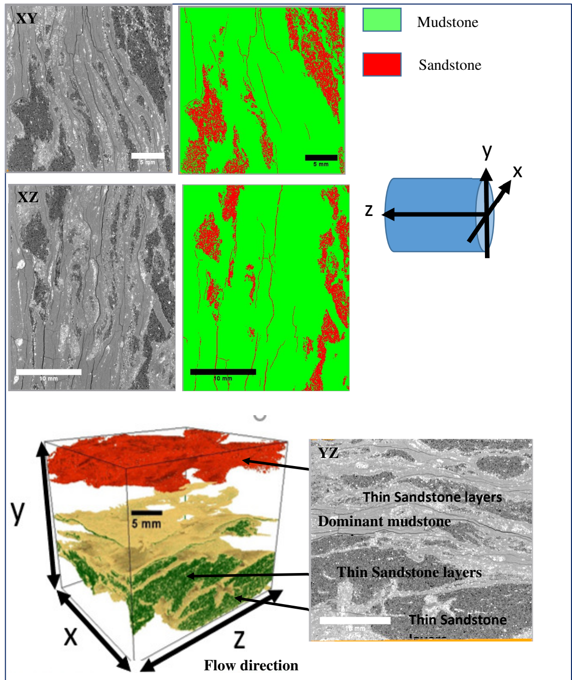
Figure 8.54: Top and Middle Images are greyscaled images and segmented images of core plug64. The left bottom left image is a rendered 3D volume of core plug 64, showing the sandstone phase tagged in red and yellow. The different colours indicate that the sand layers are not connected. The segmented sandstone in core plug 64 occupies 15% of its volume.
