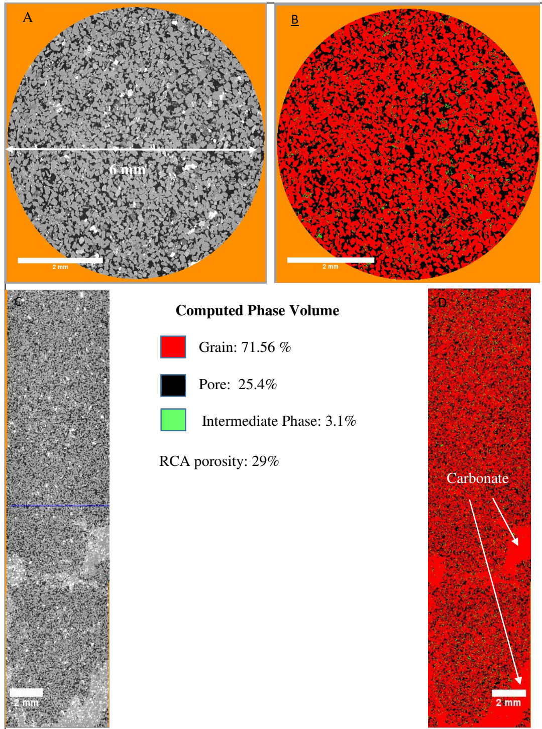
Figure 8.47: Images of Mini Plug 127. A and C: Original unprocessed Greyscale tomogram, B, and D: Segmented image of mini plug 127.
