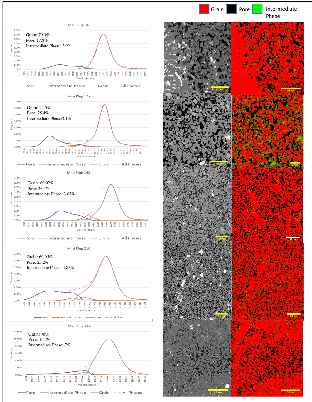
Figure 8.7: Left: Voxel Intensity Histograms for the five mini plugs. Right: Greyscale and segmented images of the mini plug.
