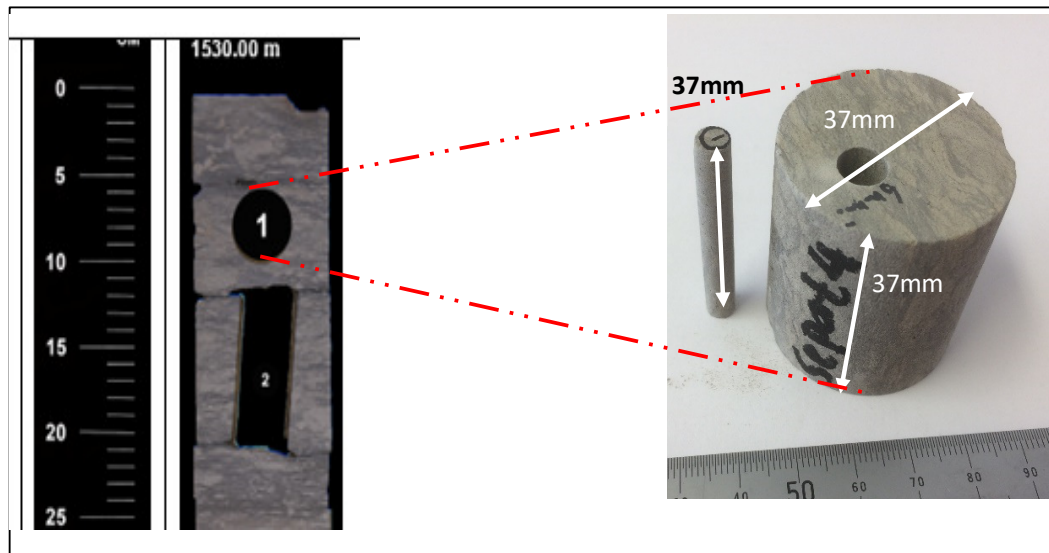
Figure 8.69: A view of core plug 245 and the core slab that indicates dark-coloured mudstone with intercalated with thin streaky layers of light-colored sandstone.
