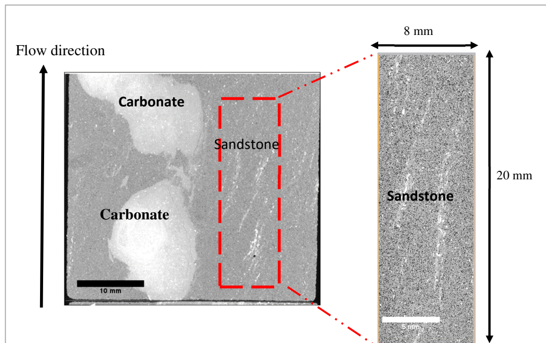
Figure 8.38: Left: Low resolution (16.3 microns/voxel) and Right: High Resolution (3.74 microns/voxel) tomograms of core plug and mini plug 148, respectively. The bright areas represent carbonate minerals. We also indicate the direction of fluid flow through the core plug and mini plug.
