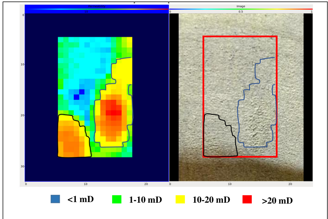
Figure 8.74: Permeability map of the surfaces of core plug 245 showing permeability contrast between sandstone (yellow and red) and the tight mudstone matrix (green and blue)
