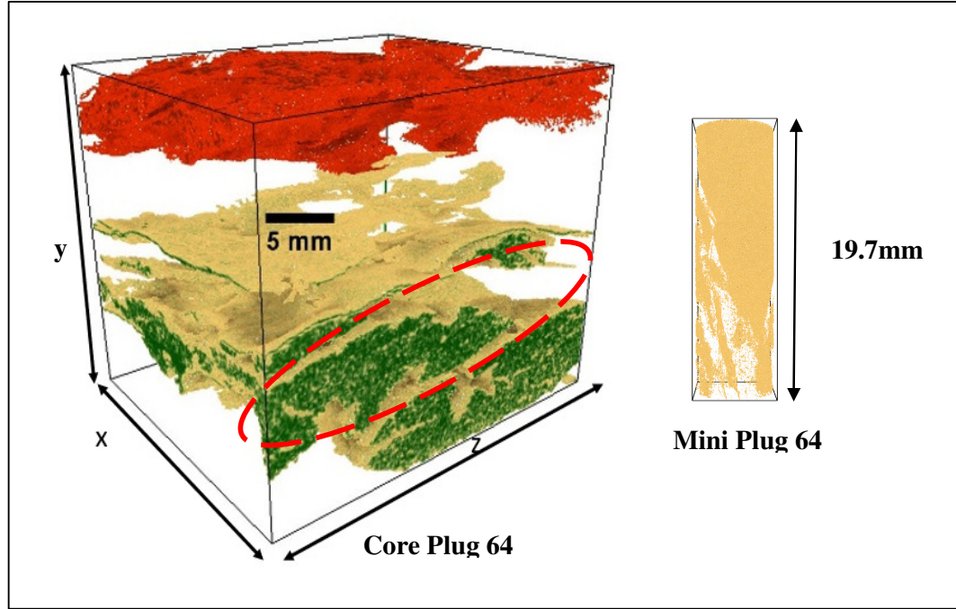
Figure 8.16: Rendered sandstone layers in core plug 64 using Drishti visualization software with the rendered mini plug 64 to the right for comparison. The green sandstone layer inside the red circle in core plug 64 is the general area from which we extracted mini plug 64.
