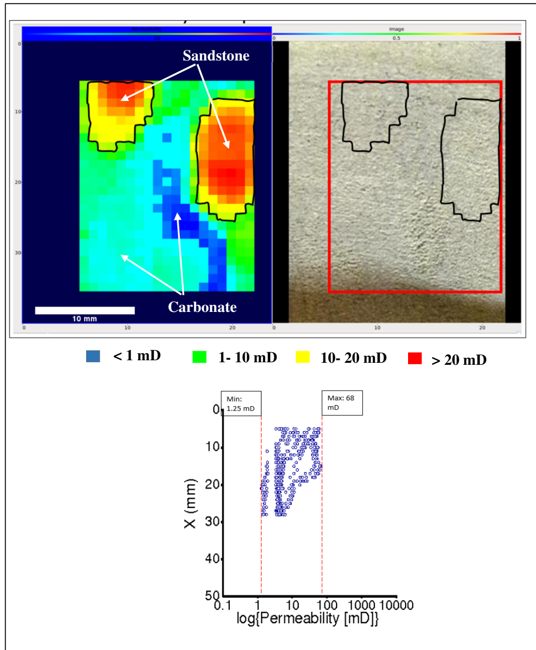
Figure 8.36: Permeability map of core plug 245, side B.
