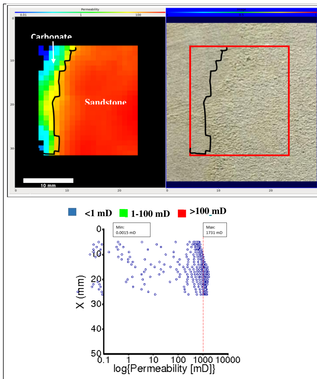
Figure 8.31: Permeability map of core plug 148, side A.
