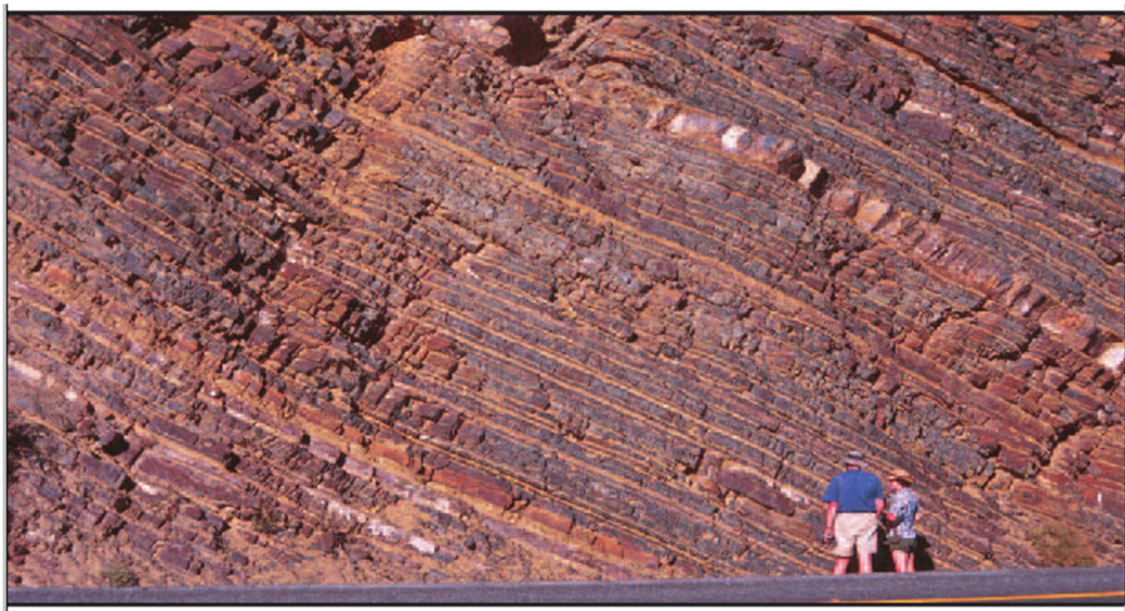
Figure 2.5: An example of a thin bed outcrop. Deep-water Turbidites, Permian Collingham Formation, Bavians Syncline, Laingsburg Karoo, South Africa. Picture by Anthony Spragues (Passey et al., 2006)
