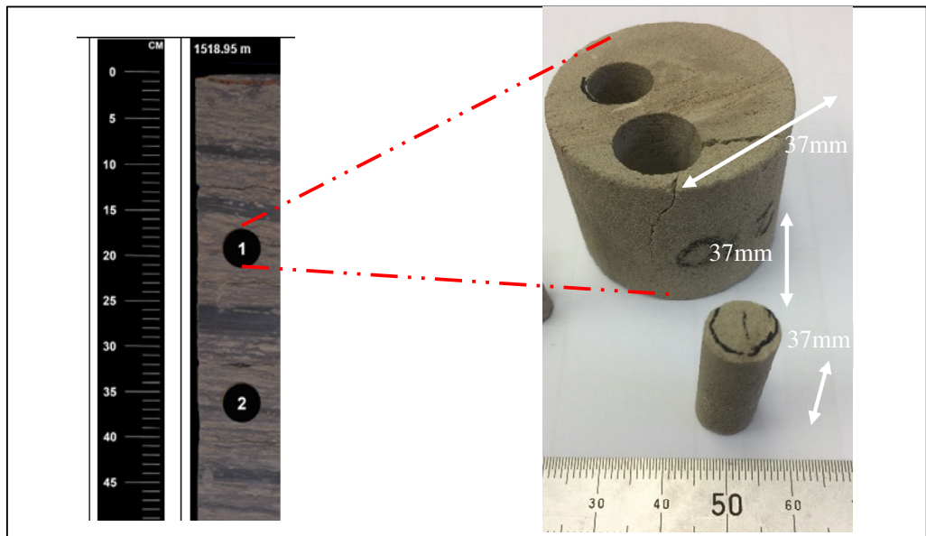
Figure 8.61: A view of core plug 210 and the core slab that indicates light-coloured sandstone with interbedded mudstone and siltstone layers.
