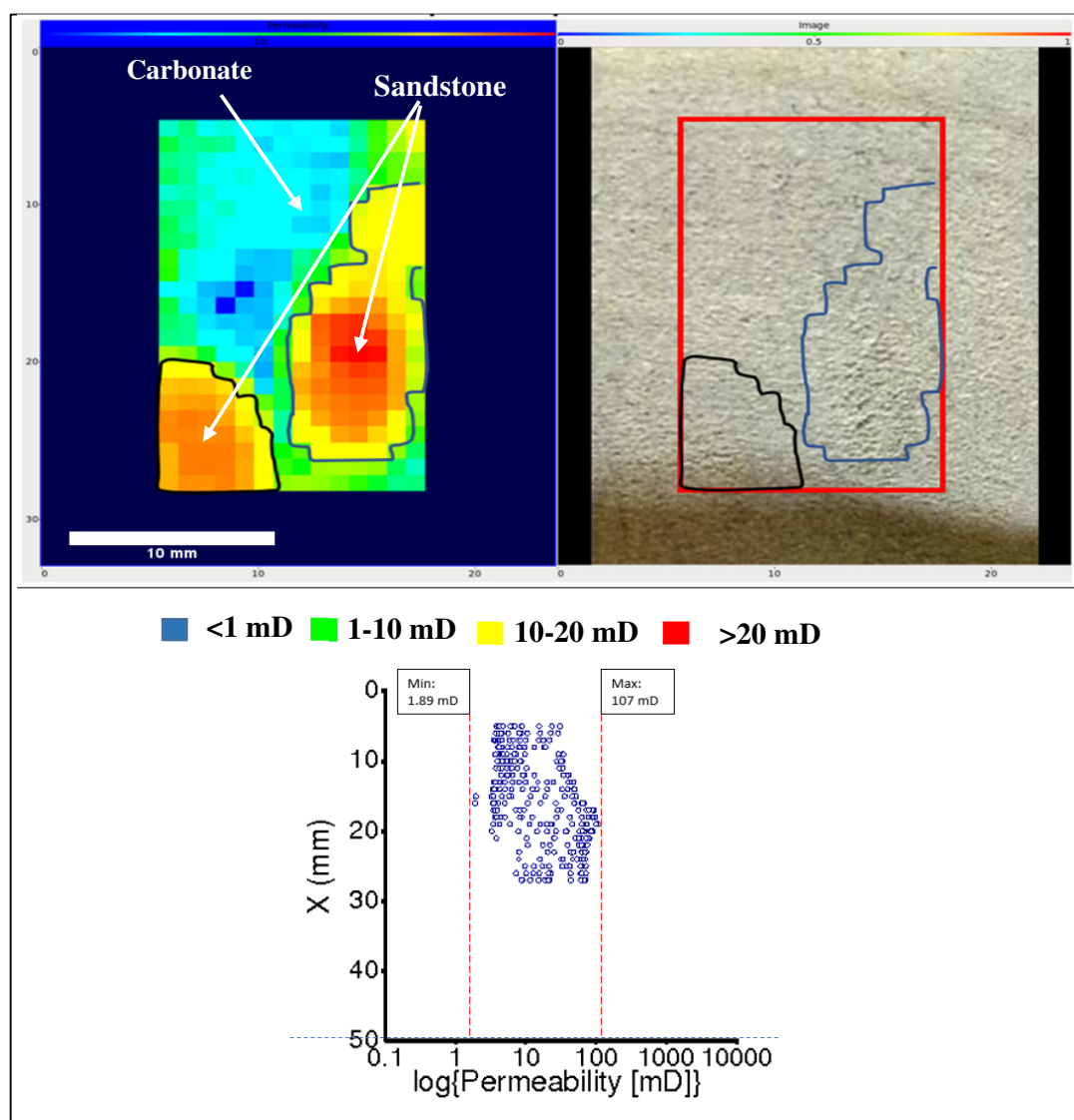
Figure 8.35: Permeability map of core plug 245, side A.
