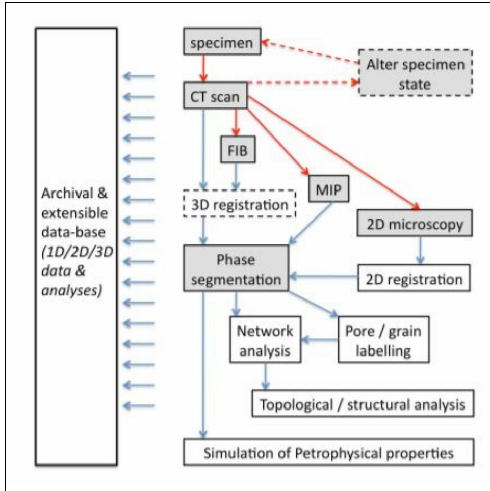
Figure 4.1: A proposed workflow used for specimens analyzed using Computer Tomography Imaging at the Australian National University (Kumar et al., 2013). MIP= Mercury Intrusion Porosimetry.
