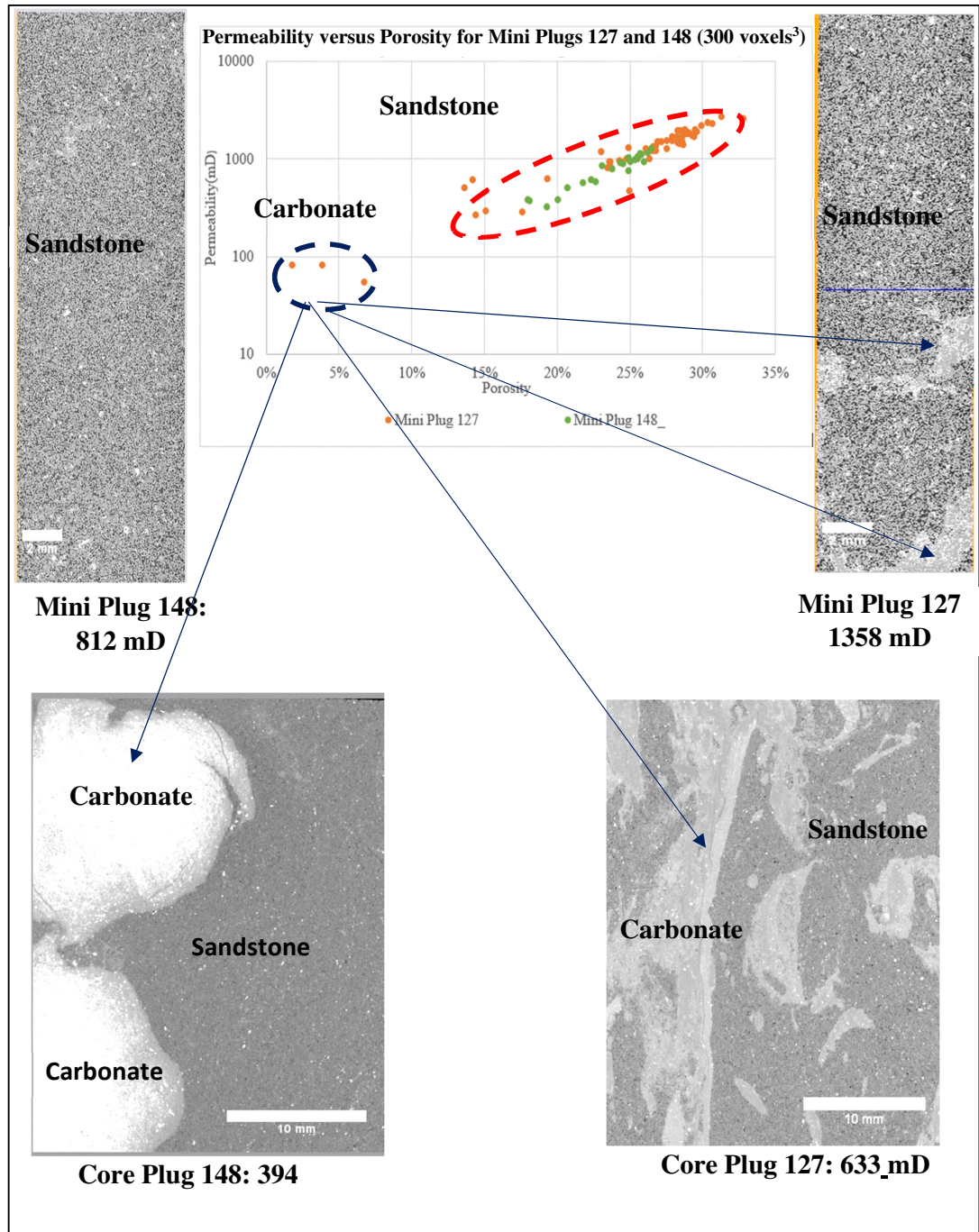
Figure 8.49: Permeability versus Porosity for mini plug 127 and 148, indicating that the gradient of the sandstone in both mini-plugs is relatively similar. With the low permeability data points below 100 mD captured in mini plug 127 representing the carbonate mineral. As sample 127 and 148 are only 6 meters apart, the carbonate in sample 127 and 148 should be similar.
