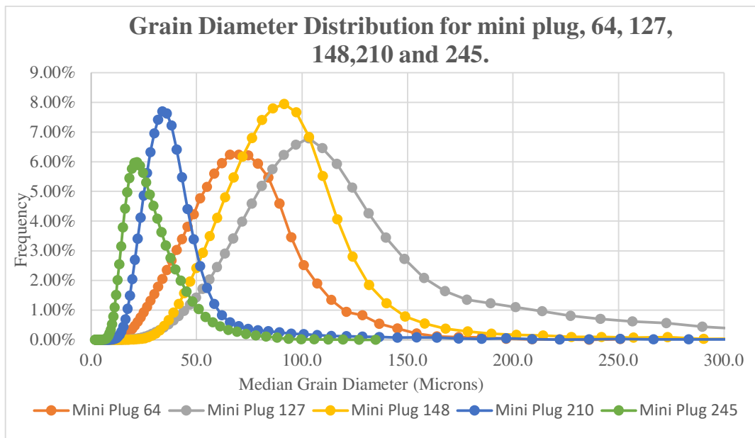
Figure 8.8: Grain size distribution calculated from the images of the mini-plugs.
