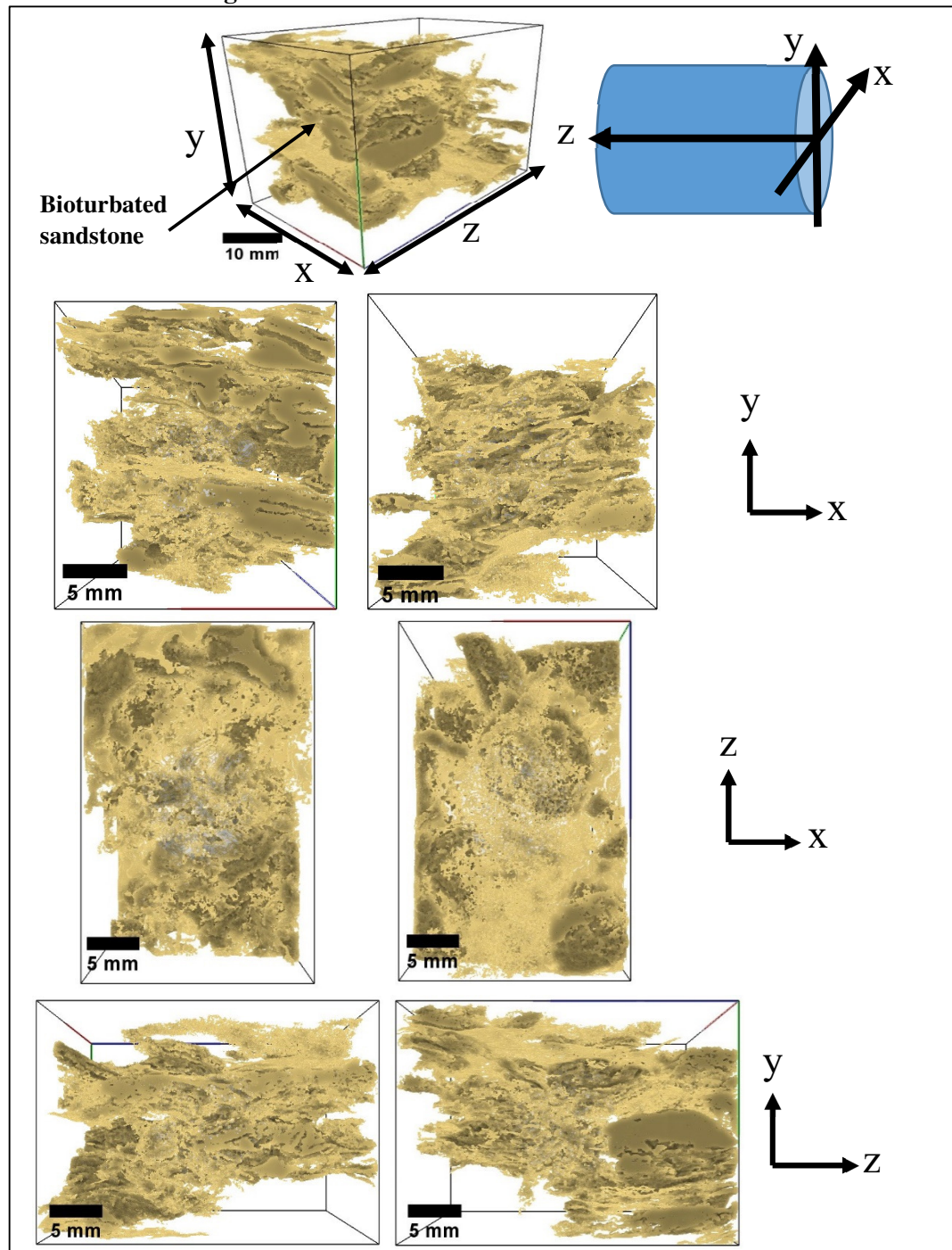
Figure 8.26: 3D Volume images of Core Plug 245, showing the sandstone phases. The bioturbated sandstone layers consist of very thin sheets that are poorly connected.
