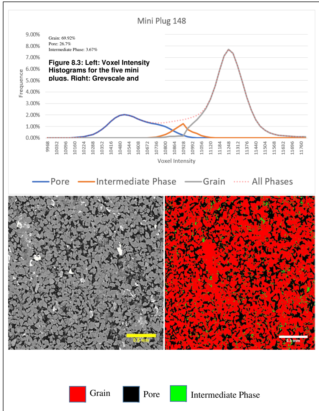
Figure 8.4: Top: Voxel Intensity Histograms of mini plug 148. Bottom: Greyscale and segmented images the mini plug 148.
