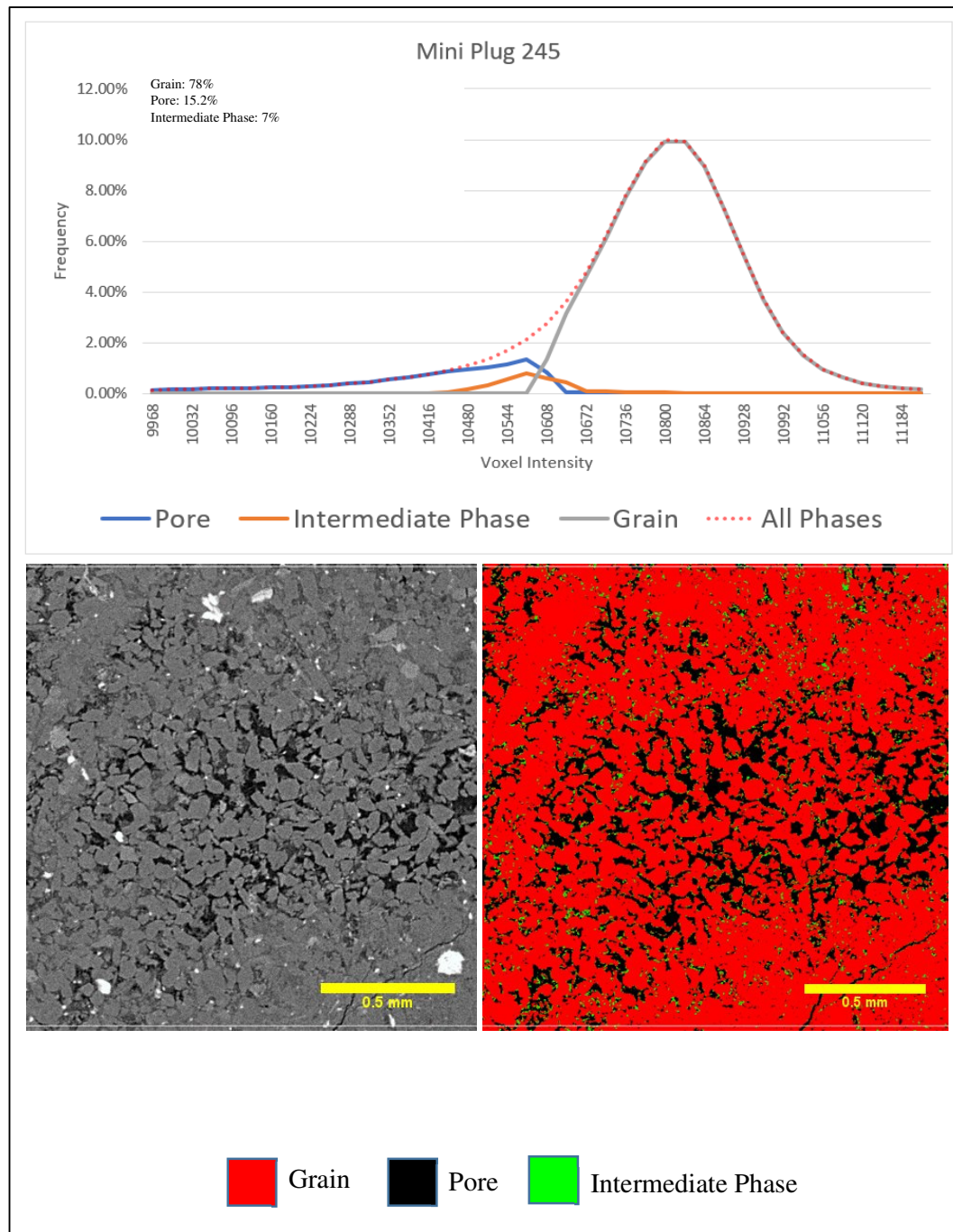
Figure 8.6: Top: Voxel Intensity Histograms of mini plug 245. Bottom: Greyscale and segmented images the mini plug 245.
