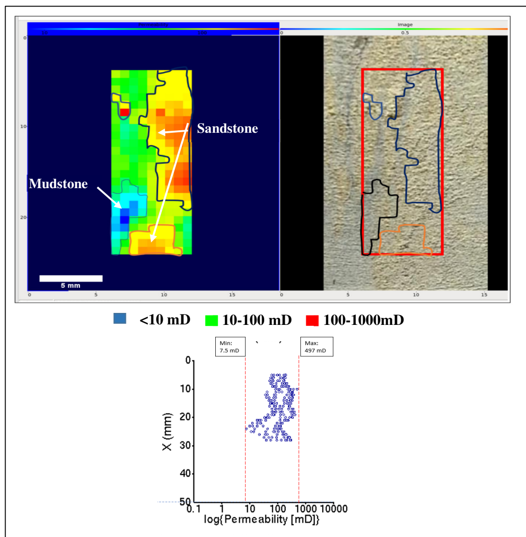
Figure 8.27: Permeability map of core plug 64, side A.
