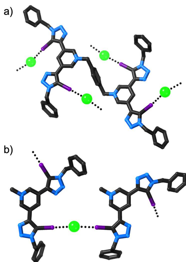
Figure 5 Two views of the structure of 2^{\text{I}}_{\text{Bn}}^{2+}\text{Cl}_2 : a) view showing a complete receptor with all positions of the anion, b) view showing two partial receptors forming linear interactions with a single anion. Halogen bonds shown as dotted lines, hydrogen atoms omitted for clarity.
