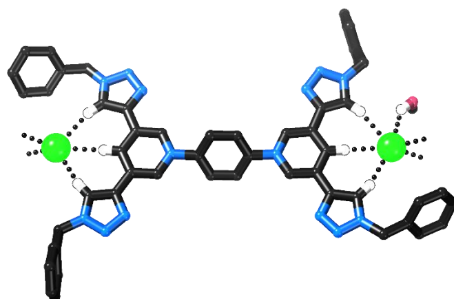
Figure 6 Structure of 7 H -Cl 2 : only hydrogen atoms involved in hydrogen bonding are shown, hydrogen bonds are shown as dotted lines. the dotted lines without a donor group represent relatively long hydrogen bonds (86–89% \Sigma_{\text{vdW}} ) to phenylene C–H donors of an adjacent receptor.
