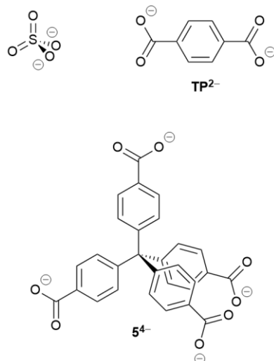
Figure 3 2- and 4- anions used in crystallisation studies.
