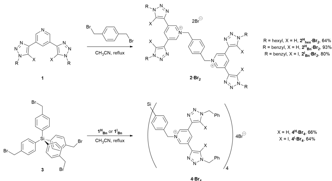
Scheme 1 Synthesis of flexible ditopic receptors \mathbf{2^H_{hex} \cdot Br_2} , \mathbf{2^H_{Bn} \cdot Br_2} and \mathbf{2^I_{Bn} \cdot Br_2} , and flexible tetratopic receptors \mathbf{4^H \cdot Br_4} and \mathbf{4^I \cdot Br_4} . All of these receptors were also anion exchanged to give the corresponding \text{BF}_4^- or \text{PF}_6^- salts.
