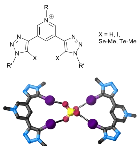
Figure 1 General structure of btp motif, and partial crystal structure showing two iodo- btp groups arranged around a sulfate anion reported by Beer 48 (CSD: 1033648).
