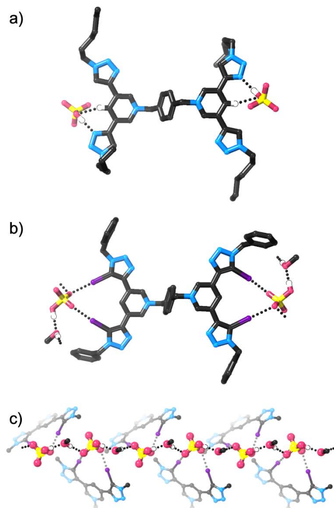
Figure 4 Structures of \text{HSO}_4^- complexes of 2^{\text{H}}_{\text{hex}}^{2+} and 2^{\text{I}}_{\text{Bn}}^{2+} : a) structure of 2^{\text{H}}_{\text{hex}}^{2+}(\text{HSO}_4)_2 , b) structure of 2^{\text{I}}_{\text{Bn}}^{2+}(\text{HSO}_4)_2 , c) structure of \text{HSO}_4^- -methanol hydrogen bonded polymer in the structure of 2^{\text{I}}_{\text{Bn}}^{2+}(\text{HSO}_4)_2 . Only hydrogen atoms involved in hydrogen bonding are shown, with hydrogen bonds shown as dotted lines. PLATON-SQUEEZE 57 was used in the refinement of 2^{\text{H}}_{\text{hex}}^{2+}(\text{HSO}_4)_2 .
