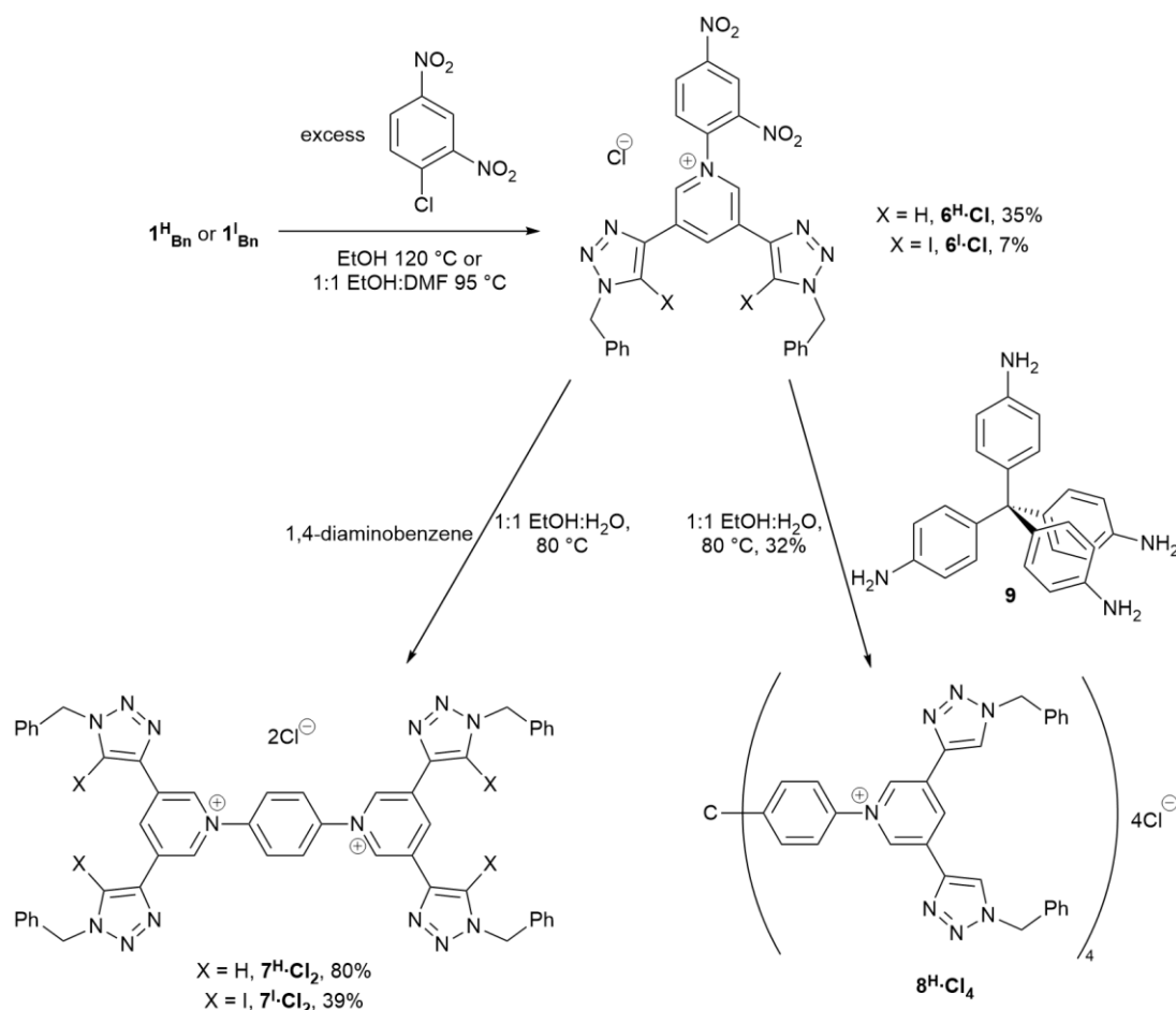
Scheme 2. Synthesis of Zincke salts 6 H -Cl and 6 I -Cl , and rigid receptors 7 H -Cl 2 , 7 I -Cl 2 and 8 H -Cl 4 . The ditopic and tetratopic receptors were also anion exchanged to give the corresponding \text{BF}_4^- or \text{PF}_6^- salts.
