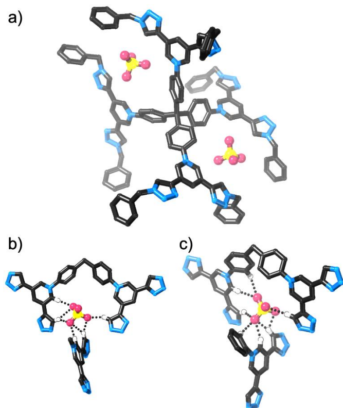
Figure 7 Structure of 8 H+ (SO 4 ) 2 : a) view of the asymmetric unit cell (hydrogen atoms omitted), b and c) view of the hydrogen bonding environments around each independent SO 4 2- anion (only hydrogen atoms involved in hydrogen bonding shown, hydrogen bonds shown as dotted lines). PLATON-SQUEEZE 57 was used.
