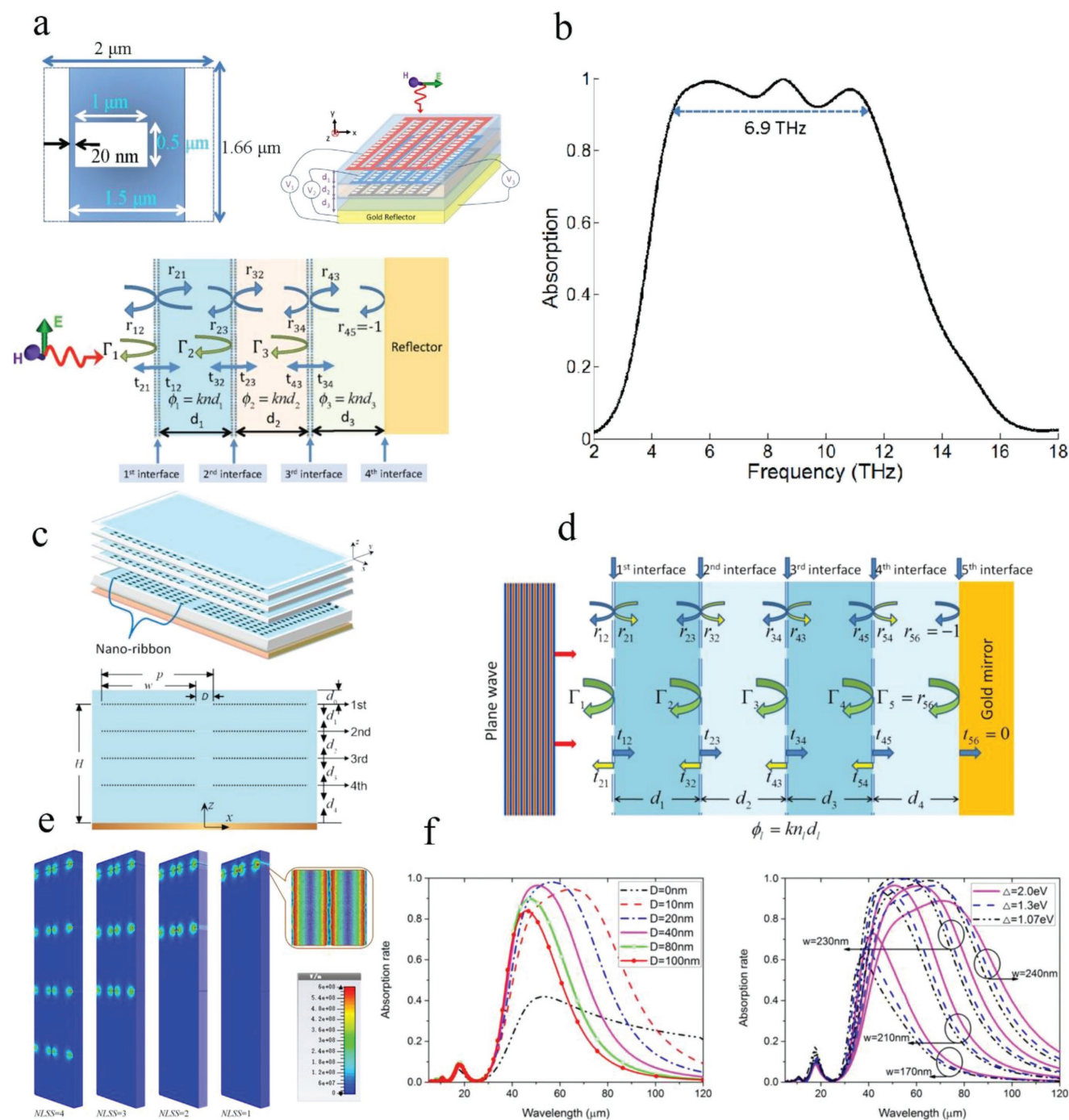
Figure 7. a) The schematic diagram of the proposed absorber with three layers of graphene (top right). The graphene unit cell with an asymmetric void with its dimensions (top left). Description of the transmission line model for the multilayered absorber (bottom). b) The absorption spectra of the three-layer design with d_1 = 0.67 \mu\text{m} , d_2 = 0.5 \mu\text{m} , and d_3 = 4.78 \mu\text{m} . c) Schematic of the proposed sandwich-like structured BP absorber and front view of the proposed absorber with layer dimensions. d) A schematic diagram of the transmission and reflection for a four-layered sandwich-like BP structure. e) Simulated average electric field intensity values for monolayer BP MM with two nanoribbon periods aligned along the x-direction. The inset presents a sectional view at the in-plane across the first interface for NLSS value of 1. f) Simulated absorption rate spectra for TM polarization at various distances between two nanoribbons and for various thicknesses of BP in monolayer, bilayer, and trilayer with ridges perpendicular to the x-direction. (a,b) Reproduced with permission. [105] Copyright 2013, Optical Society of America. (c–f) Reproduced with permission. [79] Copyright 2017, Optical Society of America.
