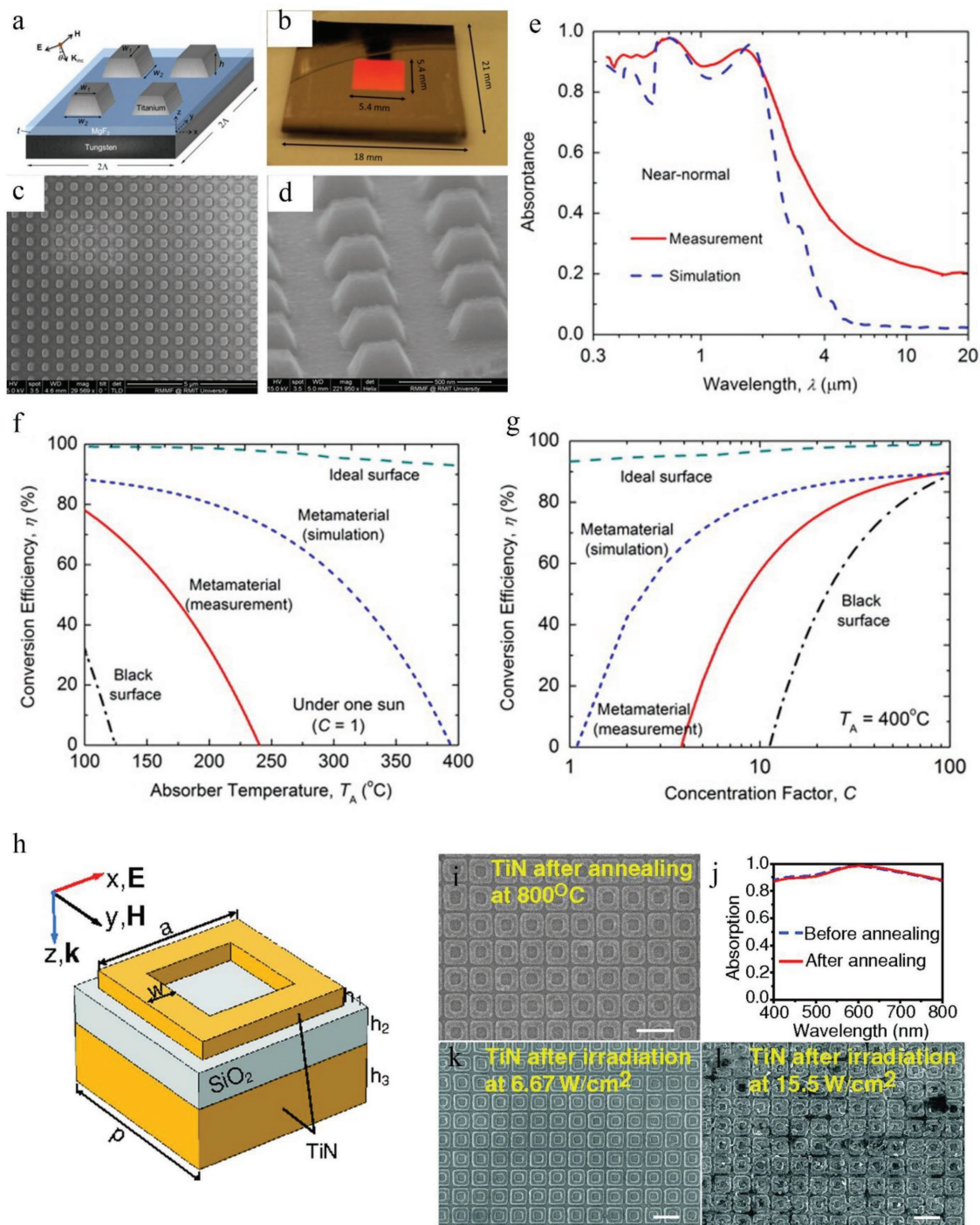
Figure 15. a) Structure schematic for proposed MM solar absorber. K_{\text{inc}} represents the incident wavevector, and the incidence angle \theta is defined as the angle between K_{\text{inc}} and the surface normal. The plane of incidence (POI) is defined as the xz -plane. The E field is in the POI for TM incidence, while it is perpendicular to the POI for TE incidence. b) Photo of the fabricated sample for optical characterization. SEM images of the fabricated absorber sample from c) top view and d) side view. e) Measured and simulated room-temperature spectral absorbance of the MM solar absorber. f) Predicted solar-to-heat conversion efficiencies of an ideal selective surface, the MM solar absorber (with optical properties either measured or simulated), and a black surface as a function of absorber temperature T_A under 1 sun. g) Solar-to-heat conversion efficiency for all three surfaces as a function of concentration factor C at an absorber temperature of T_A = 400^{\circ}\text{C} . h) Schematic representation of a unit cell of the three-layer TiN MMPA with dimensions of a = 250 \text{ nm} , w = 50 \text{ nm} , p = 300 \text{ nm} , h_1 = 30 \text{ nm} , h_2 = 60 \text{ nm} , and h_3 = 150 \text{ nm} . i) SEM image and j) the measured absorbance of the TiN absorber after annealing at 800^{\circ}\text{C} for 8 h, as well as the reference measured absorbance of TiN before annealing; SEM images for the TiN absorber after being illuminated by a laser with an intensity of k) 6.67 and l) 15.5 \text{ W cm}^{-2} . (a–g) Reproduced with permission. [68] Copyright 2015, Elsevier B.V. (h–l) Reproduced with permission. [16] Copyright 2014, Wiley-VCH.
