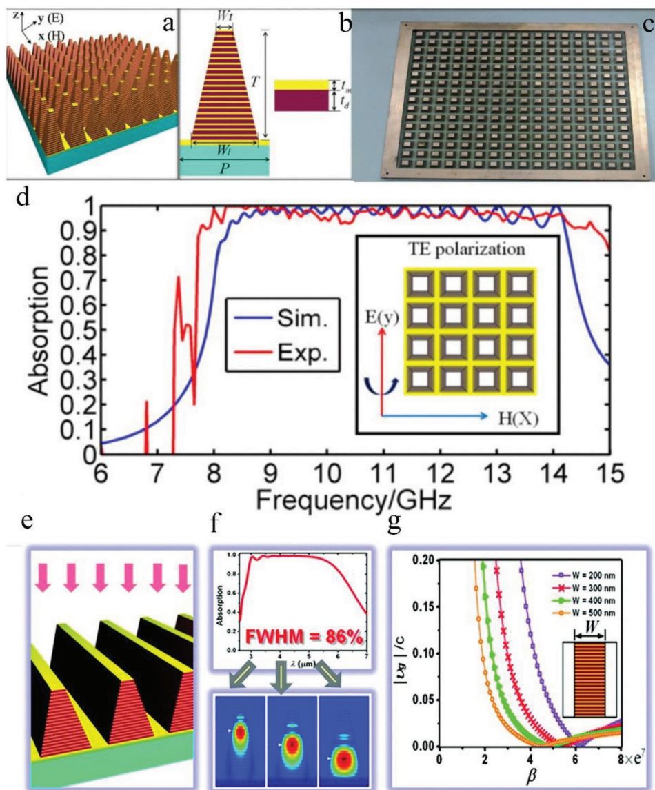
Figure 5. a) 3D illustration of the simulated MMMPA, b) schematic of a MMMPA unit cell, and c) photograph of the fabricated sample. The optimized dimensions of a unit are W_t = 5 mm, W_l = 9 mm, P = 11 mm, t_m = 0.05 mm, t_d = 0.2 mm, and T = 5 mm. Subscript “m” represents copper, and “d” for FR4. d) Comparison between the simulated absorption (blue line) and experimental absorption (red line). The inset shows the configuration of the incident wave. e) Diagram of the sawtooth anisotropic MM thin film absorber. Light of TM polarization is incident along z-direction. f) Absorption spectra for the sawtooth MMMPA and distributions of magnetic field corresponding to 3.5, 4.5, and 5.5 \mu m, respectively. g) Relationship between the group velocity and propagation constant (proportional to wavevector) at different W . (a–d) Reproduced with permission. [102] Copyright 2012, AIP Publishing. (e–g) Reproduced with permission. [82] Copyright 2012, American Chemical Society.
