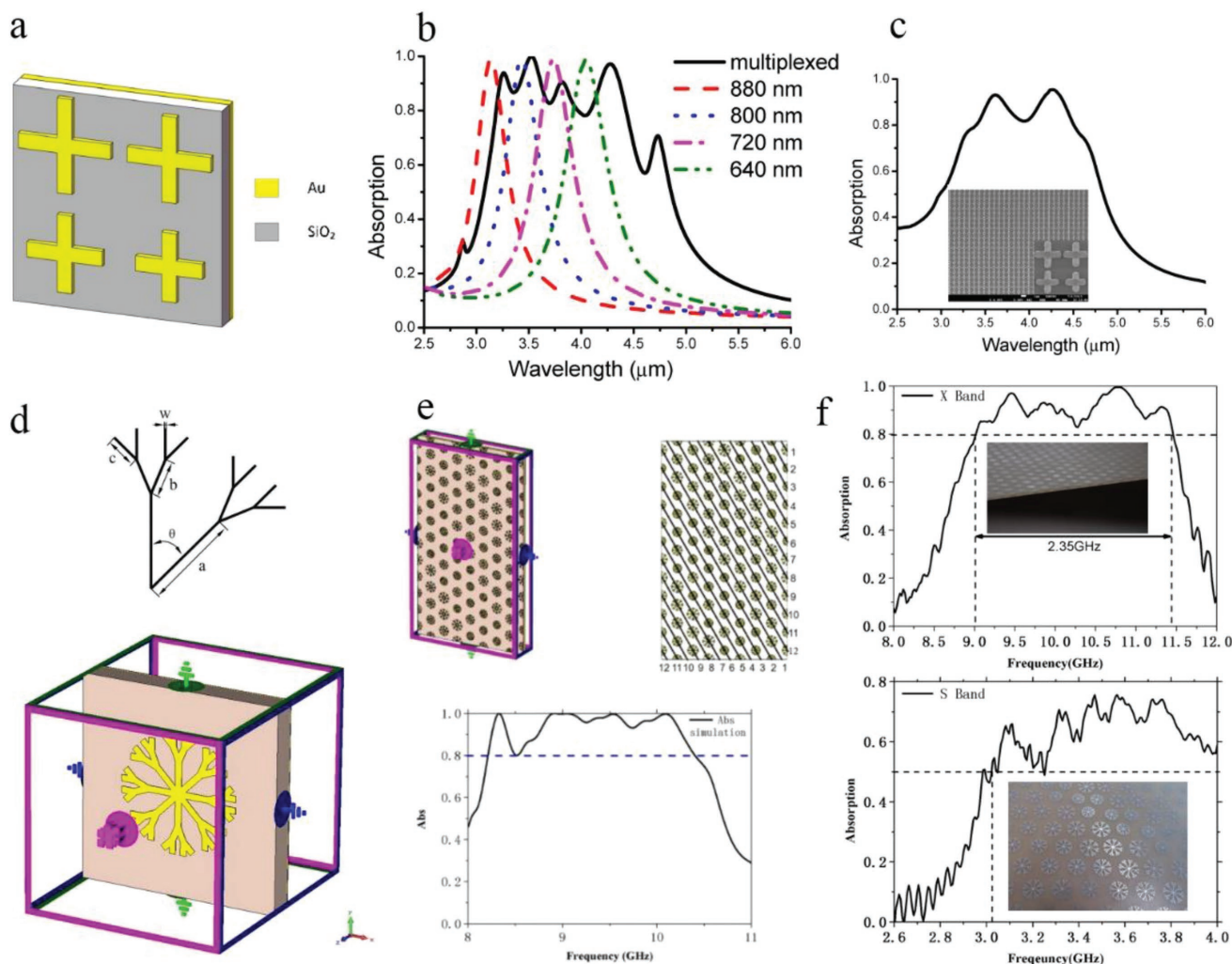
Figure 3. a) Unit cell schematic diagram of four cross resonators. The gold layer is 100 nm thick for the ground plane and 60 nm for the metallic patterns. The SiO 2 dielectric layer is 190 nm. b) Simulated absorption of multiplexed and four traditional non-multiplexed absorbers. c) Measured absorption for multiplexed absorber. The inset is a SEM image of the multiplexed absorber. d) Three-level dendritic structure and dendritic unit cell in the simulation model. e) The schematic of the X-band absorber composed of 12 kinds of independent units and its simulation result. f) The experimental results of the X-band and S-band absorbers. (a–c) Reproduced with permission. [62] Copyright 2013, Optical Society of America. (d–f) Reproduced with permission. [58] Copyright 2013, AIP Publishing.
