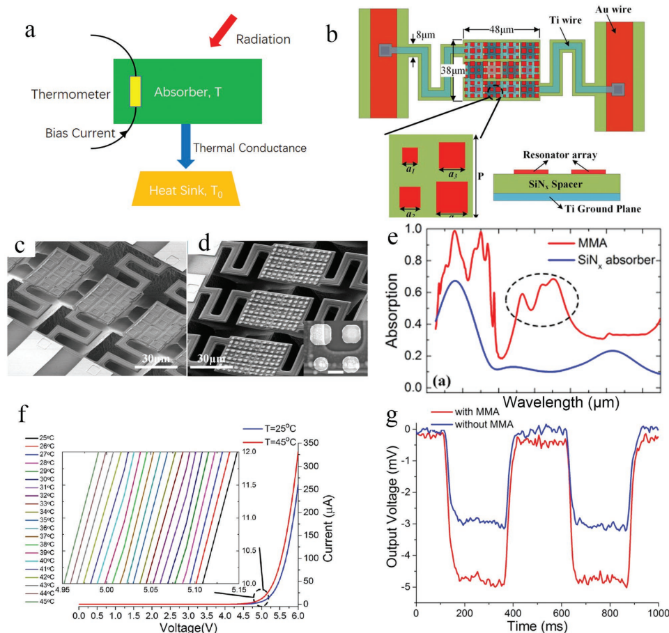
Figure 20. a) A typical bolometer structure including a BMMPA. b) Top view of the designed microbolometer. c,d) SEM pictures of the fabricated microbolometers without and with BMMPA. The zoomed-in picture in (d) is the unit cell of the resonator array (scale bar: 2 \mu\text{m} ). e) Simulated absorption of BMMPA and the ordinary \text{SiN}_x absorber; f) I - V characteristics of the fabricated microbolometer at the two different device temperatures of 25 and 45 ^{\circ}\text{C} , respectively. The inset is the zoomed-in view of different I - V curves with a 1 ^{\circ}\text{C} step around a 10 \mu\text{A} bias. g) Transient responses of the microbolometers under modulated IR incidence at a bias current of 10 \mu\text{A} . (b–g) Reproduced with permission. [173] Copyright 2016, Optical Society of America.
