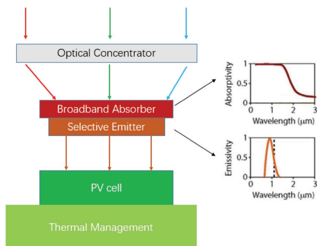
Figure 14. Schematic of STPV systems. The absorber and emitter typically operate above 1000 K while the PV cell operates at room temperature.
