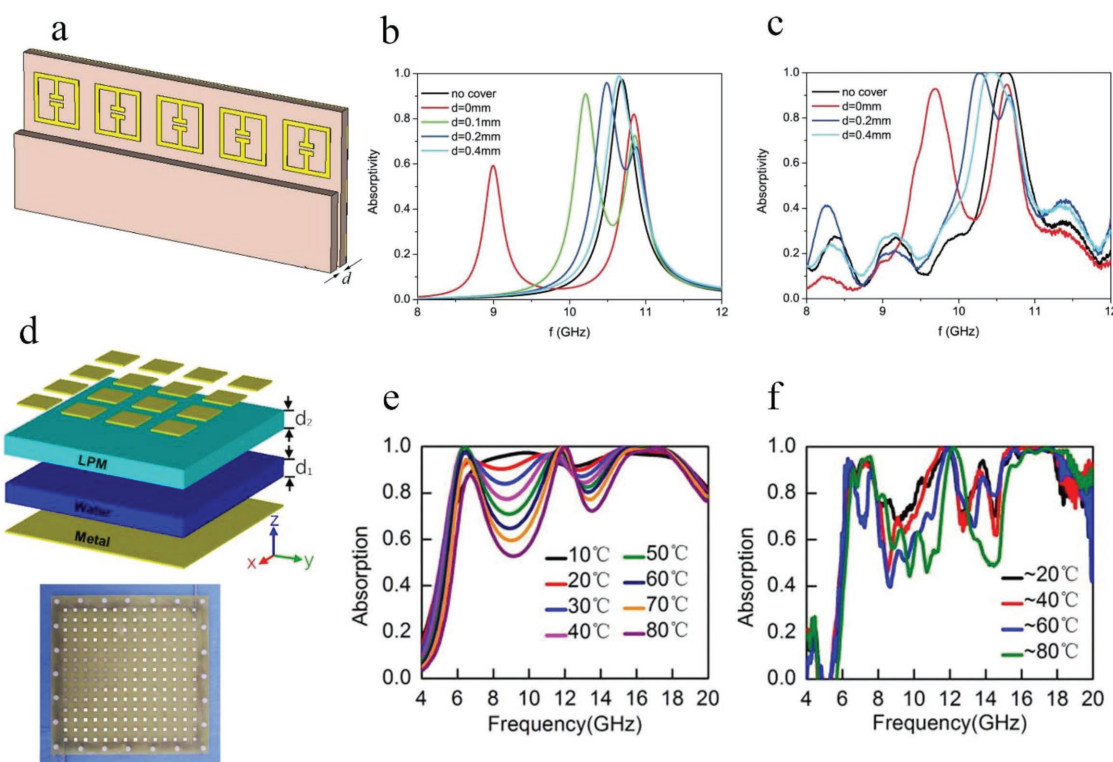
Figure 11. a) BMMPA with a horizontal half-slab; b) theoretical and c) experimental absorption spectra for different d . d) 3D schematic diagram of the water-substrate BMMPA and optical image of the assembled prototype of the water-substrate BMMPA; e) simulated and f) measured absorption spectra of the fabricated water-substrate BMMPA at different temperatures. (a–c) Reproduced with permission. [124] Copyright 2012, Optical Society of America. (d–f) Reproduced with permission. [89] Copyright 2017, AIP Publishing.
