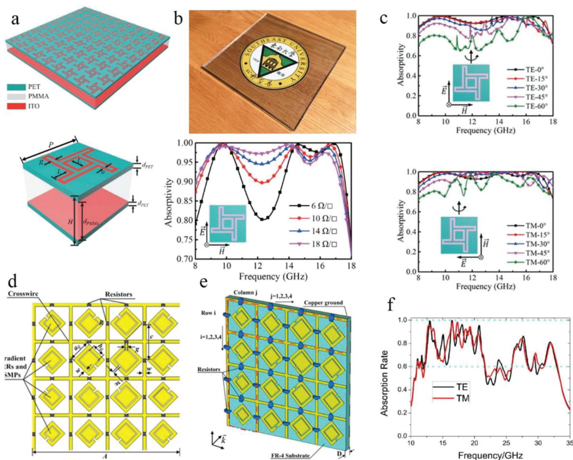
Figure 4. a) Schematics of an optically transparent B MMPA. b) Photograph of the fabricated sample and simulated absorptivity spectra with the increase of surface resistance of the ITO layer at normal incidence of TE wave, with the polarization direction illustrated in the inset. c) The angular dependence of the simulated absorptivity spectra for the MMA under the incidence of TE and TM waves, with the polarization direction and the incidence angle \theta illustrated in the insets. The structure of the unit cell of a proposed integrated B MMPA: d) plan view and e) stereogram. f) The calculated absorption rate for both TE and TM wave. (a–c) Reproduced with permission. [73] Copyright 2017, AIP Publishing. (d–f) Reproduced with permission. [86] Copyright 2014, AIP Publishing.
