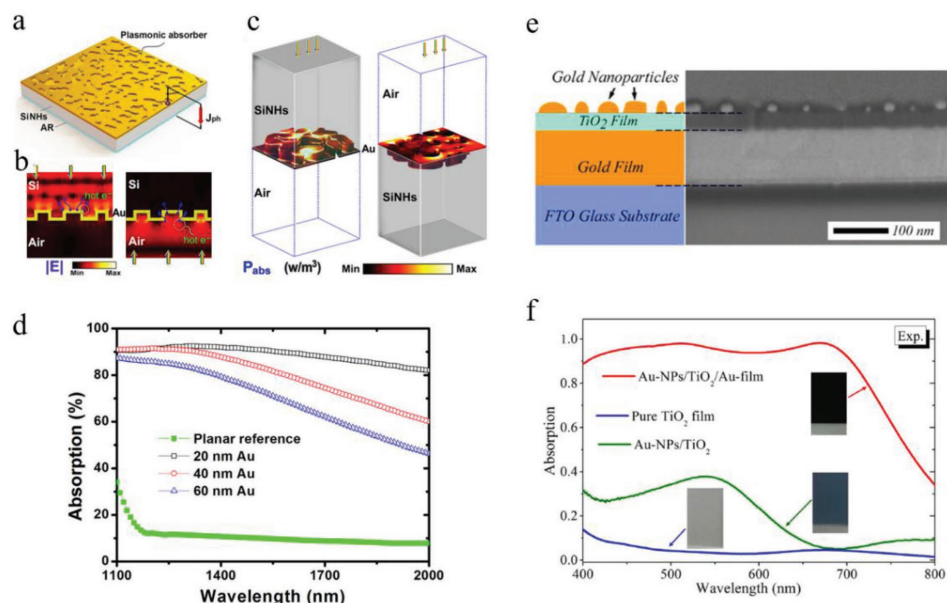
Figure 19. a) Schematic of the proposed plasmonic hot electron photodetector. b,c) Field and volumetric power absorption ( P_{\text{abs}} ) distributions of the device operating at the front and back-illumination modes, from simulations replicating a typical morphology of Au/SiNHs from the experiments. d) Measured absorption spectra under back illumination of the Au/SiNH devices with different thicknesses of Au coatings. The result of a planar reference device with 20 nm thick Au deposited on nonstructured sample is also included. e) Left: Schematic of the metal–dielectric–metal nanostructure that is composed of (from bottom to the top) a FTO glass substrate coated with an optically thick Au film ( \approx 150 nm) followed by a thin \text{TiO}_2 film acting as the spacer layer and at the very top, a monolayer of Au NPs with random size dispersion and spatial distribution. Right: Side-view SEM image of the optimized Au-NPs/ \text{TiO}_2 /Au-film nanostructure prepared with a 5-nm-thick Au film predeposited on a 50-nm-thick \text{TiO}_2 spacer layer. f) Experimentally measured absorption spectra of the Au-NPs/ \text{TiO}_2 /Au-film nanostructure, the pure \text{TiO}_2 film, and the Au-NPs/ \text{TiO}_2 nanostructure. The insets show the photographic images of the prepared samples. (a–d) Reproduced with permission. [168] Copyright 2017, American Chemical Society. (e,f) Reproduced with permission. [165] Copyright 2016, Springer Nature.
