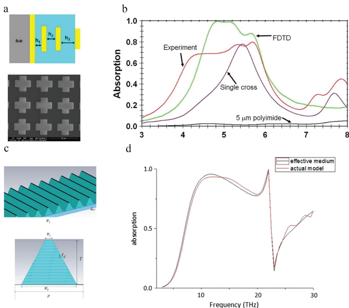
Figure 6. a) Cross-section illustration and SEM image of the complete multilayer absorber. b) Experimental and simulated data of the multilayer absorber. Also plotted is the experimental absorption spectrum for a single-layer absorber. c) Schematic diagram for a line array of graphene-dielectric multilayered quadrangular pyramidal frustums backed with a homogeneous metal film. A unit cell of the graphene BMMPA is illustrated, with P = 10 \mu\text{m} , w_b = 8 \mu\text{m} , w_t = 1 \mu\text{m} , t_d = 400 \text{ nm} , and T = 6 \mu\text{m} . Light with TM polarization is incident along z-direction. d) Absorption spectra for a graphene-dielectric multilayered pyramid absorber with N = 15 periods and thickness of dielectric layers equal to 400 nm. The red line is the result of the real structure, and the effective homogeneous mode is shown by the black line. (a,b) Reproduced with permission. [93] Copyright 2011, Optical Society of America. (c,d) Reproduced with permission. [78] Copyright 2013, IEEE.
