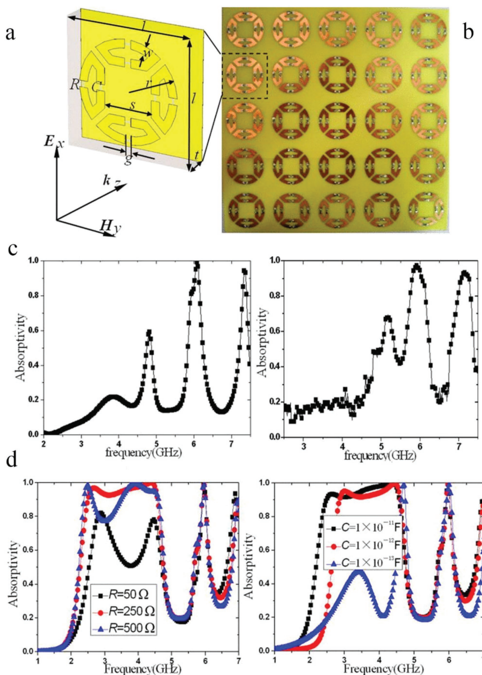
Figure 8. a) Perspective view of unit cell with indicated TEM wave direction and geometric dimensions and lumped parameters: l = 40 mm, r = 16 mm, s = 15.2 mm, w = 2.7 mm, g = 2 mm, t = 6 mm, C = 4 pF, R = 249 \Omega . b) Photograph of fabricated lumped elements BMMPA sample. c) Absorptivity of MPPA before introducing lumped elements: absorptivity of the simulation (left) and experimental results (right). d) Absorptivity of the BMMPA with different values for the lumped elements: lumped resistance R (left) and lumped capacitance C (right). Reproduced with permission. [45] Copyright 2012, AIP Publishing.
