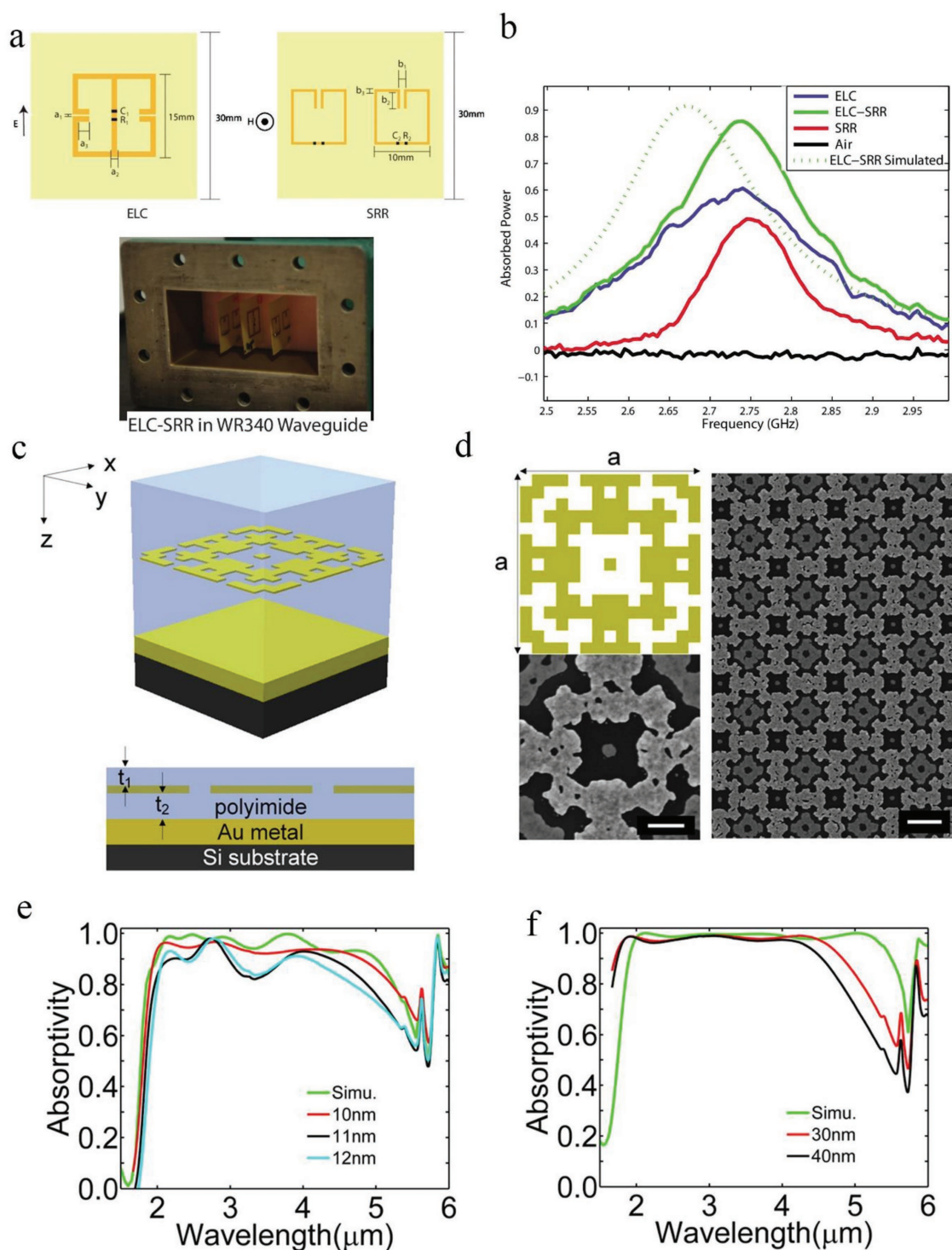
Figure 10. a) The optimum single-cell ELC-SRR absorption was achieved with ELC parameters of a_1 = 0.35 mm, a_2 = 1 mm, a_3 = 0 mm, C_1 = 10 pF, and R_1 = 10 \Omega , SRR parameters of b_1 = 0.7 mm, b_2 = 3 mm, b_3 = 0.5 mm, C_2 = 10 pF, and R_2 = 5 \Omega and ELC-SRR measured in a WR340 closed waveguide. b) ELC-SRR has the highest and broadest absorption with a 86% peak at 2.74 GHz, and FWHM bandwidth of 170 MHz. c) Diagram of optimized Au-based B MMPA structure. d) Top left: Top view of one unit cell of the design. Bottom left: FESEM image of a unit cell of the fabricated structure. Scale bar is 200 nm. Right: Low-magnification FESEM image of the same structure. Scale bar is 600 nm. e) Simulation and measurements for Au-based B MMPA under unpolarized illumination at normal incidence. The average Au thicknesses of the Au nanostructures as determined by atomic force microscopy measurements are 10, 11, and 12 nm. f) Simulation and measurements for Pd-based MMAs with Pd nanostructure thicknesses of 30 and 40 nm under unpolarized illumination at normal incidence. (a,b) Reproduced with permission. [42] Copyright 2010, AIP Publishing. (c–f) Reproduced with permission. [69] Copyright 2014, American Chemical Society.
