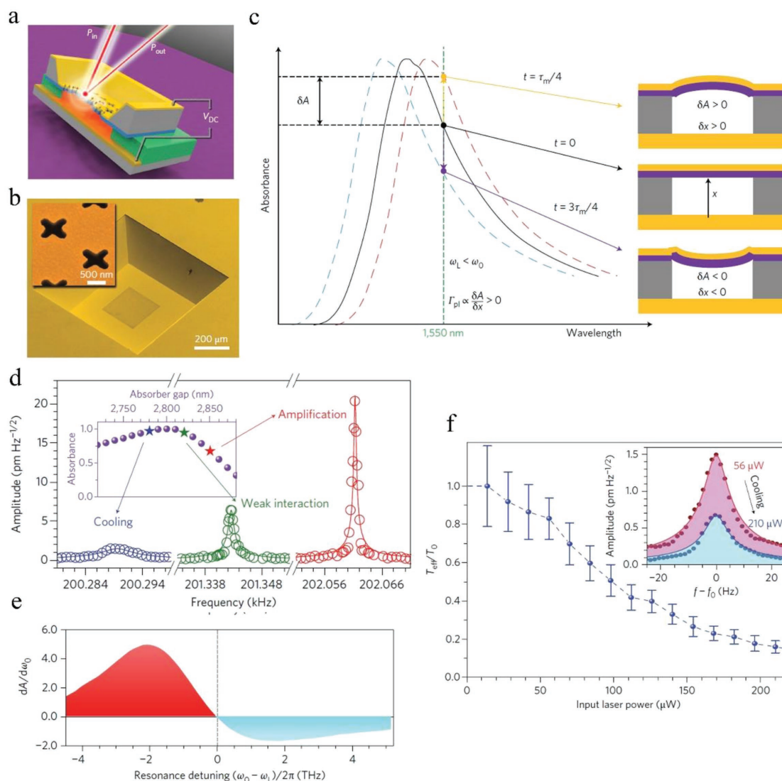
Figure 21. a) Schematic of a MPPA with a mechanically compliant bilayer (Au (25 nm)/SiN (100 nm)) membrane component decorated with a nano-antenna array. b) The false-color SEM image of the fabricated cross-shaped nanoslot (length (360 nm)/width (150 nm)) antenna array (period 800 nm) that covers an area of 250\ \mu\text{m} \times 250\ \mu\text{m} at the center of the 500\ \mu\text{m} \times 500\ \mu\text{m} membrane. Inset: close-up SEM of the array. c) Plasmomechanical coupling: when the MM is illuminated with a pump laser at \omega_L corresponding to a wavelength of 1550 nm, tuned slightly to the red side of the Fano resonance frequency \omega_0 , the natural oscillation of the membrane of amplitude \delta x at its mechanical resonance frequency ( 1/\tau_m ) leads to a dynamic modulation of total absorbance ( \delta A ). As \delta A varies between positive and negative values, this leads to a dynamic modulation on the thermal expansion of the membrane. As illustrated here for positive resonance detuning, that is, \omega_L < \omega_0 , the light-induced mechanical damping \Gamma_{pl} \propto \delta A/\delta x is always positive, which dampens the mechanical resonance. d) The thermomechanical Brownian noise spectra for the fundamental mechanical resonance measured at a pump power of \approx 17\ \mu\text{W} for different absorber gap values corresponding to weak (unperturbed), positive (amplification), and negative (cooling) absorption-induced forces. The inset shows the MM absorbance as a function of absorber gap at 1550 nm pump wavelength near the Fano resonance. e) Differential spectral absorbance ( dA/d\omega_0 ) versus the detuning between the Fano resonance frequency ( \omega_0 ) and the fixed 1550 nm pump laser frequency ( \omega_L ). f) The effective temperature T_{eff} of the fundamental mechanical mode is proportional to the area under its peak thermomechanical noise spectrum, exemplified in the inset. The absorber gap has been tuned at 5.5 V, corresponding to the maximum |dA/d\omega_0| on the red side of the Fano resonance. At 210\ \mu\text{W} pump power, T_{eff} for the Brownian motion of the mechanical mode is reduced below 50 K from room temperature ( T_0 = 300\ \text{K} ). (a–f) Reproduced with permission. [18] Copyright 2016, Springer Nature.
