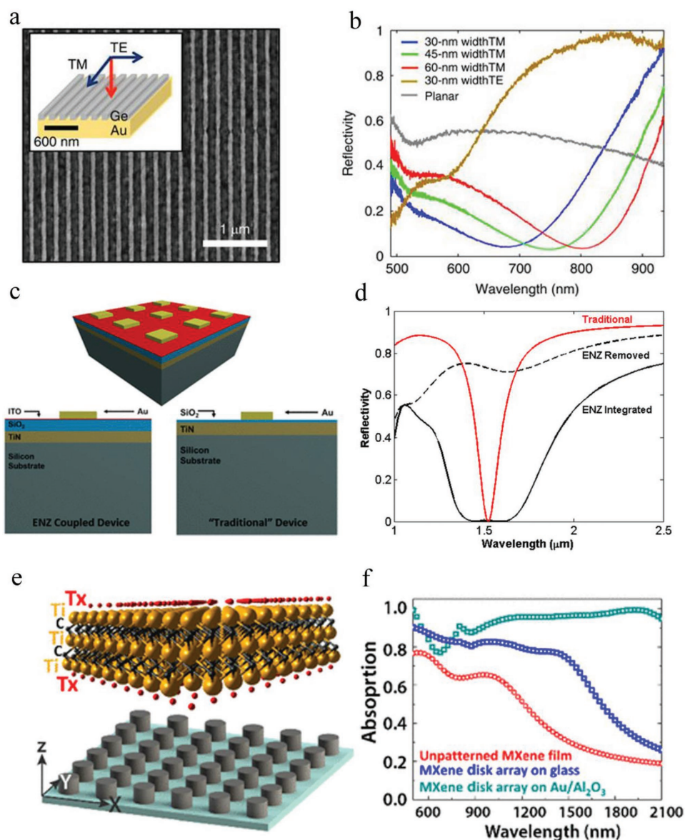
Figure 13. a) Top-view SEM image of a fabricated metafilm with Ge beams, with a 200 nm period and 0.3 duty cycle. Scale bar: 1 μm. b) Measured reflectivity spectra for TM polarized light for metafilms constructed from nanobeams with a width of 30 (blue), 45 (green), and 60 nm (red). The reflectivity spectra for TE polarized light of the array with 30-nm-wide beams (brown) and a planar Ge film (grey) are shown for reference. c) Schematic (top) and cross section of the device consisting of a TiN metallic thick film, a SiO 2 dielectric layer, an ITO nanofilm, and a patterned periodic array of metal squares, all on top of a Si substrate, and a schematic of a reference “traditional” perfect light absorber without an ENZ layer. d) Simulated reflectivity curves for a perfect absorber with integrated ENZ (solid black line), absorber without ENZ layer (dashed black line), and an optimized “traditional” gap-plasmon perfect light absorber without ENZ layer (solid red line). e) Schematic of the BMMPA fabricated using 2D titanium carbide (Ti 3 C 2 T x ) MXene. f) Comparison of experimental absorption spectra of the two types of disk arrays and unpatterned MXene film (incident light is TE polarized; angle of incidence is 20°). (a,b) Reproduced with permission. [137] Copyright 2015, Springer Nature. (c,d) Reproduced with permission. [128] Copyright 2018, American Chemical Society. (e,f) Reproduced with permission. [81] Copyright 2018, American Chemical Society.
