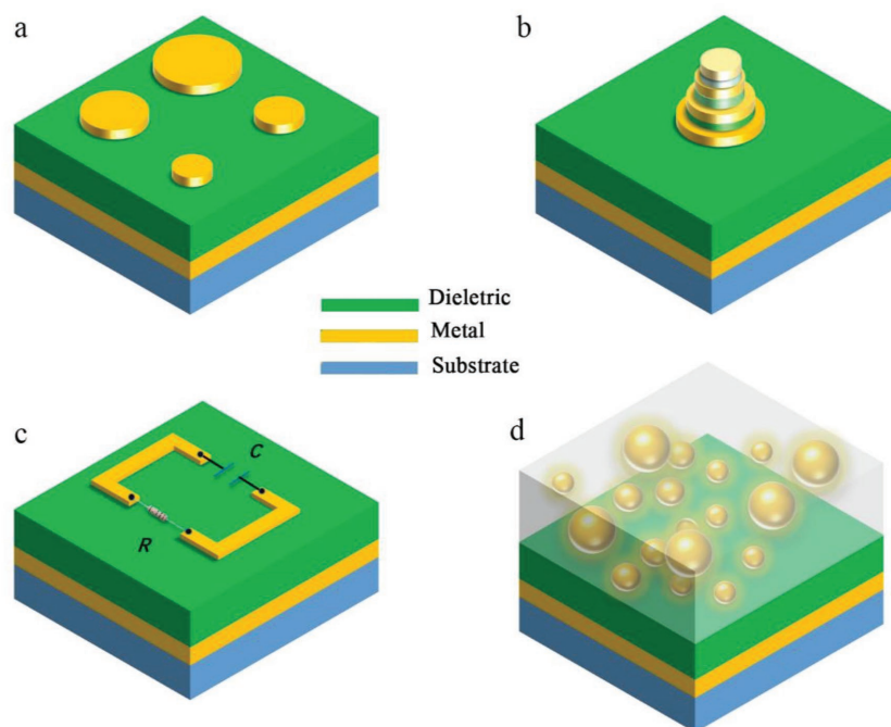
Figure 2. Conventional designs for BMMPAs. a) Planar arrangement, b) vertical arrangement, c) welded with lumped elements, and d) nanocomposites.
