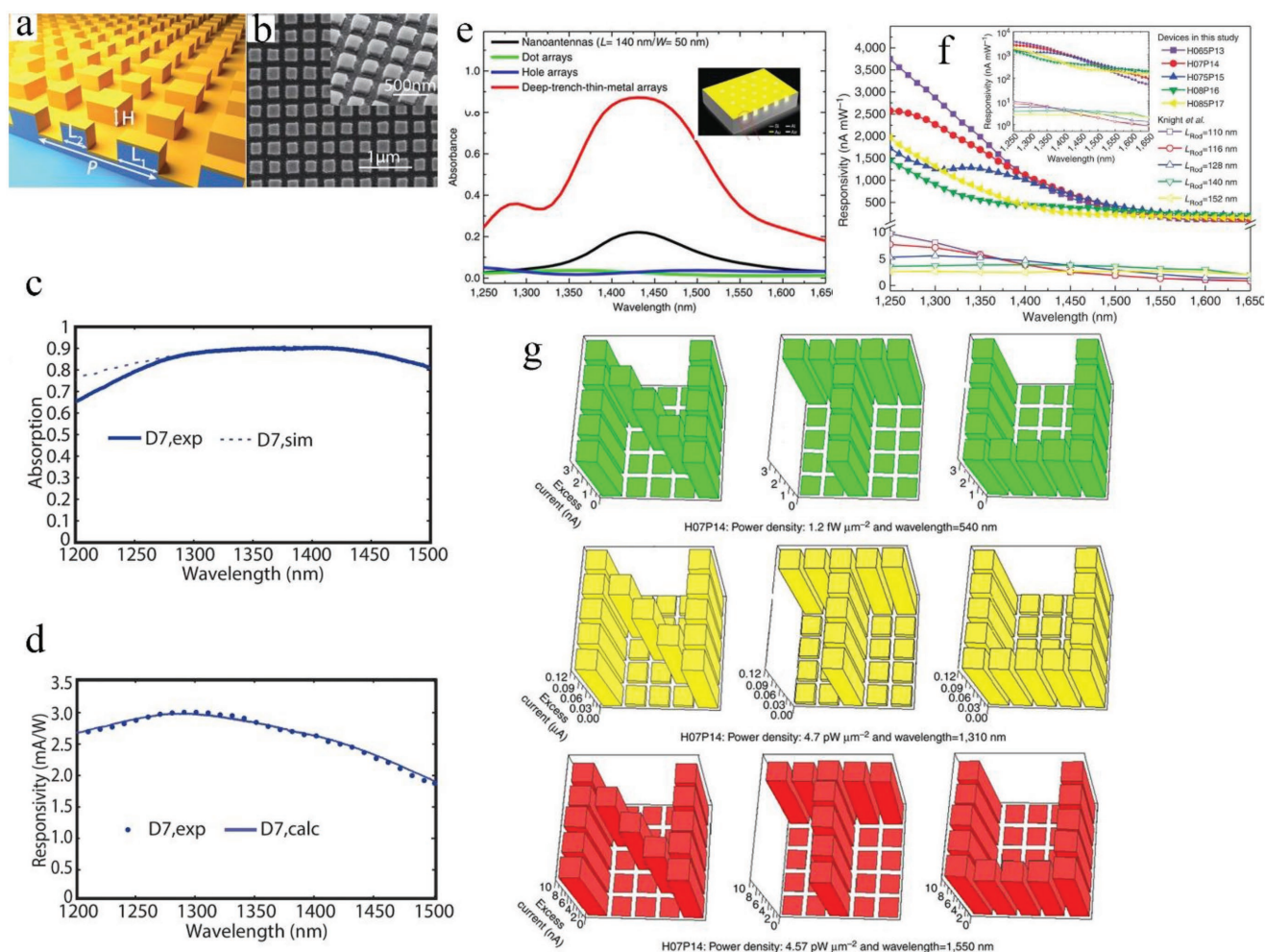
Figure 17. a) Schematic of the BMMPA photodetector. The dimensions of the photodetector are L_1 = 185 nm, L_2 = 225 nm, P = 680 nm, H = 160 nm. b) SEM image of the fabricated device. c) Experimentally measured (solid) and simulated (dashed) absorption spectra of the BMMPA detector. d) Experimentally measured (circles) and calculated (line) photoresponsivity spectra of the BMMPA photodetector. e) Simulated absorption spectra of the four types of antenna structures. Among them, the DTTM arrays exhibited the largest absorption in the broadband regime. The inset is the illustration of the detector structure. f) Responsivity spectra of the proposed DTTM devices, in comparison with the nanoantenna-based devices reported by Knight et al. [156] g) Bar charts displaying excess current obtained by the H07P14-containing DTTM device under an applied bias voltage of 0 V, detected at wavelengths of 540, 1310, and 1550 nm. The images were constructed based on the existence or absence of a photocurrent during the point-by-point scanning of the DTTM device. Clear images of the capitalized letters “NTU” were obtained, even though the incident power density was low; in particular, 4.7 \text{ pW } \mu\text{m}^{-2} at a wavelength of 1310 nm and 4.57 \text{ pW } \mu\text{m}^{-2} at a wavelength of 1550 nm. The pixel size is 5 nm. (a–d) Reproduced with permission. [154] Copyright 2014, American Chemical Society. (e–g) Reproduced with permission. [30] Copyright 2014, Springer Nature.
