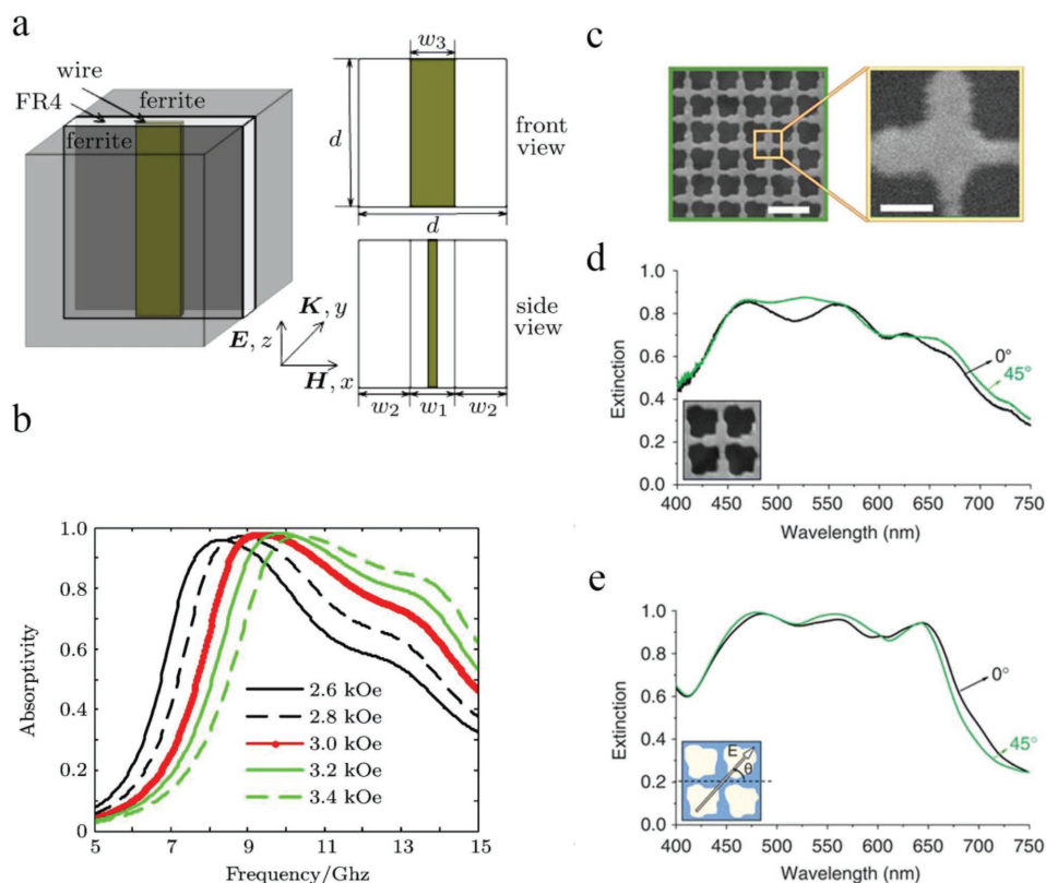
Figure 12. a) Schematic diagram of the ferrite-wire BMMPA unit cell. Front view, side view, and structure parameters are presented. b) The absorption bands under different magnetic biases. c) SEM image of the fabricated crossed trapezoidal arrays (left) and a single unit cell (right). Scale bars are 500 and 100 nm, respectively. d) Measured and e) simulated extinction spectra using digitized SEM images (inset) for different incident electric field polarization angles (inset). (a,b) Reproduced with permission. [125] Copyright 2012, IOP Publishing. (c–e) Reproduced with permission. [124] Copyright 2011, Springer Nature.
