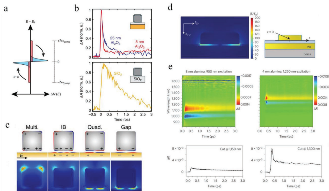
Figure 18. a) Hot electron distribution from plasmon excitation. Nonthermal (red) carriers initially form a symmetric stepwise distribution relative to the Fermi energy upon excitation. After electron–electron scattering, a thermalized electron population (cyan) with a Fermi–Dirac distribution is formed from the nonthermal electrons, with an electronic temperature above that of the lattice. b) Kinetic trace of normalized differential absorbance for Ag nanocubes on an 8 nm \text{Al}_2\text{O}_3 spacer compared to a 25 nm \text{Al}_2\text{O}_3 spacer at the gap resonance (top) and to bare Ag nanocubes on \text{SiO}_2 in transmission mode (bottom), which exhibit no ultrafast ( \approx 100 fs) decay of the response, arising from the relaxation of highly energetic nonthermal carriers. c) Cross section of the surface charge (top) and electric field profiles (bottom) at the peaks of the interband (IB) transition and plasmon modes for an electric field oriented in-plane. The field strength scale is up to 20 \times that of free space for the multipolar (Multi) mode, IB transition, and quadrupolar (Quad) mode and 100 \times that of free space for the gap mode. d) Left: Electromagnetic field distribution inside the nanostructure (defined as |E/E_0| ), showing strong plasmonic hot spots at the edges of the nanodisk; right: geometry of the system. e) 2D map of the time evolution of the plasmonic spectral change in 8-nm-thick (left) and 4-nm-thick (right) alumina spacer samples, and (bottom) cuts at 1115 nm (left) and 1300 nm (right) showing the time dynamics of the corresponding data in the above panels after excitation of the plasmon. The time dynamics in the 4-nm-thick spacer are drastically different to the thicker spacer, with a new ultrafast component following the excitation near its resonance at 950 nm. (a–c) Reproduced with permission. [158] Copyright 2017, Springer Nature. (d,e) Reproduced with permission. [157] Copyright 2015, Springer Nature.
