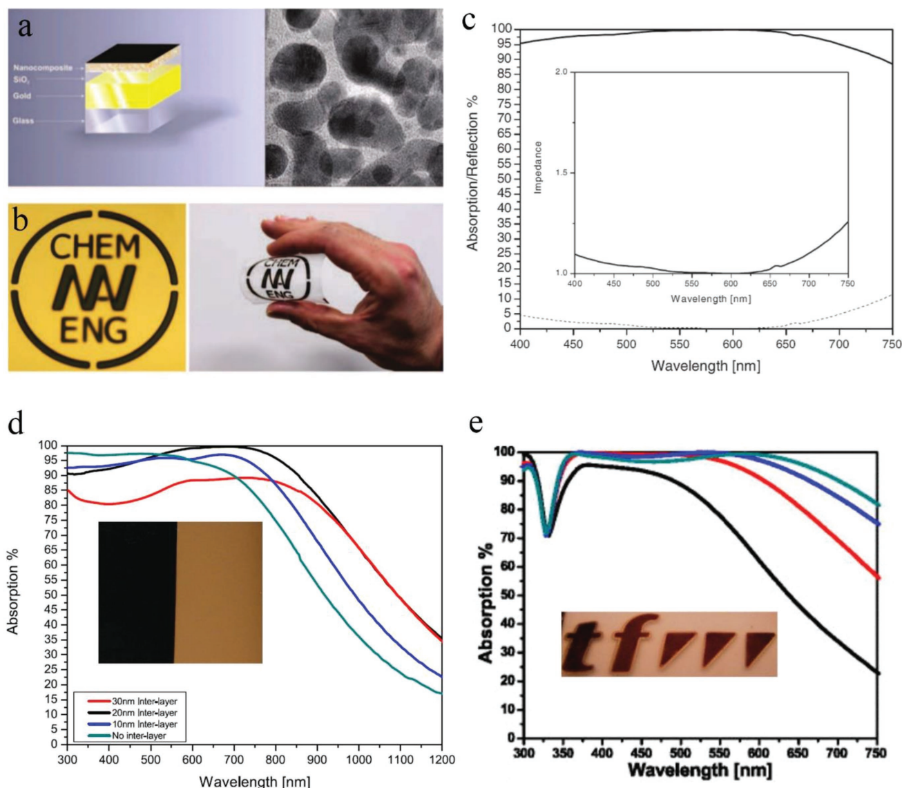
Figure 9. a) Schematic of a perfect absorber structure manufactured by sputtering. The thickness of the nanocomposite, SiO 2 spacer, and gold mirror layers are 20, 25, and 100 nm, respectively. The left panel illustrates that the whole structure sits on top of a glass substrate; the right panel shows a top-view TEM image of the nanocomposite film. b) Perfect absorber (blackbody) coated via mask on gold-coated glass (left) and flexible polymer foil (right). These examples show the potential of the coating for application on different substrates, including flexible ones. c) Absorption (solid line) and reflection (dashed line) spectra of the system described in panel (a), measured at 6° angle of incidence. The inset shows the impedance data of a 20 nm Au/SiO 2 nanocomposite deposited on a 100 nm gold film with 25 nm SiO 2 spacer layer. d) Absorption spectra of 20 nm Cu-PTFE composite on a PTFE spacer layer with different thicknesses, over 100 nm of Cu. The green curve shows the composite on a base layer without any interlayer for comparison. The inset is the photo of the perfect black absorber (left) in comparison with bare copper film (right). e) Absorption spectra of a silver-SiO 2 nanocomposite of 15 nm (black curve), 20 nm (red curve), 25 nm (blue curve), and 30 nm (green curve) thickness, deposited on 15 nm of SiO 2 coating a silver mirror. The inset is true color photograph of the perfect absorber coated on transparent polymeric substrate presenting the logo of Faculty of Engineering (TF) of University of Kiel. (a–c) Reproduced with permission. [11] Copyright 2011, Wiley-VCH. (d) Reproduced with permission. [80] Copyright 2012, Springer Nature. (e) Reproduced with permission. [116] Copyright 2014, AIP Publishing.
