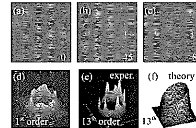
Fig. 5. (a-c) Modification of the diffraction pattern as a function of the horizontal shift. Numbers indicate the shift in \mu\text{m} . The sample is with horizontal X axis. (d,e) Experimental intensity distribution of m=1 and m=13 SH rings. (f) Theoretical prediction for the azimuthal intensity distribution of the m=13 SH ring based on Eq.(3).
