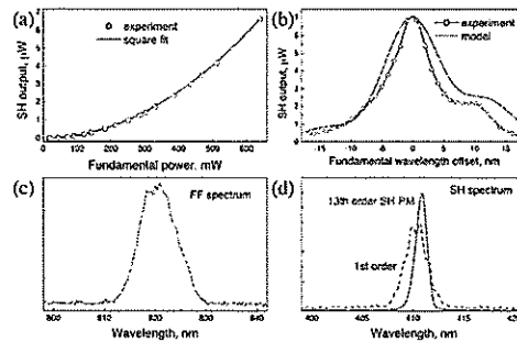
Fig. 4. (a) Quadratic dependence of the 13-th order SH ring. (b) Experimental phase matching curve and theoretical prediction normalized to the maximal point of the experiment. (c) Spectrum of the fundamental radiation. (d) Spectra of the SH rings for non phase matched (first-order) and phase matched (13-th order) SH rings.
