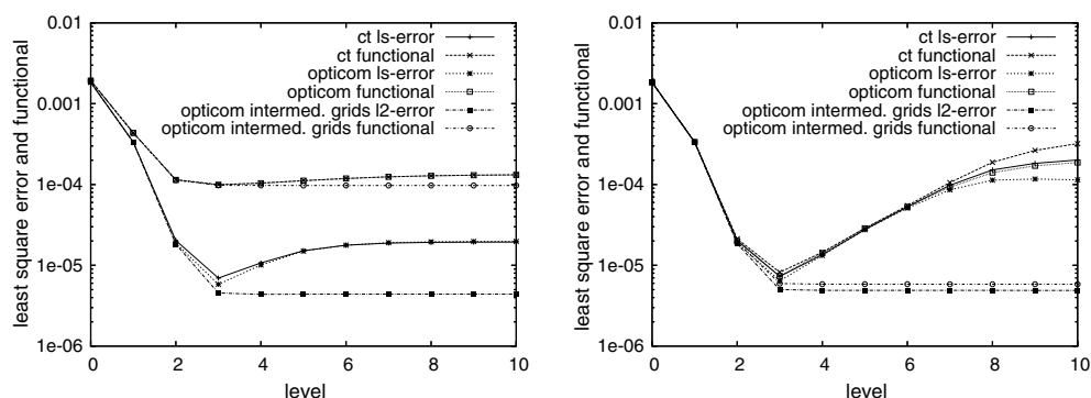
Fig. 2. Value of the functional (10) and the least squares error on the data, i.e. \frac{1}{M} \sum_{i=1}^M (f(x_i) - y_i)^2 , for the reconstruction of e^{-x^2} + e^{-y^2} for the combination technique and the optimised combination technique for the grids \Omega_{i,0} , \Omega_{0,i} , \Omega_{0,0} and the optimised combination technique for the grids \Omega_{j,0} , \Omega_{0,j} , 0 \leq j \leq i with \lambda = 10^{-4} (left) and 10^{-6} (right).
