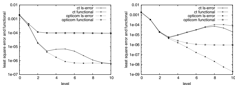
Fig. 3. Value of the functional (10) and the least squares error on the data, i.e. \frac{1}{M} \sum_{i=1}^M (f(x_i) - y_i)^2 , for the reconstruction of e^{-x^2} + e^{-y^2} for the combination technique and the optimised combination technique with \lambda = 10^{-4} (left) and 10^{-6} (right) and level n = 0, \dots, 10 .
