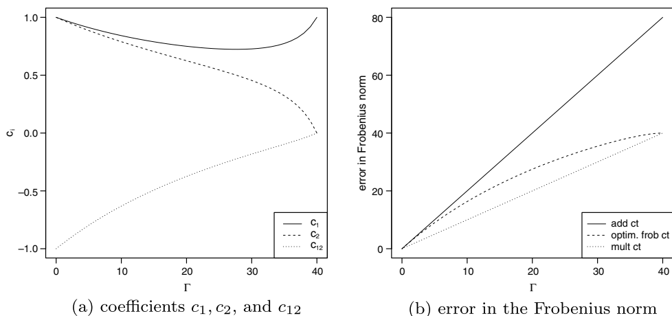
Fig. 1. Examples for the dependence of the coefficients c_1 , c_2 , and c_{12} and the errors on \Gamma for n_1 = 50 and n_2 = 40 : (a) coefficients c_1 , c_2 , and c_{12} , (b) error in the Frobenius norm.
