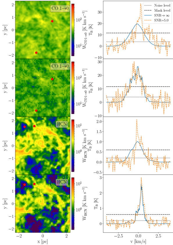
Figure 9. Velocity-integrated intensity maps (left) and two typical spectra (right) for two tracers CO 1 \rightarrow 0 and HCN, for the same snapshot as Fig. 1. In the left column, the top panel for each of the two tracers shows the results for the true PPV cube, while the bottom panel shows the results after beam convolution and with a finite SNR of 5. The red circles in the map denote the positions at which we extract the two example spectra shown in the right column. In this column, we show both the true and noise-added spectra; we also show the 1 \sigma noise level and the mask we apply at 3 \sigma as dotted and dashed lines, respectively.
